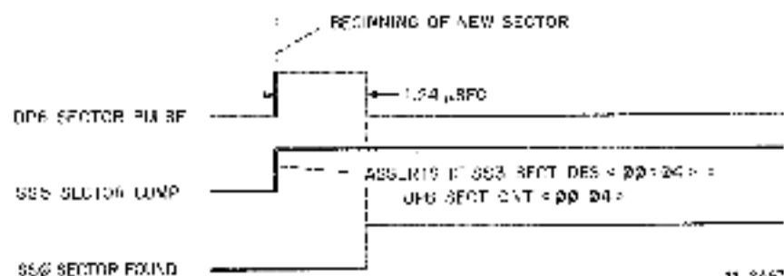
Figure 3-4 Sector Search Timing Diagram
