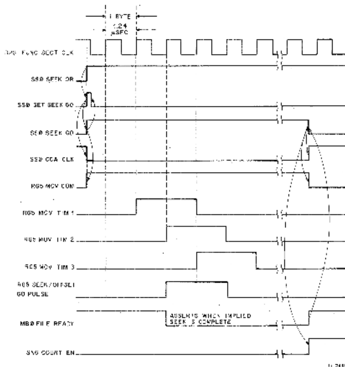
Figure 3-2 Implied Seek Timing Diagram
