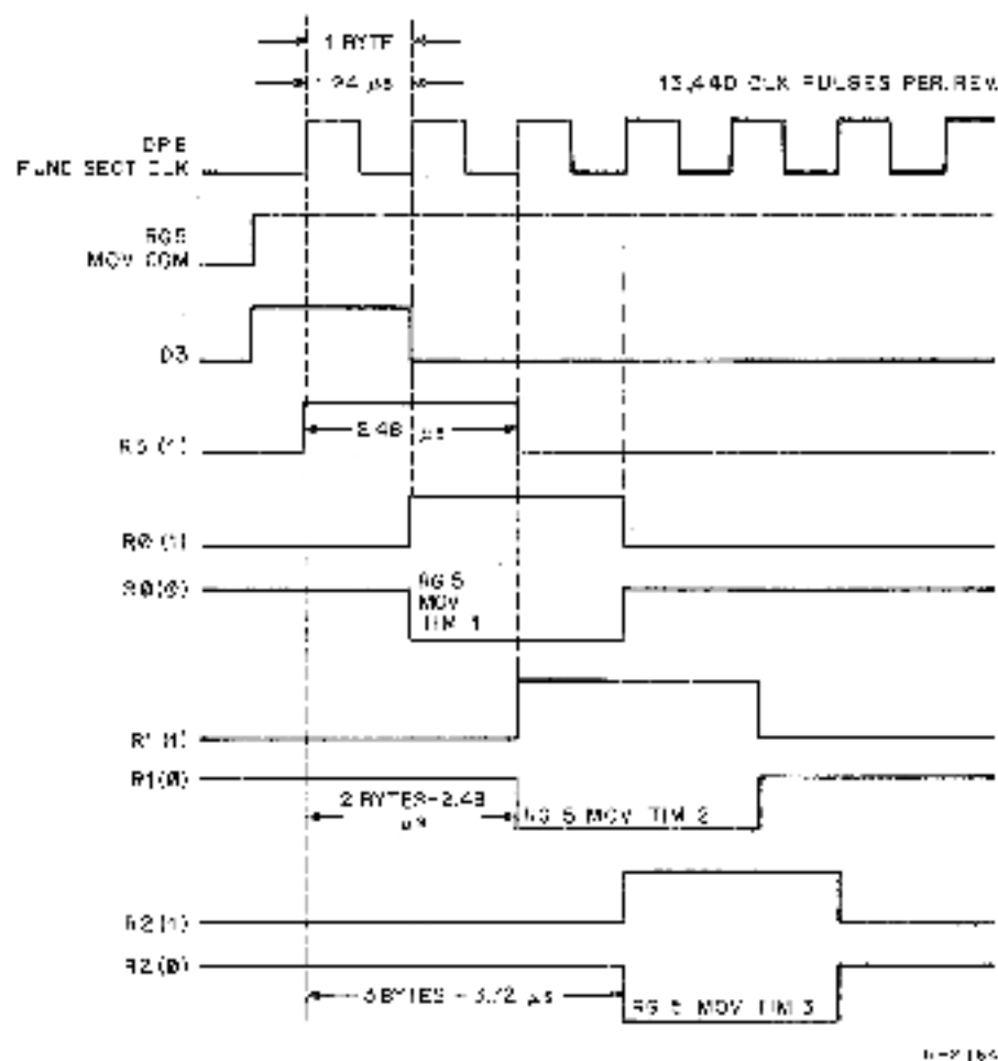
Figure 3-1 Move Timing Diagram
