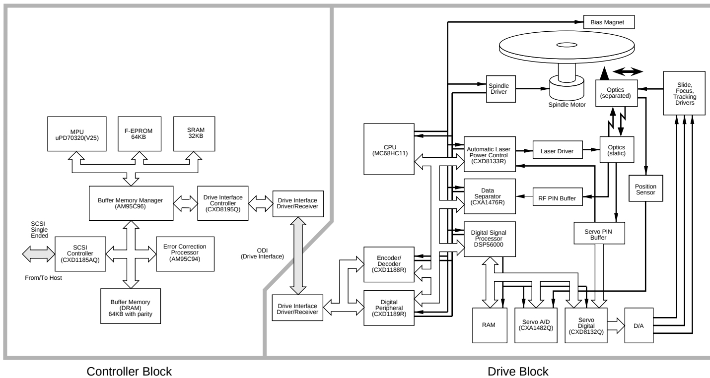
RWZ21 Block Diagram
