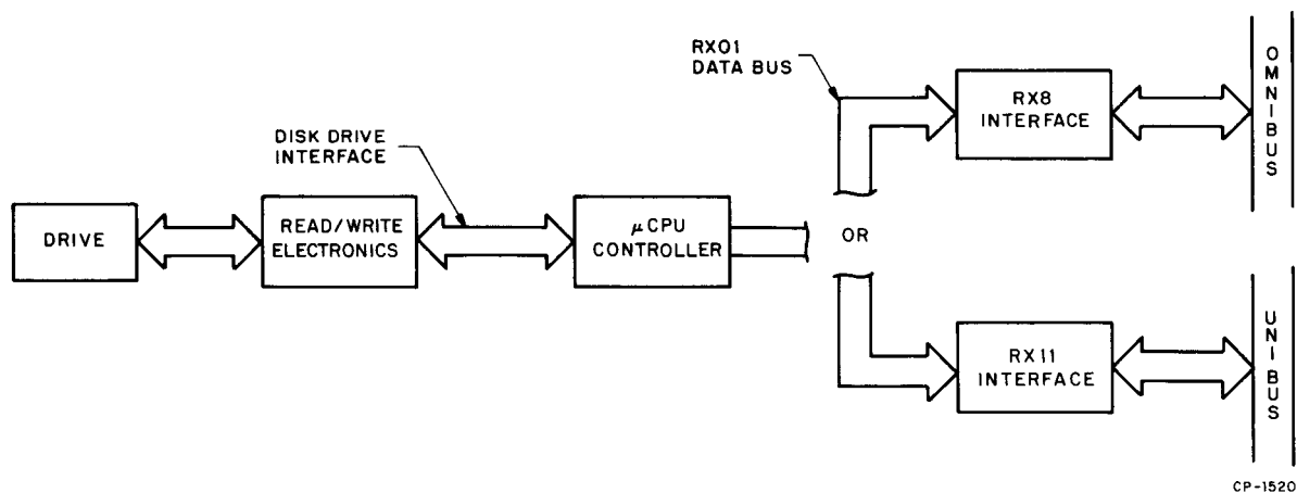
Figure 5-1 Bus Structure
