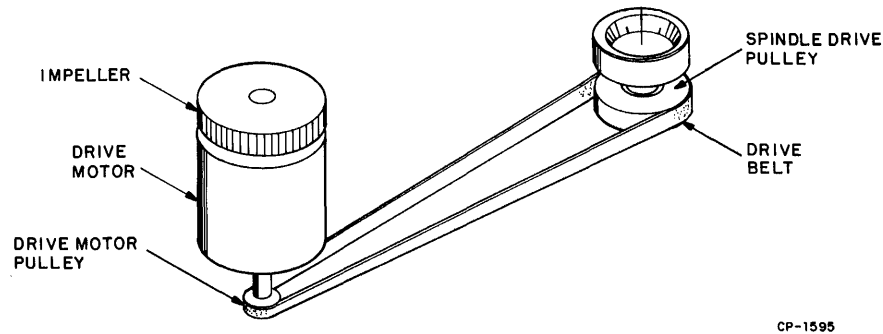
Figure 5-24 Drive Mechanism
