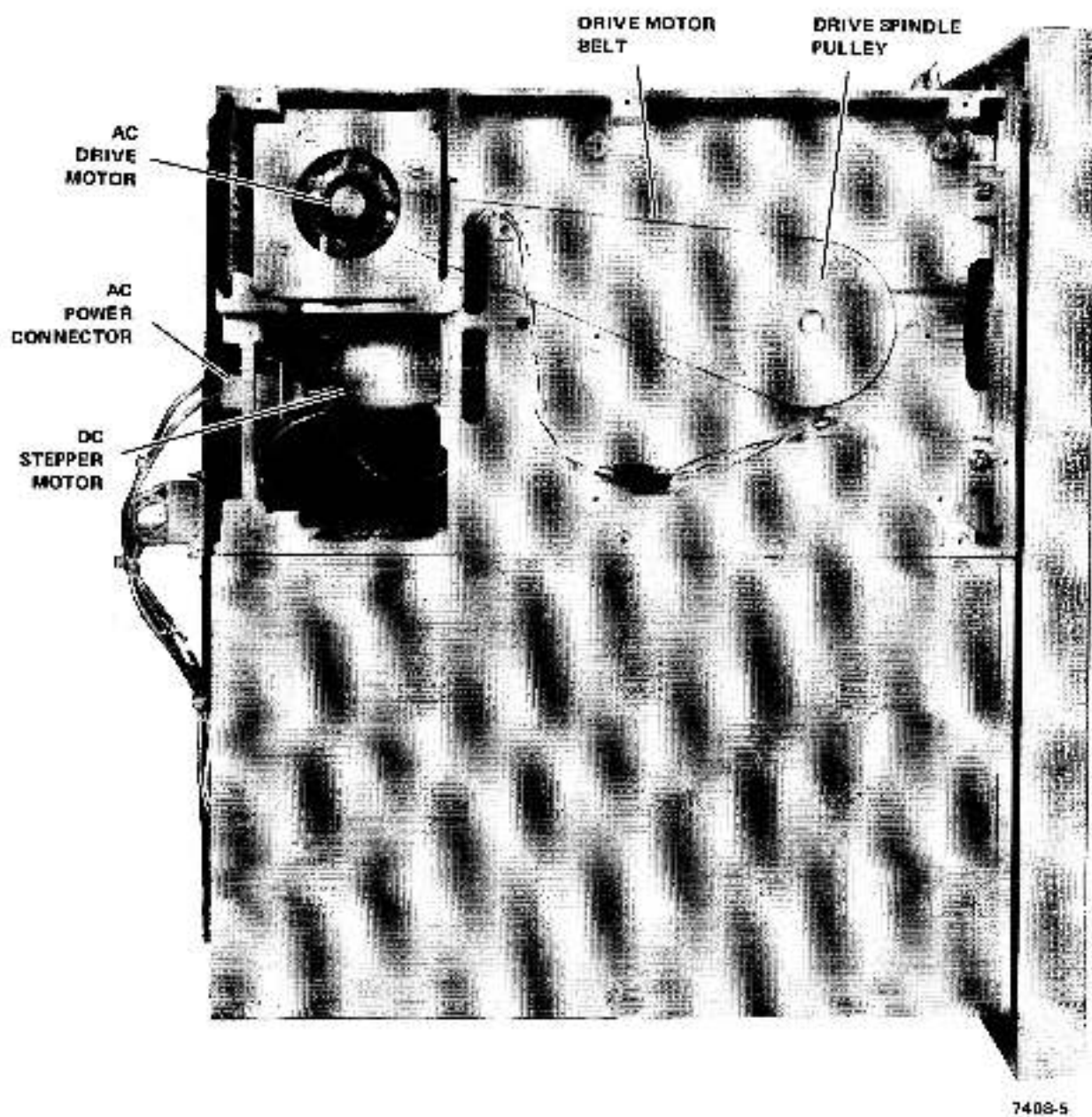
Figure 1-6 Underside View of Drive
