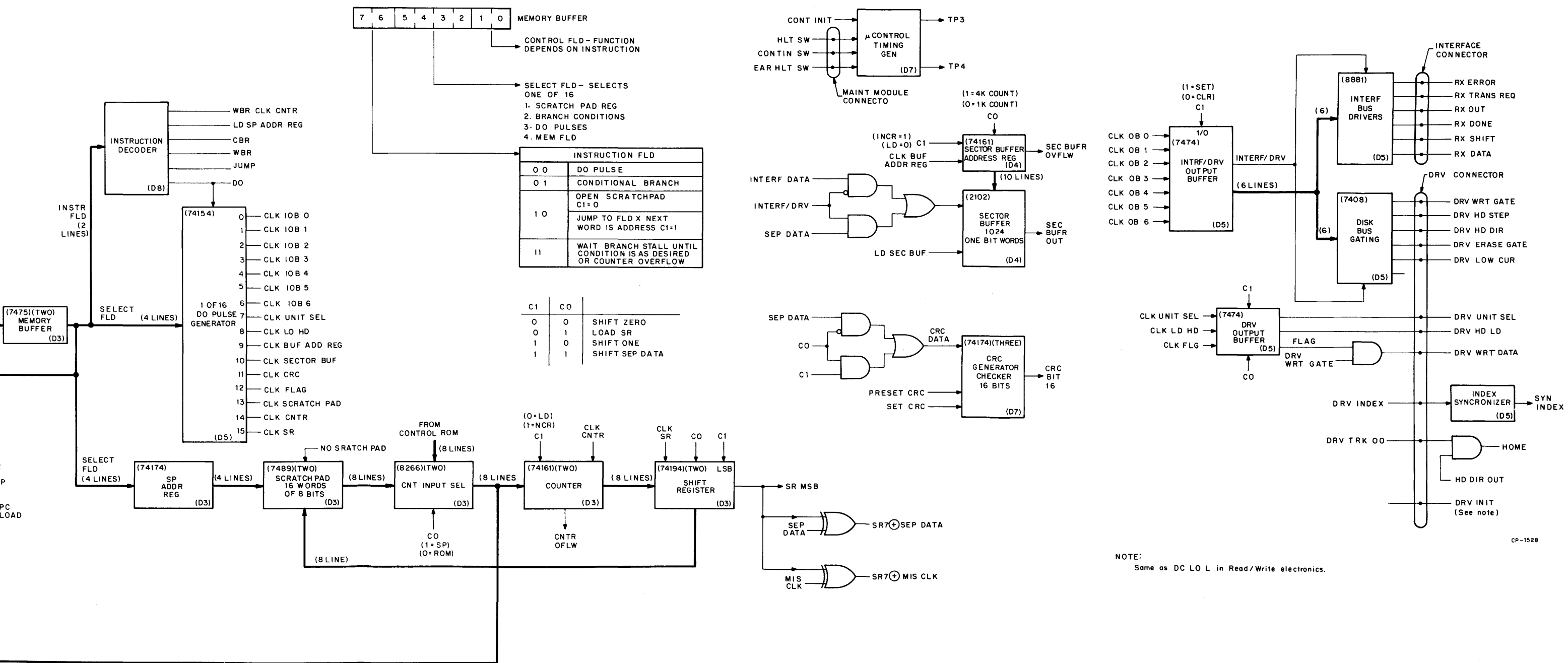
Figure 5-9 μCPU Controller Block Diagram
