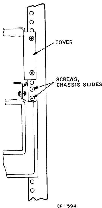
Figure 2-5 RX01 Cabinet Mounting Information
