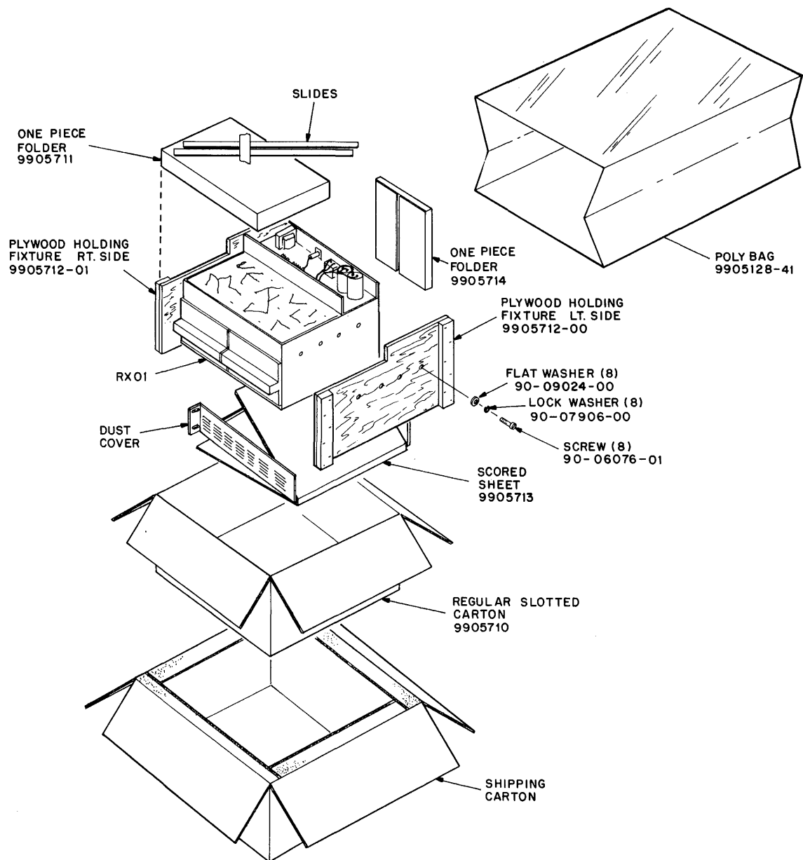
Figure 2-4 RX8/RX11 Unpacking
