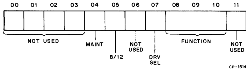
Figure 4-2 Command Register Format (RX8E)
