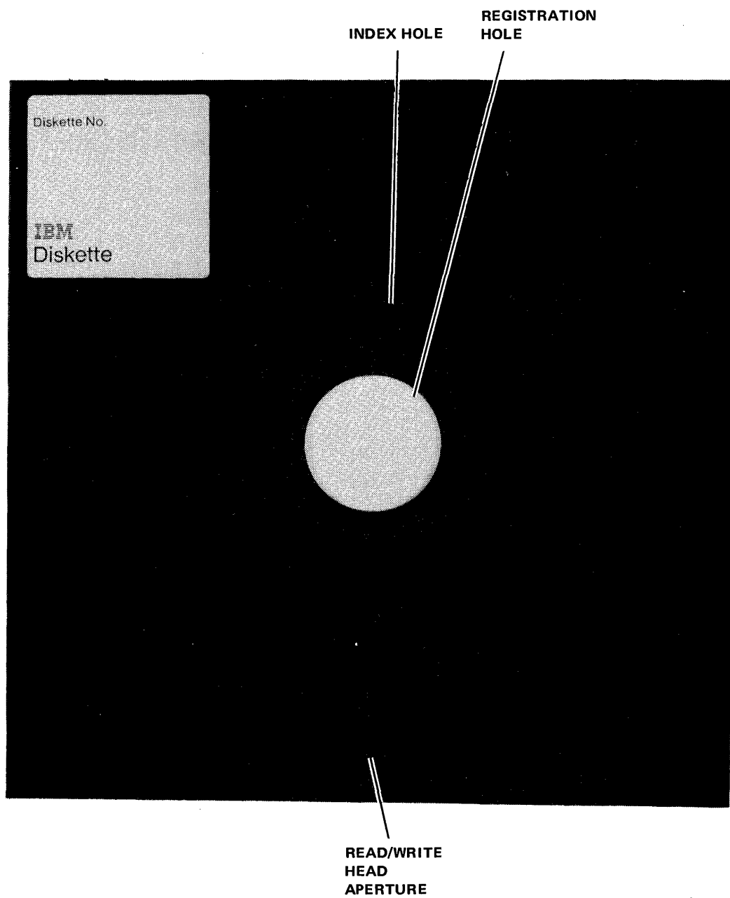
Figure 1-8 Diskette Media
