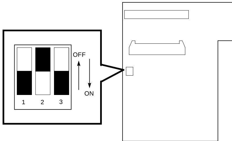
Figure 1–2 RX26 FDI Module SCSI ID Switch Locations
