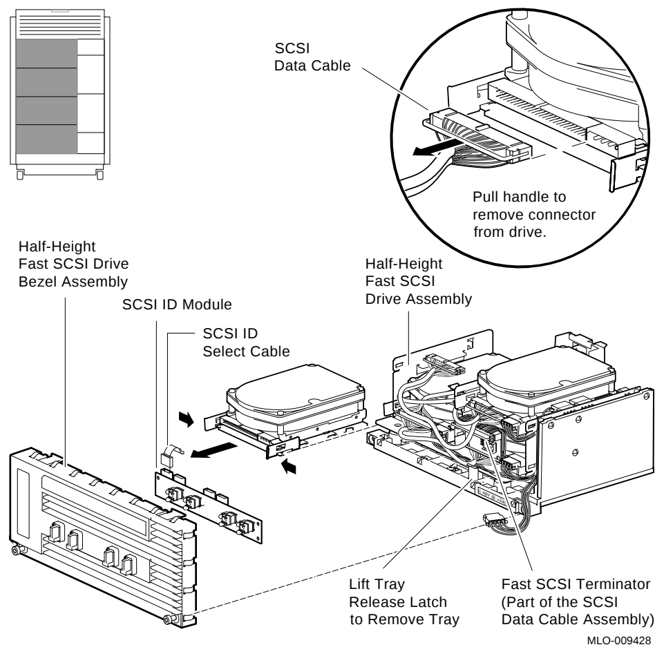
Figure 3 RZ-Series 3 1/2-Inch Fast SCSI Storage Assembly
