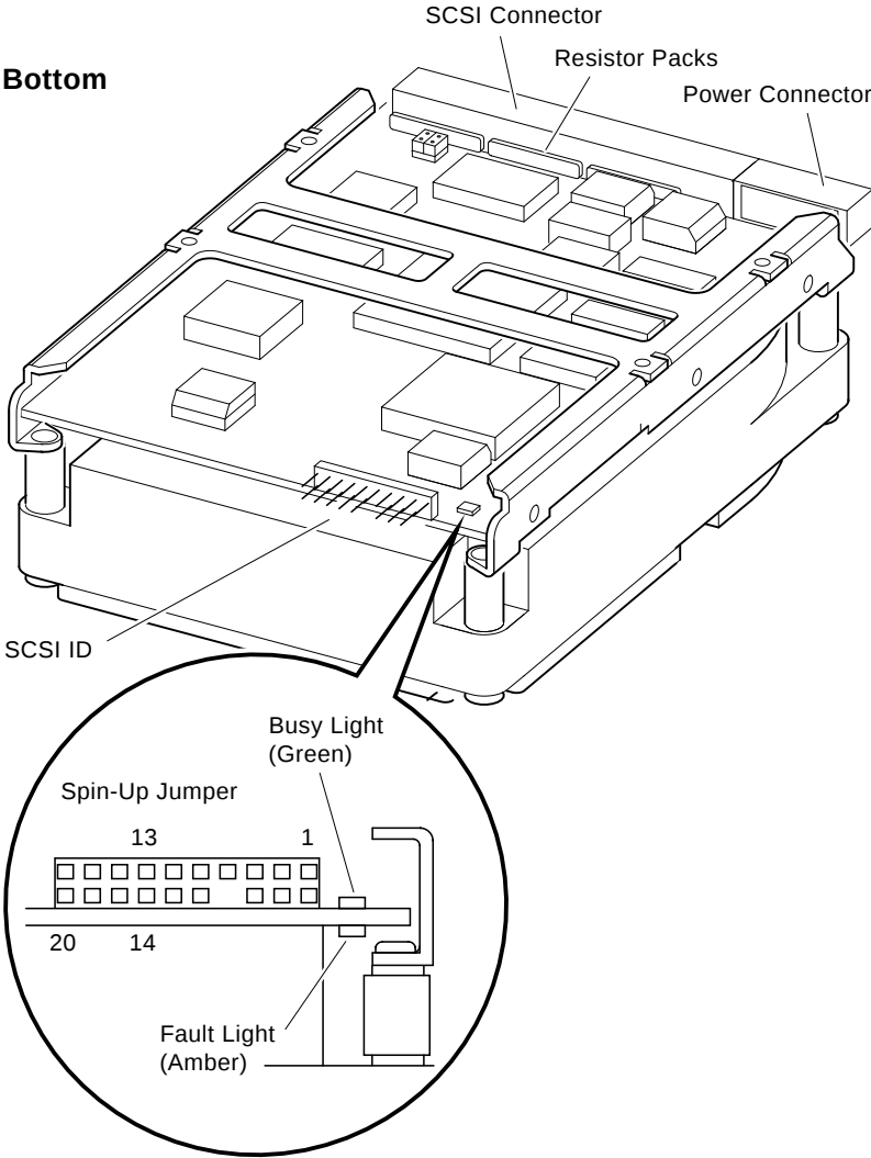
Figure 5 RZ-Series 3 1/2-Inch Light Location
