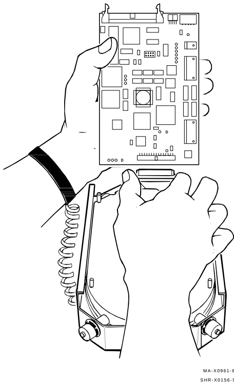
Figure 4-7 Disconnecting the RZ73 Flex Circuit
