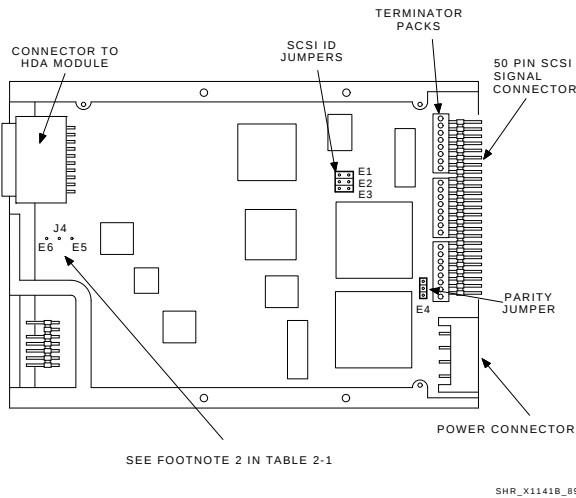
Figure 2–1 RZ22 and RZ23 Drive Module Layout
