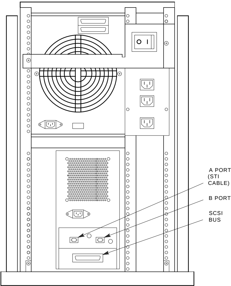
Figure 2-1 SA100 Rear View
