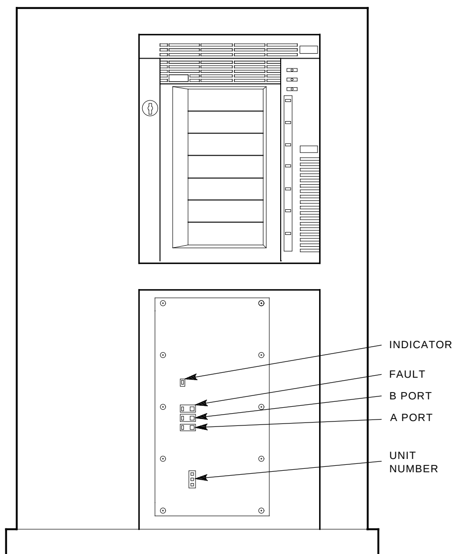
Figure 4-1 SA106 and TA867 Controls and Indicators
