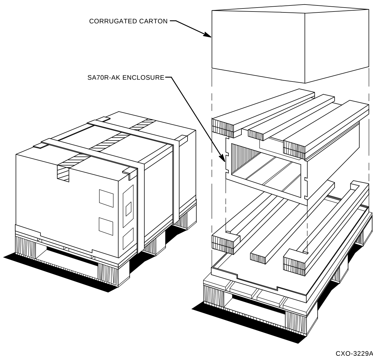
Figure 5-6 Contents of the SA70R-AK Enclosure Shipping Container
