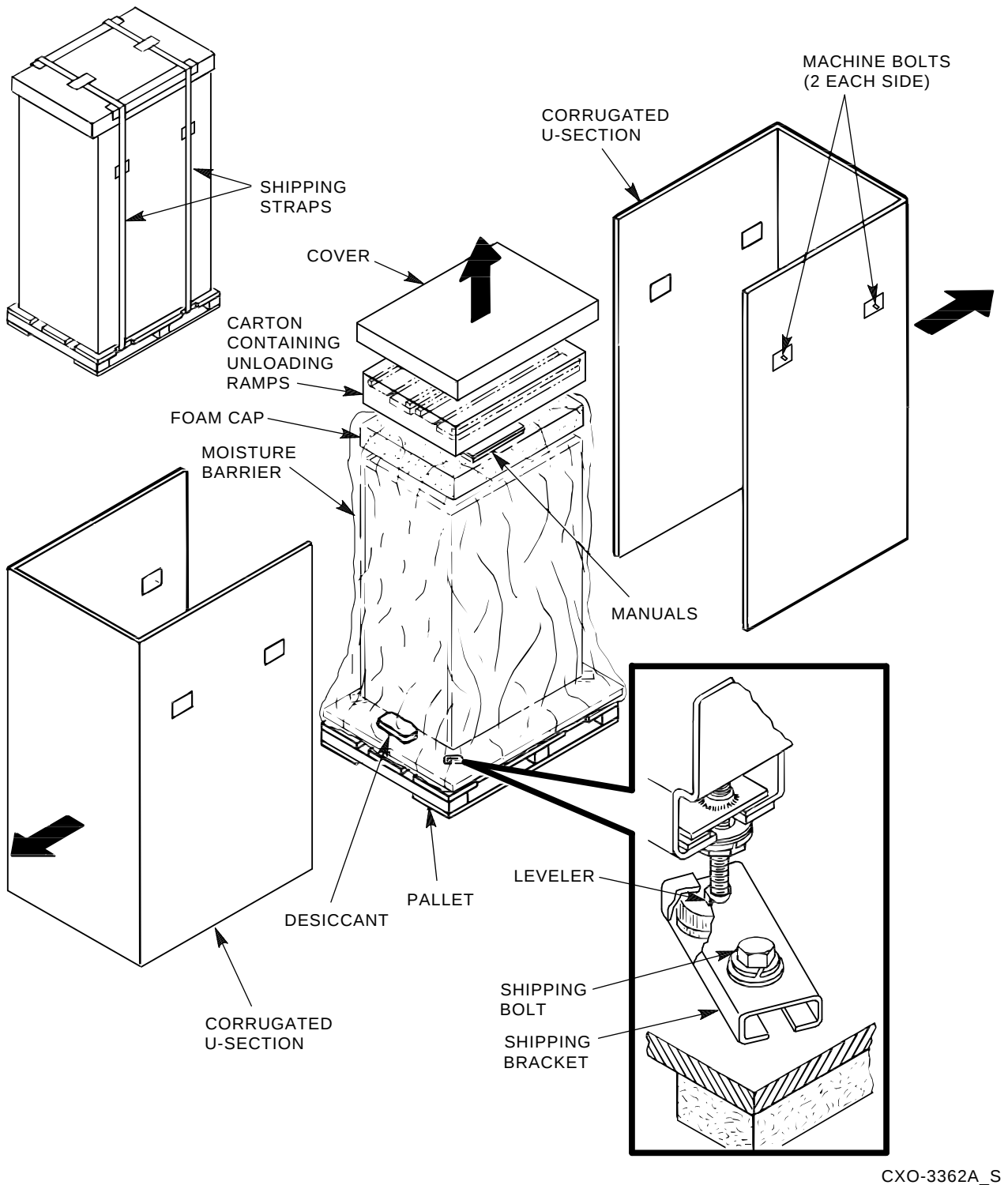
Figure 2-1 Contents of the SA705 Storage Array Shipping Container
