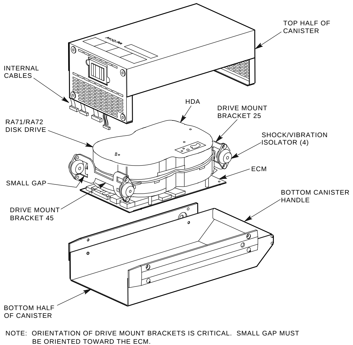
Figure 1-5 Exploded View of the RA71-RK/RA72-RK Removable Disk Drive
