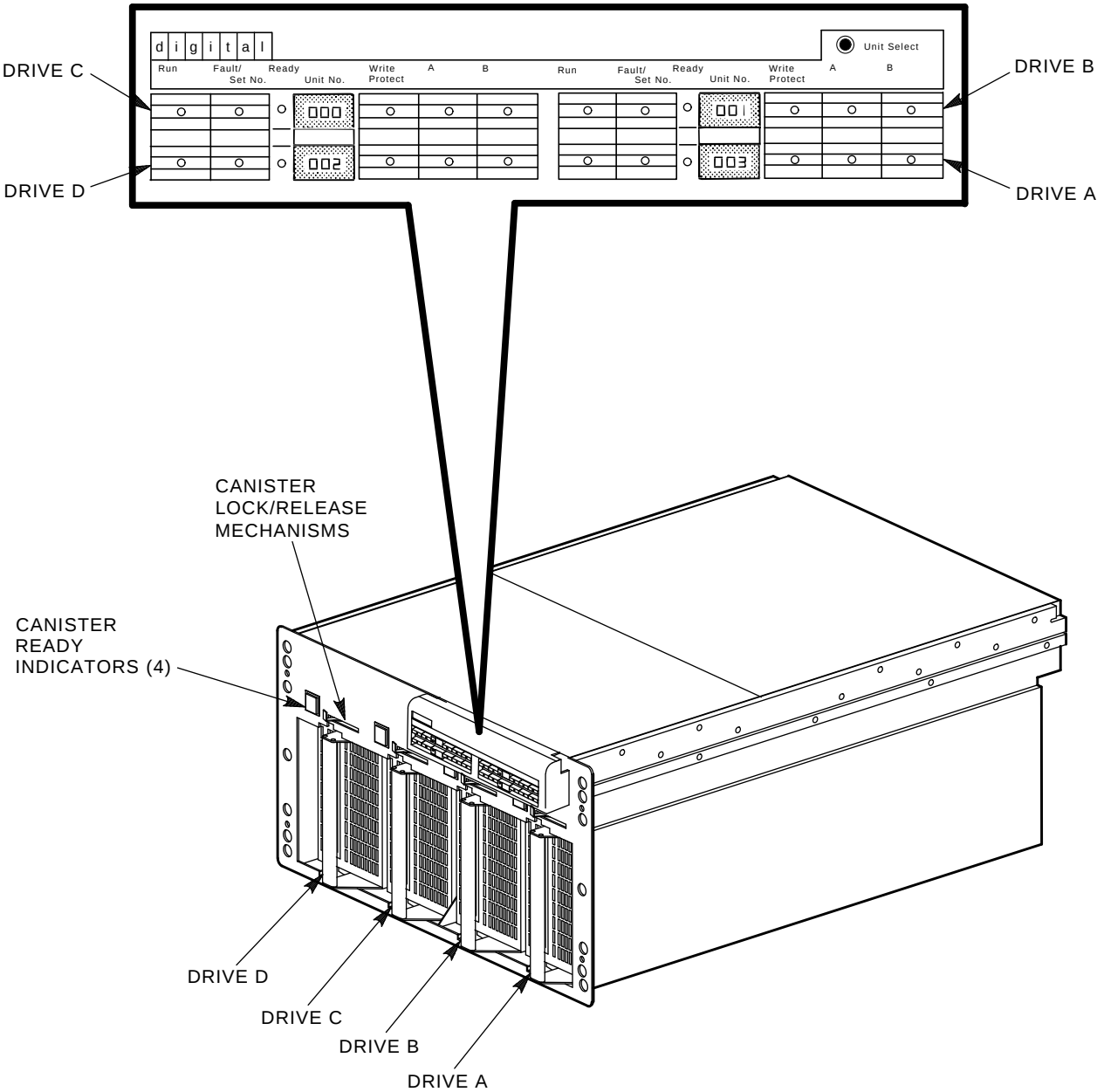
Figure 3-4 SA70R-AK Enclosure Front Panel
