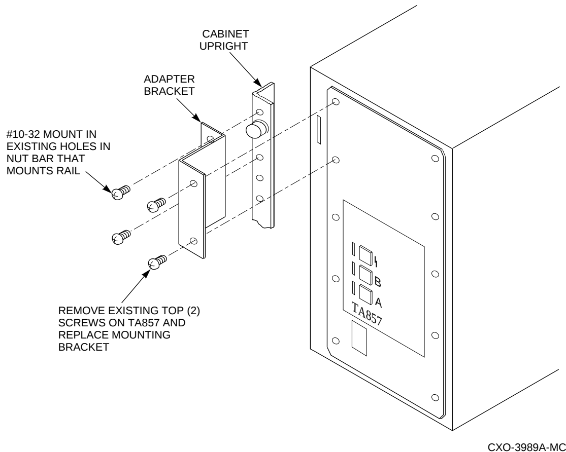
Figure 5-42 Installing Mounting Brackets
