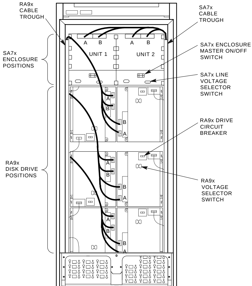
Figure 3-16 Power and Line Voltage Selector Switches
