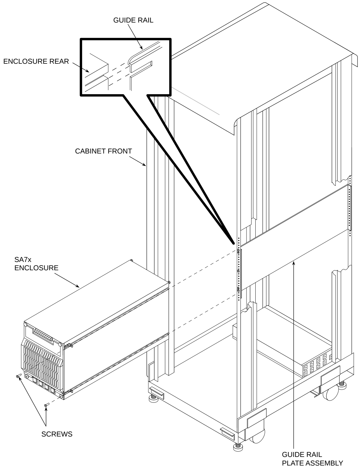
Figure 5-38 Installing the SA7x Enclosure in the SA900
