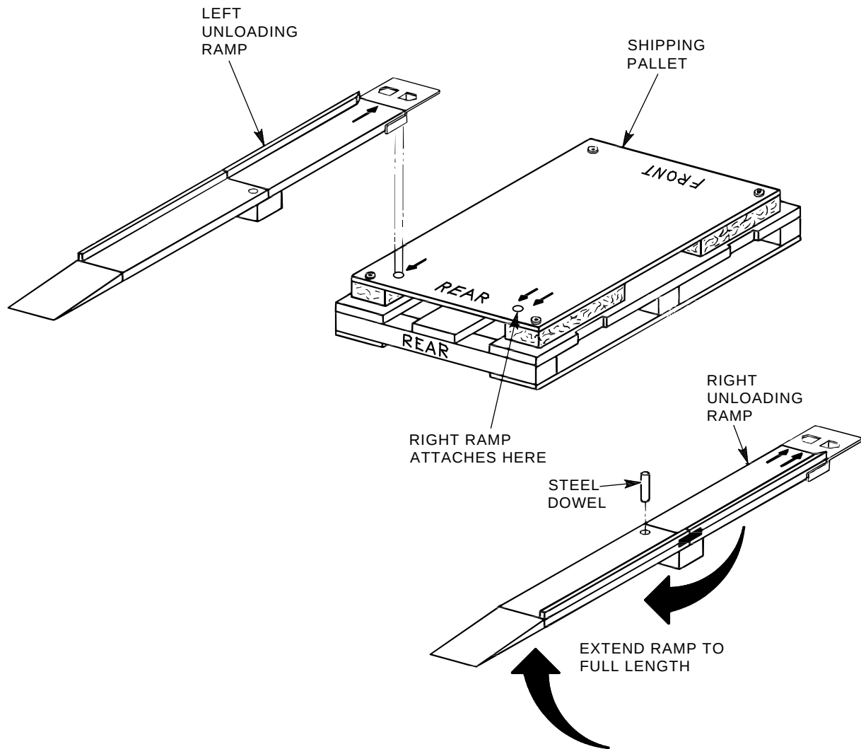
Figure 3-4 H9646 Unloading Ramps
