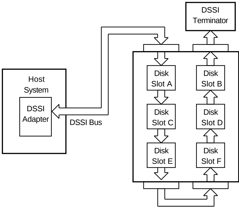
Figure 4-1 Through-Bus Mode
