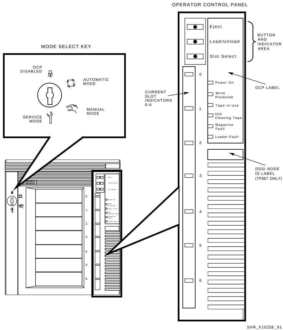
Figure 2-1 TF8x7 Operator Control Panel
