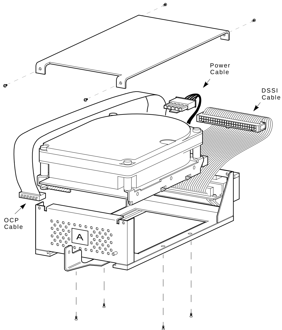
Figure 5-4 Disk ISE Replacement
