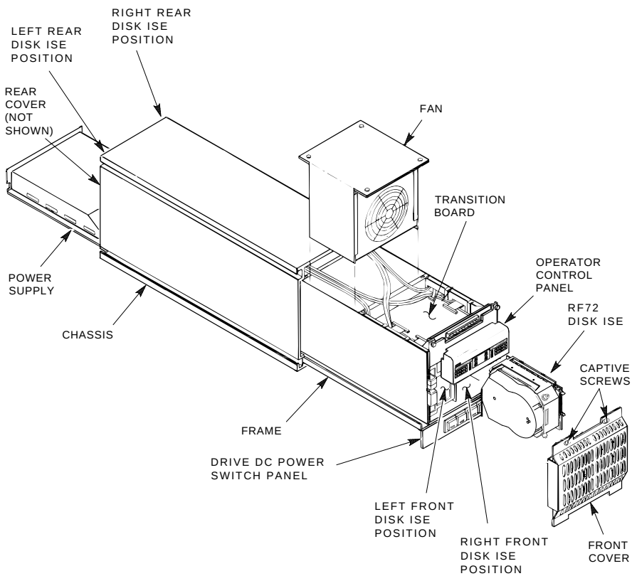
Figure 6-1 Storage Enclosure Exploded View
