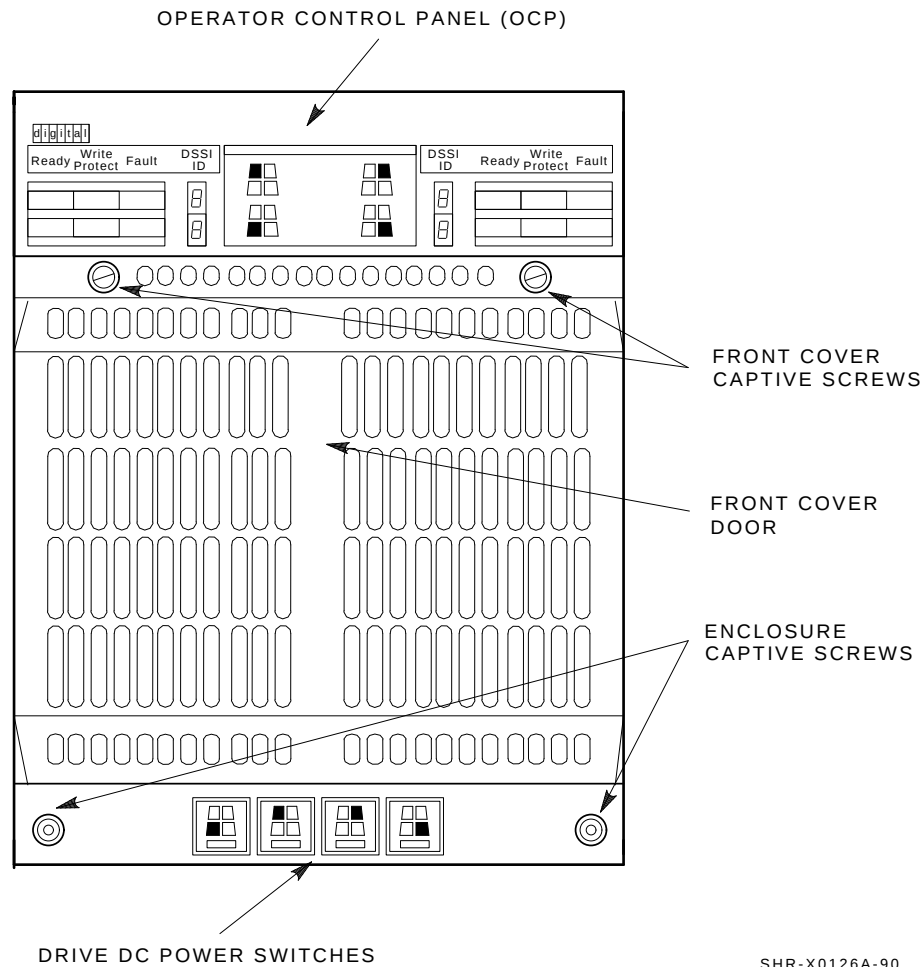
Figure 6-2 Storage Enclosure Front View
