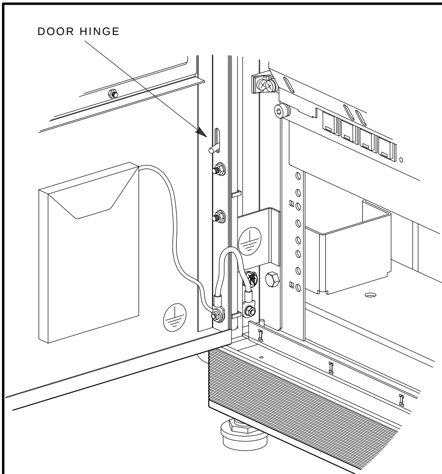
Figure 4-1 Removing DECarray Door
