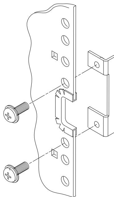
Figure 5-7 AC Power Cord Retainer
