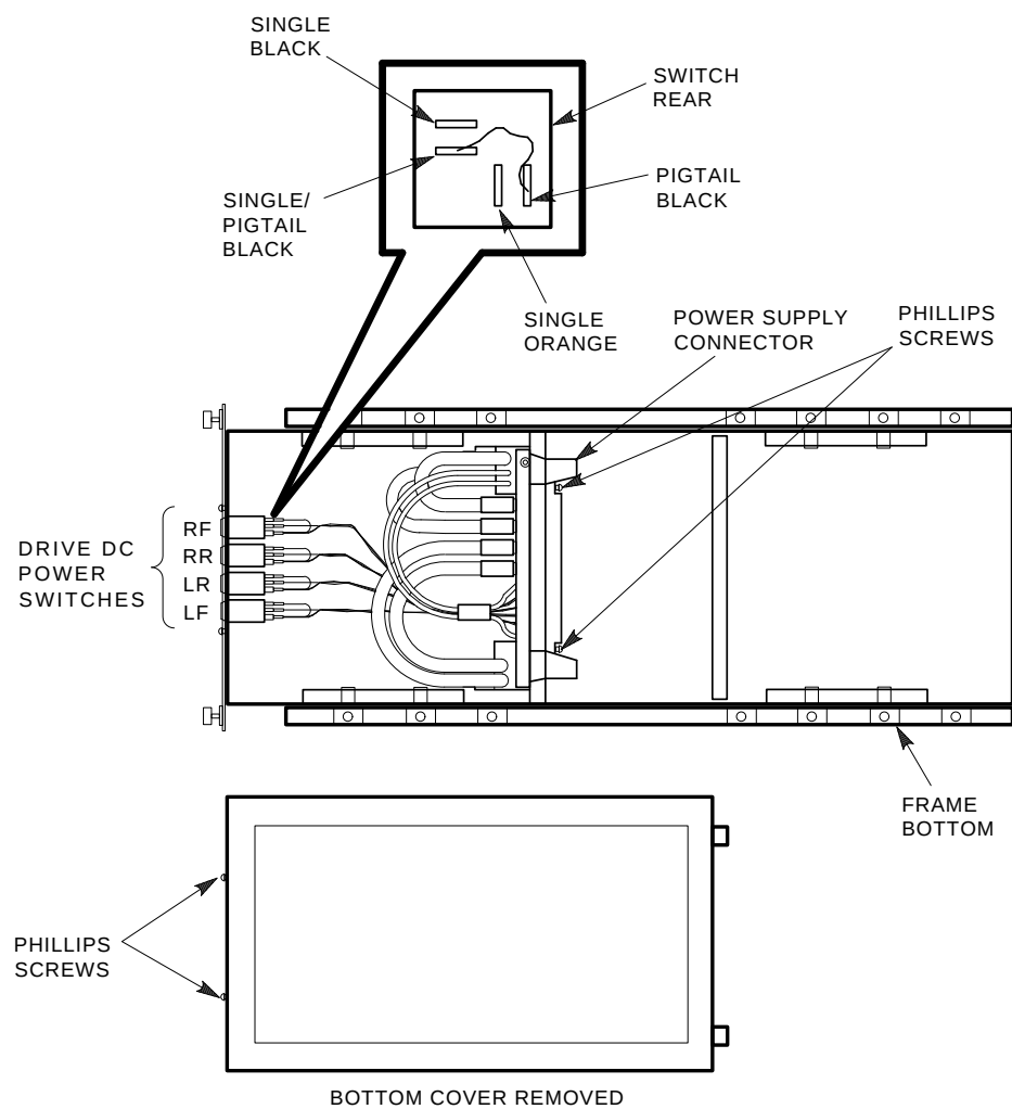
Figure 6-13 Removing and Replacing the Drive DC Power Switches
