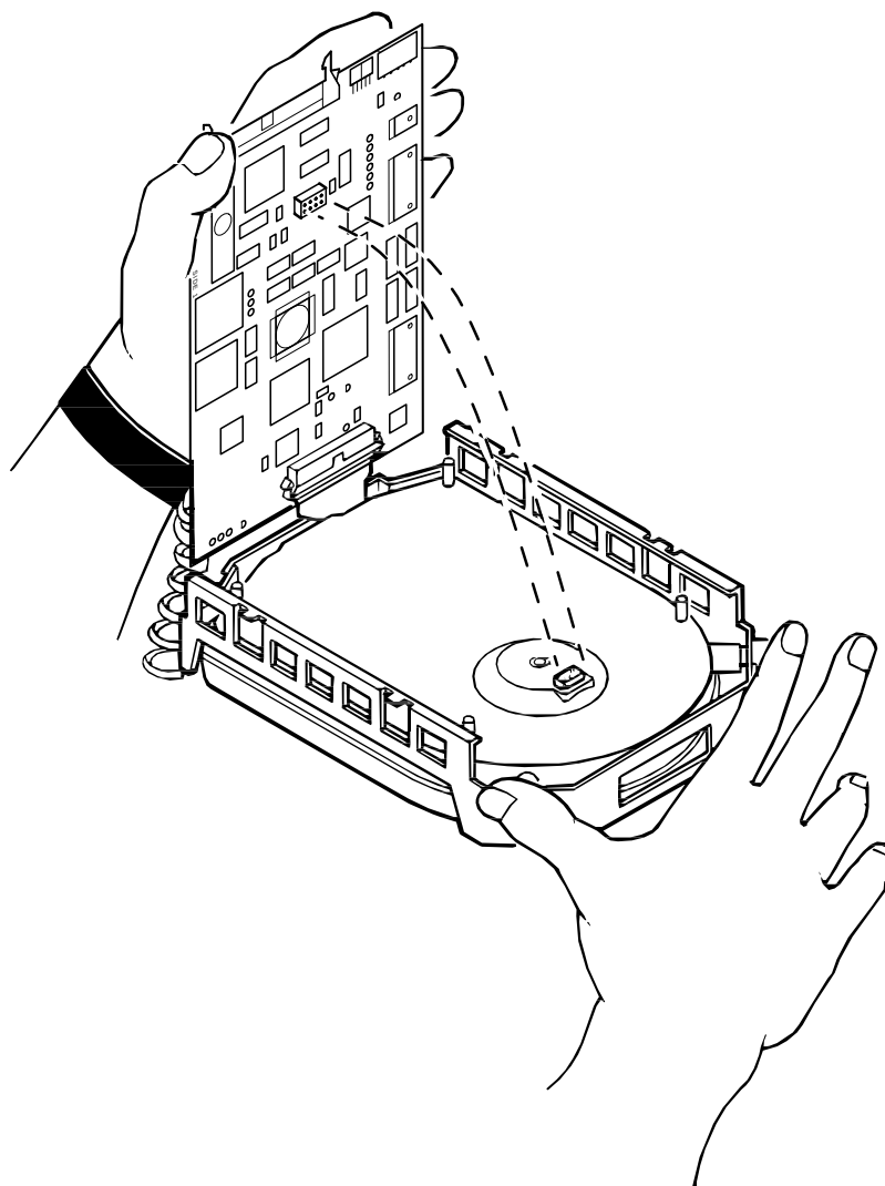
Figure 6-5 Separating the HDA from the Drive Module
