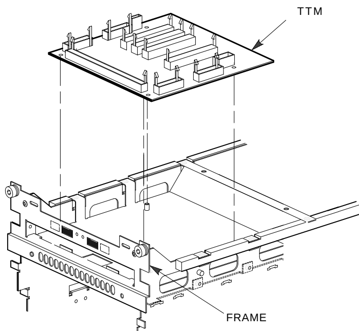
Figure 6-12 Removing and Replacing the Transition-Termination Module
