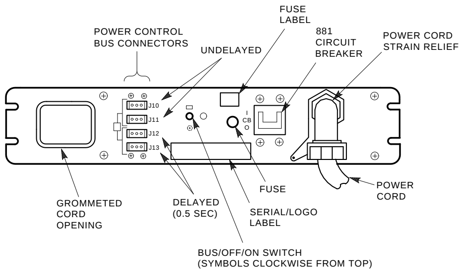
Figure 4-2 Power Controller
