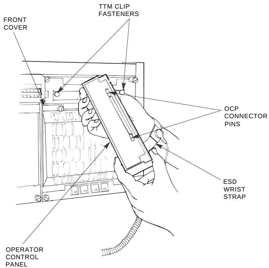
Figure 6-9 Removing the OCP
