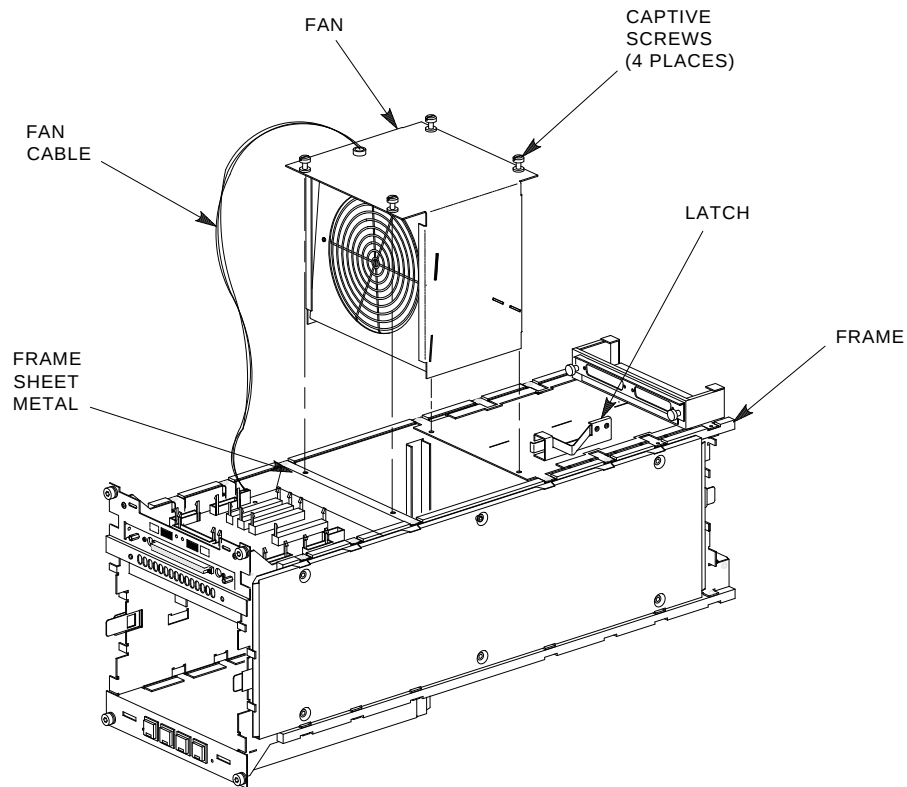
Figure 6-11 Removing and Replacing the Fan Assembly
