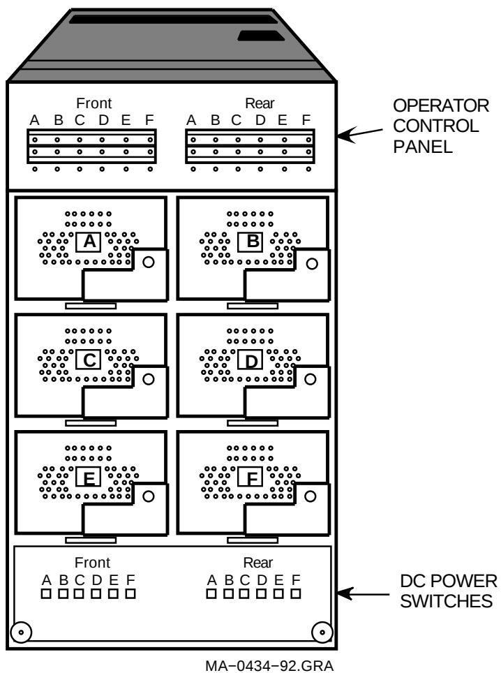
Figure 2-2 Front View of the SF3x Storage Enclosure (with cover removed)
