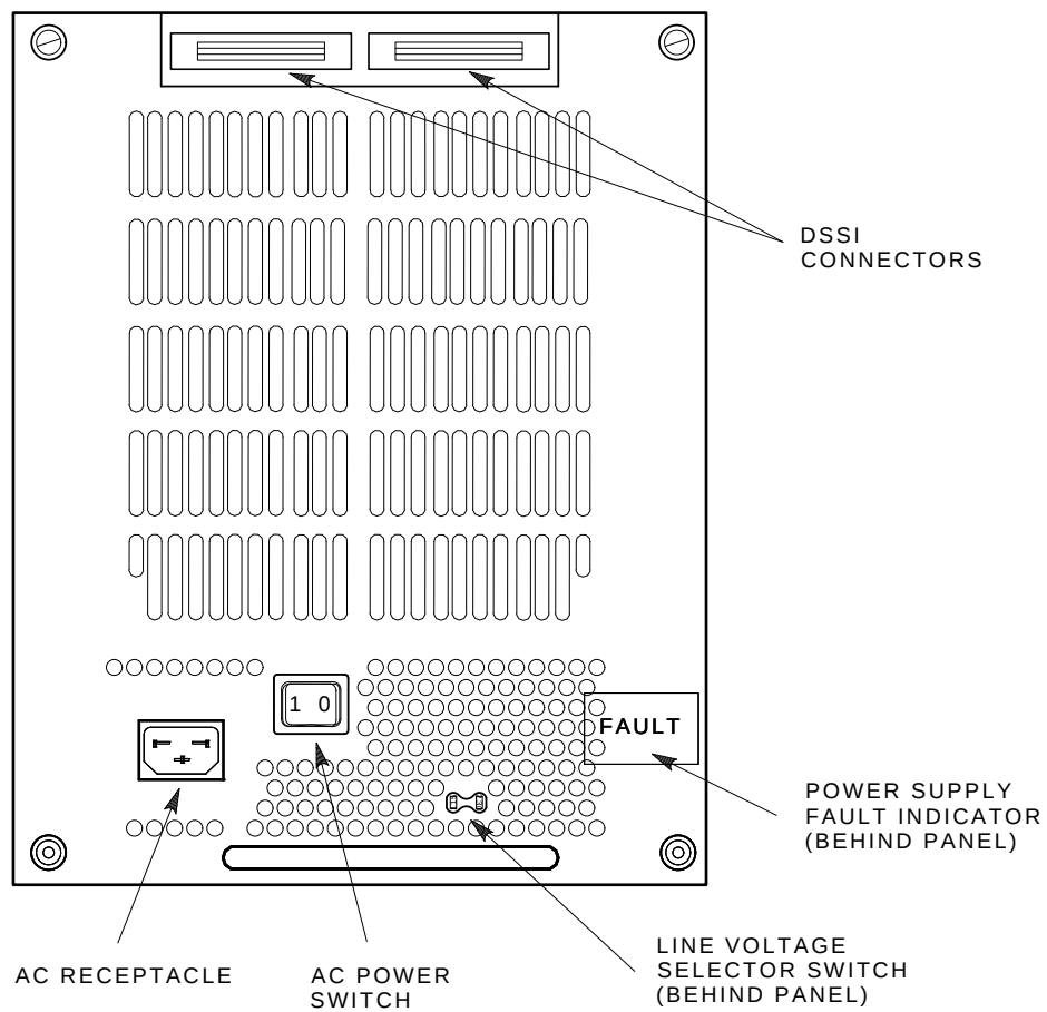
Figure 6-10 Storage Enclosure Rear View
