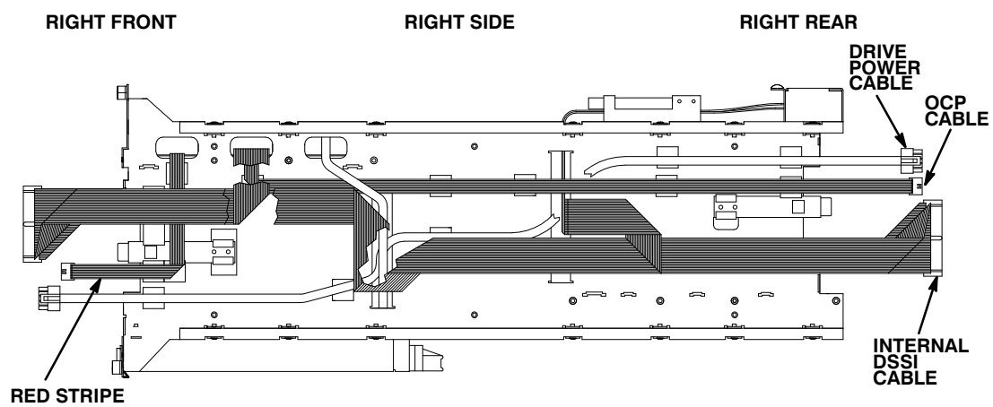
Figure 6-19 Enclosure Internal DSSI Cables (cont.)
