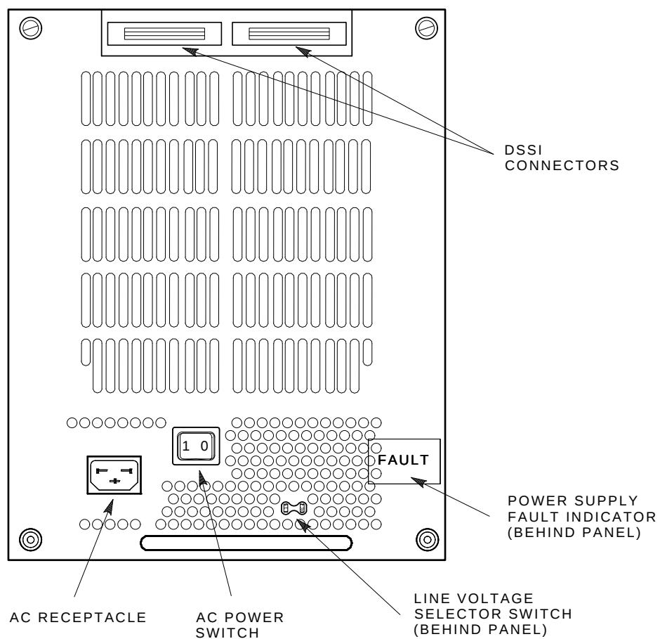
Figure 6-21 Storage Enclosure Rear View
