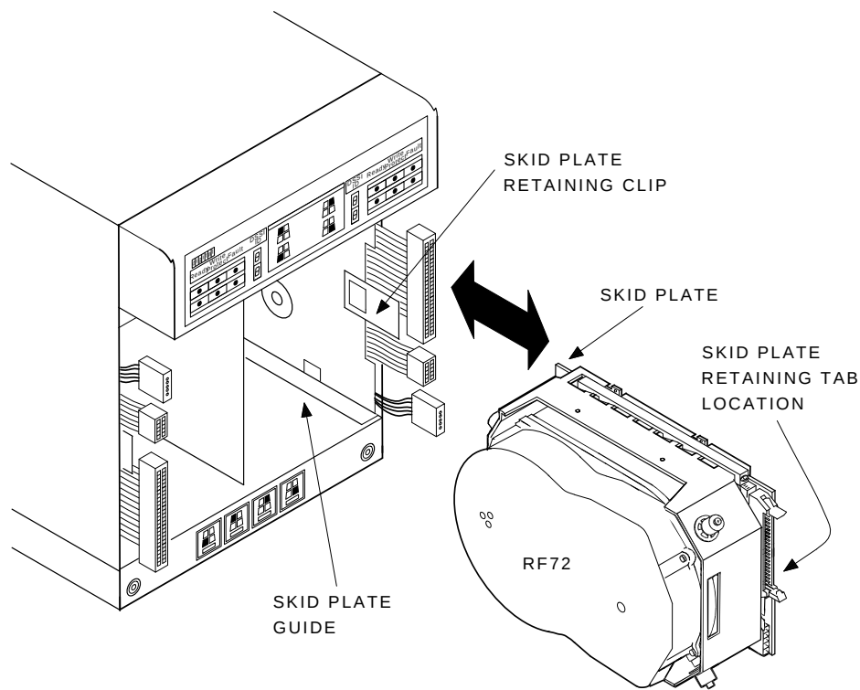
Figure 6-3 Removing and Replacing a Disk ISE
