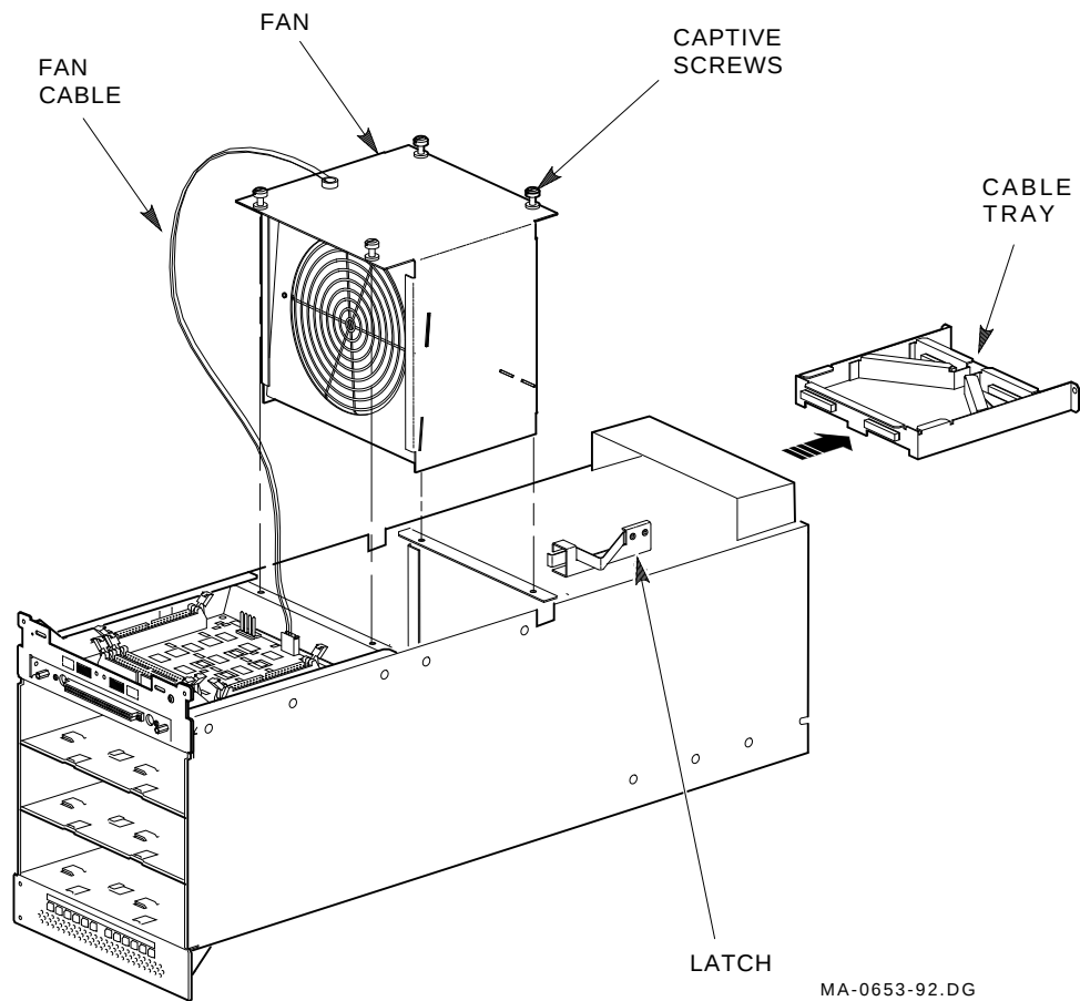
Figure 5-5 Removing and Replacing the Fan Assembly
