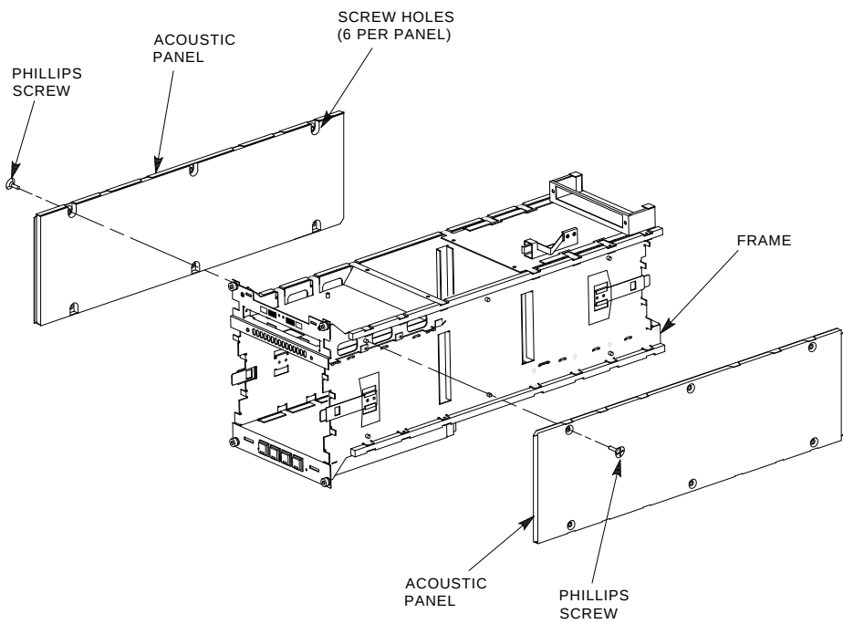
Figure 6-17 Removing the Acoustic Panels
