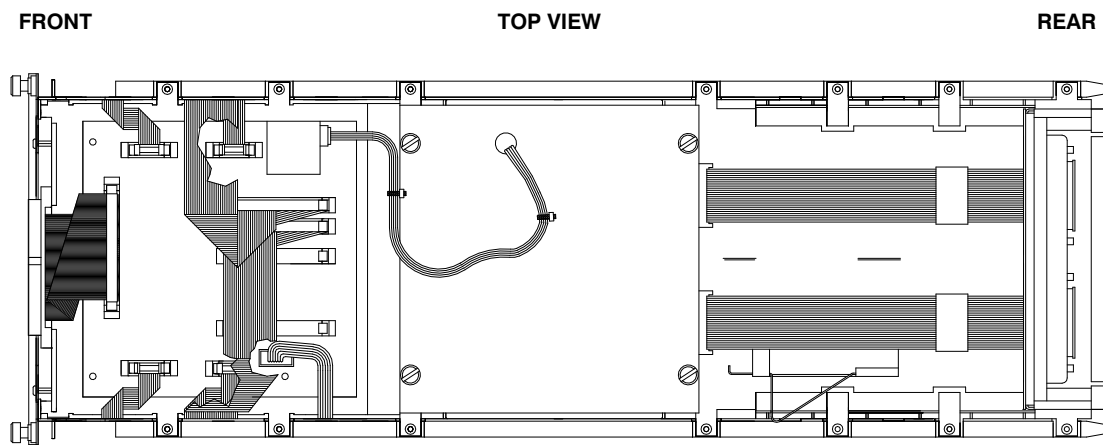
Figure 6-18 Enclosure Internal DSSI Cables
