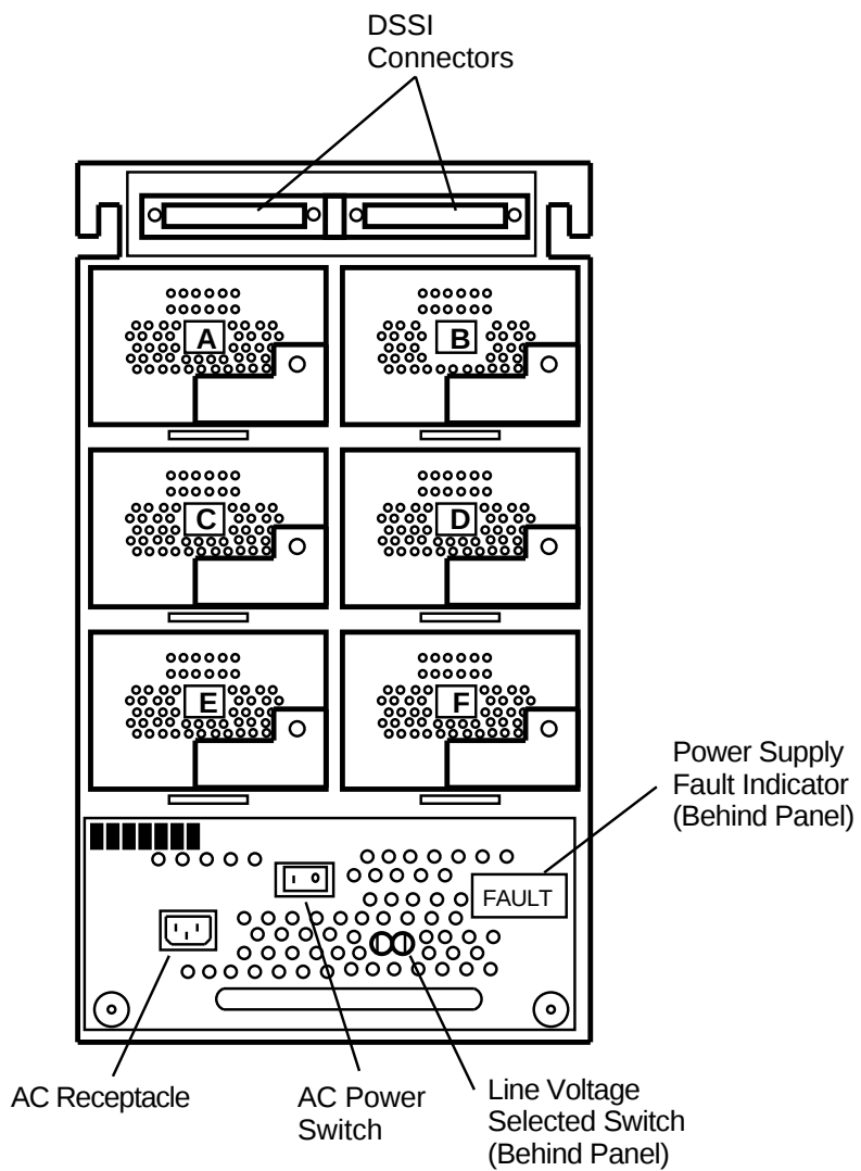
Figure 2-4 Rear Panel of the Storage Enclosure (with cover removed)
