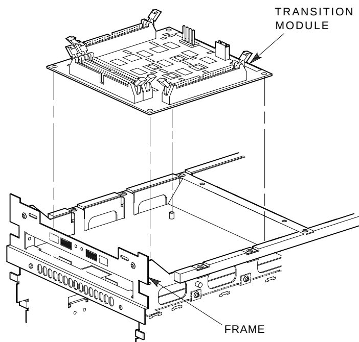
Figure 5-6 Removing and Replacing the Transition Module
