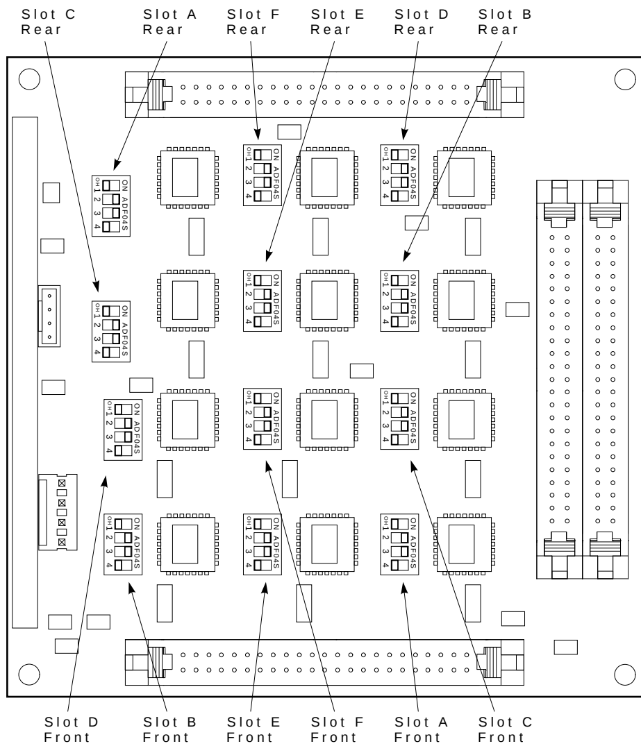
Figure 2-1 SF3x DSSI Node ID Switches
