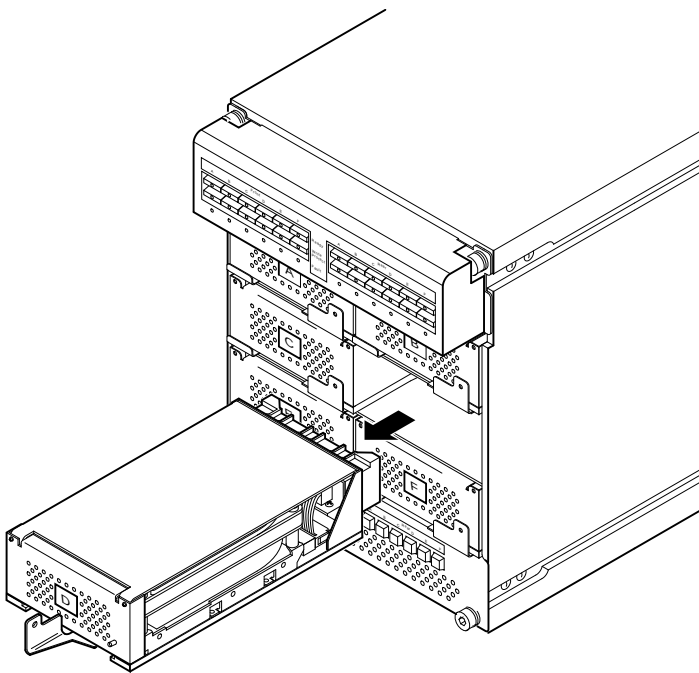
Figure 5-3 Disk ISE Removal
