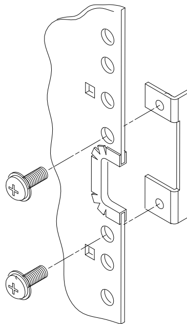
Figure 6-14 AC Power Cord Retainer
