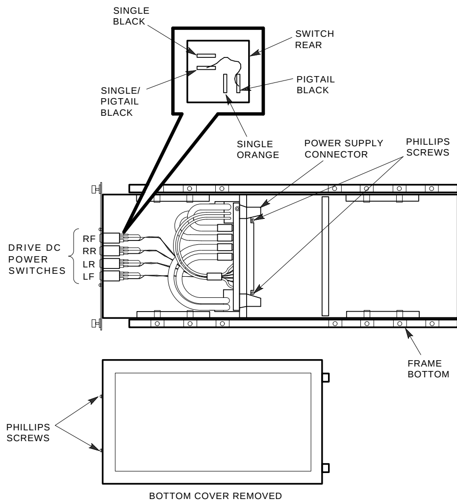
Figure 6-16 Storage Enclosure Power Harness
