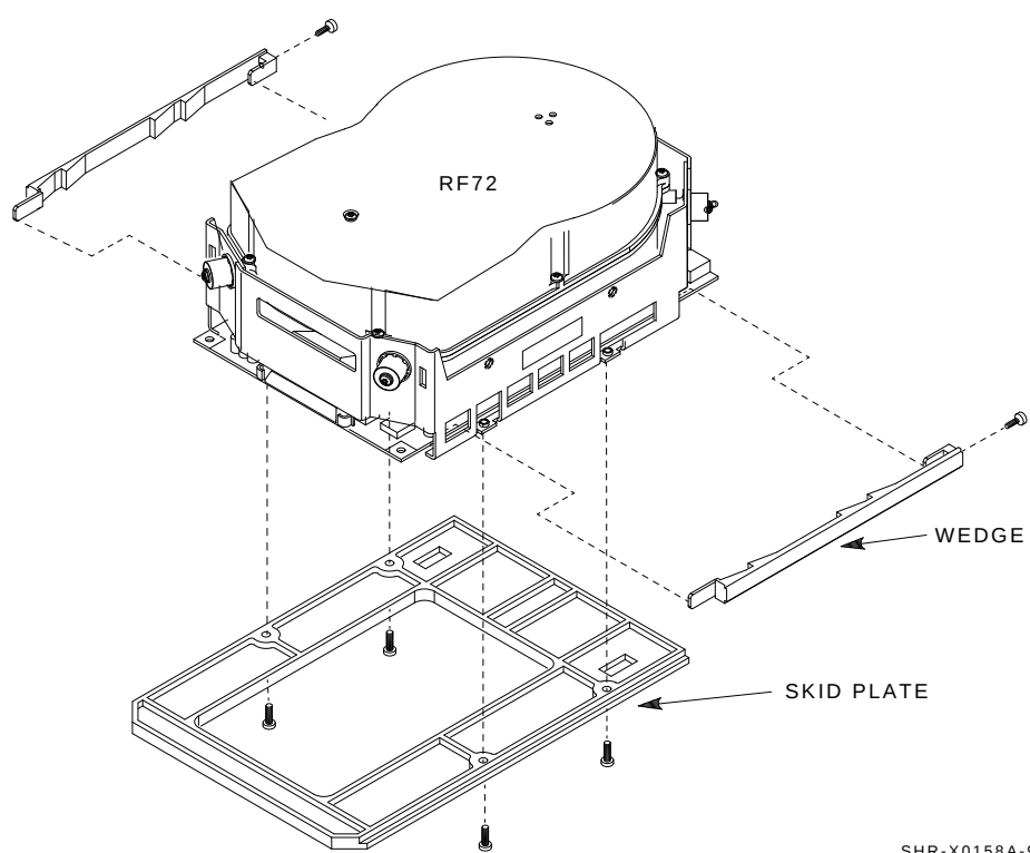
Figure 6-4 Disk ISE Skid Plate and Wedges
