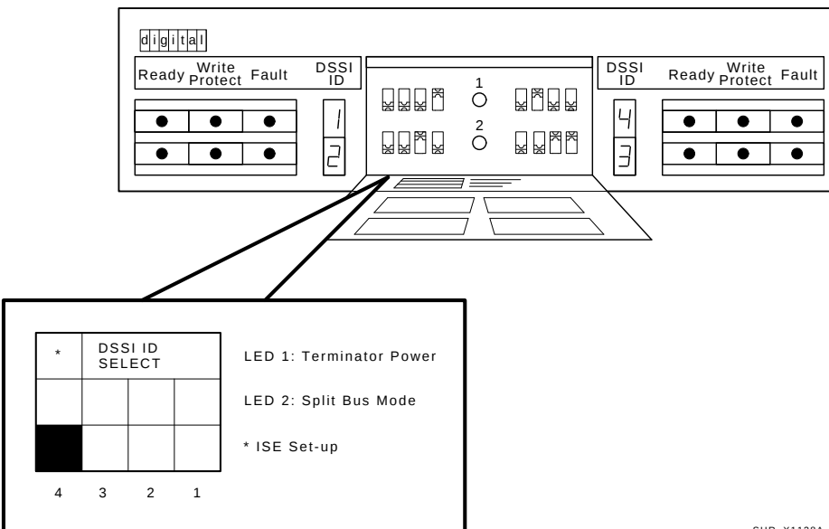
Figure 6-8 OCP MSCP Switch
