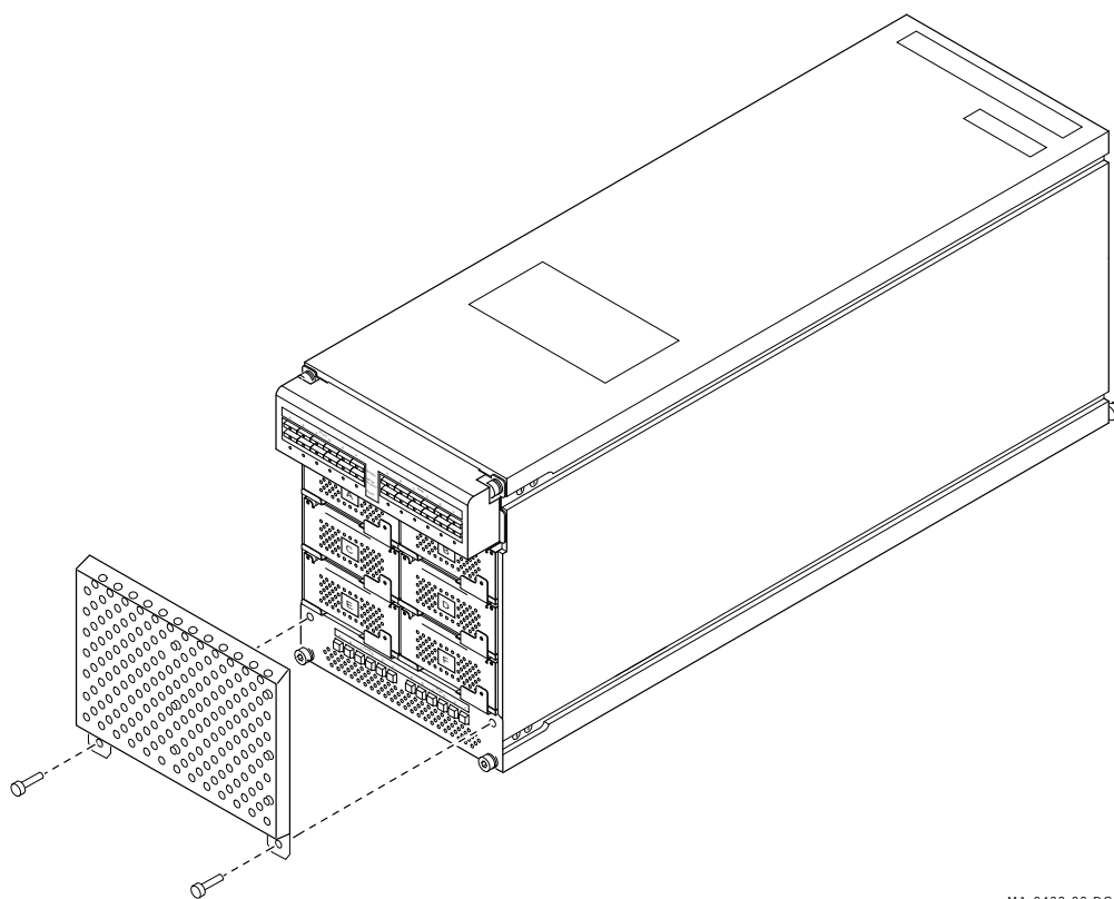
Figure 1-2 SF3x Series Storage Enclosure
