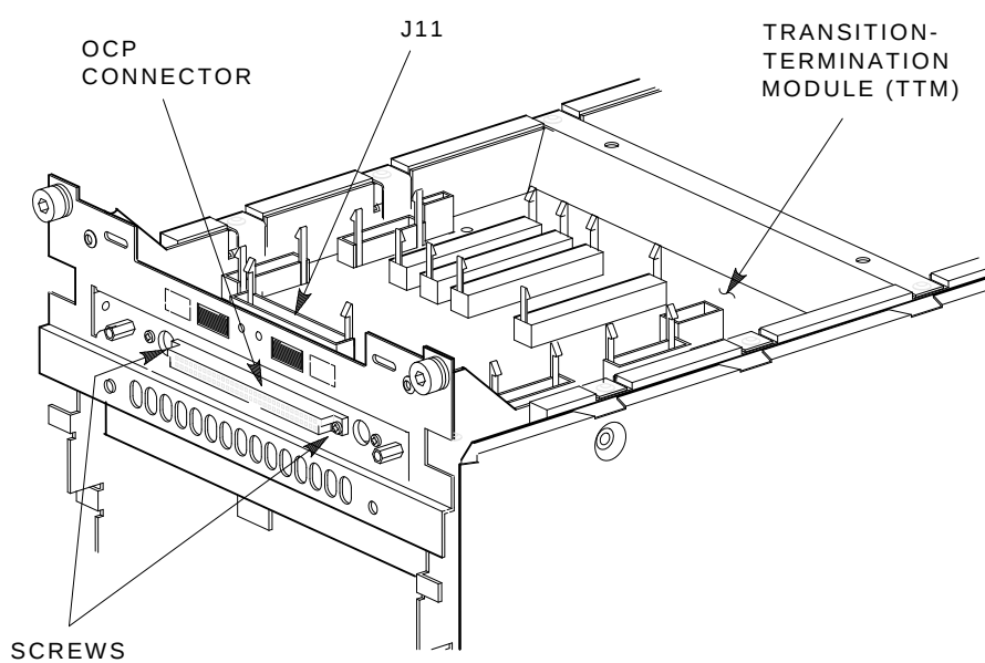
Figure 6-15 Removing and Replacing the OCP to TTM Cable
