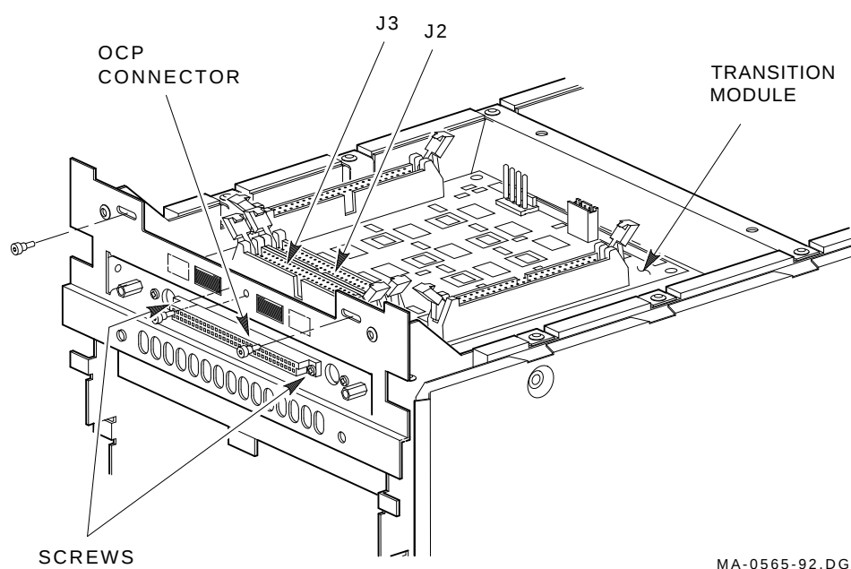
Figure 5-8 Removing and Replacing the OCP to TM Cable
