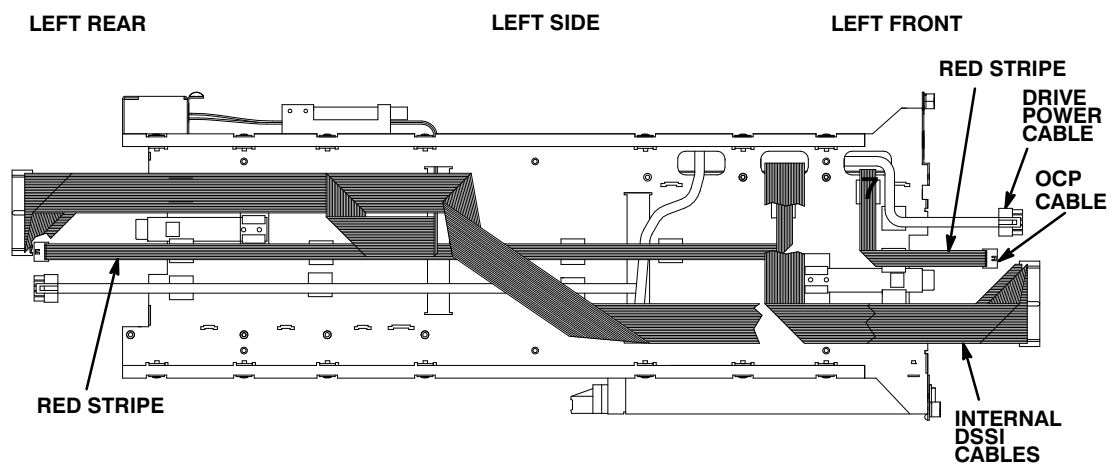
Figure 6-20 Enclosure Internal DSSI Cables (cont.)
