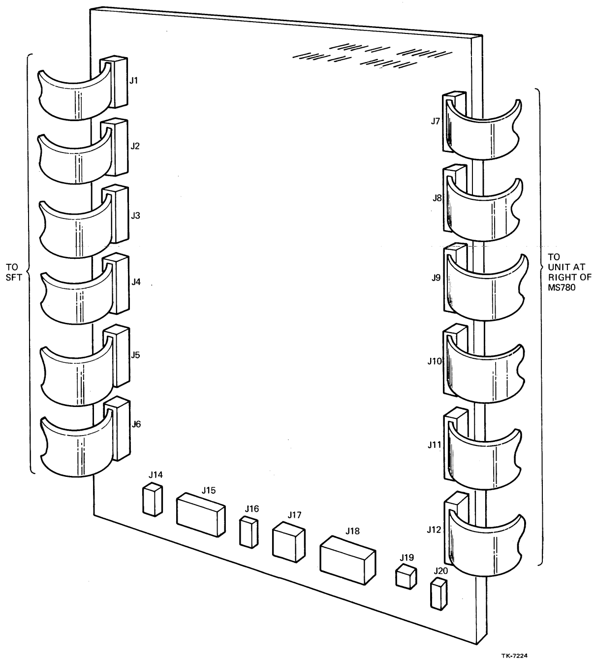
Figure 8-1 MS780 Installation Details
