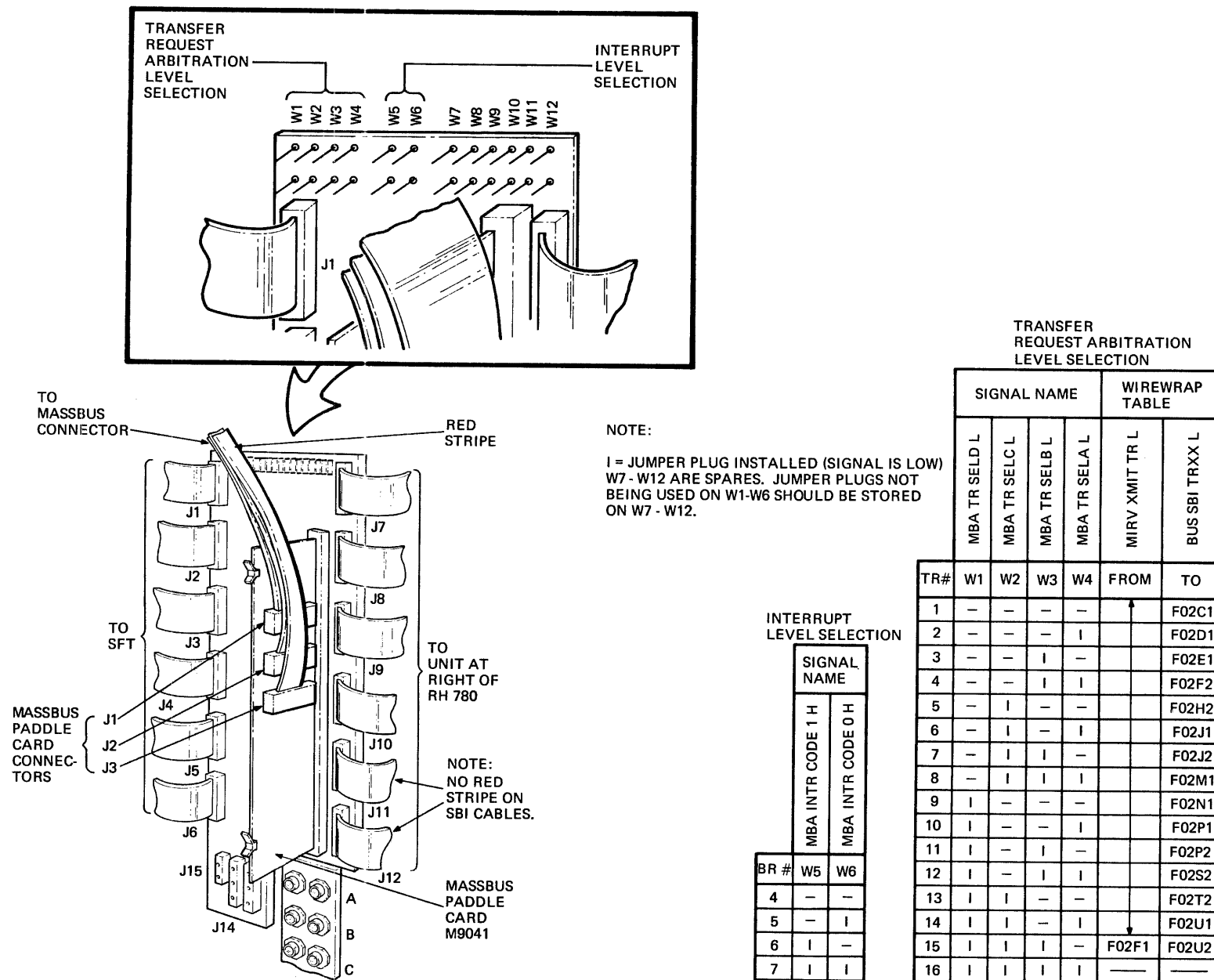
Figure 7-2 Transfer Request Arbitration, Interrupt Level Details
