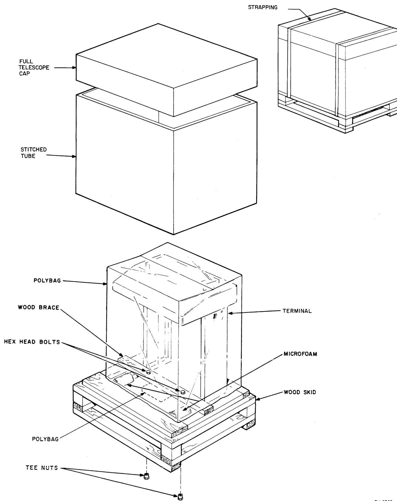
Figure 1-13 Console Packaging
