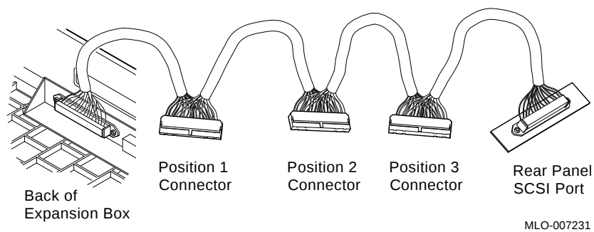
Figure 2–18 SCSI Cable and Connectors
