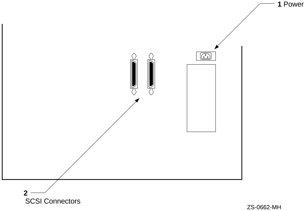
Figure 5-4 Large Optical Library Rear Panel (RW514/516/534/536-ZF)
