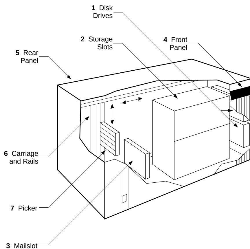
Figure 1-3 Rackmount Optical Library Components (RW511-ZC)
