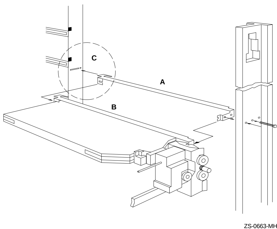
Figure 3-3 Positioning the Shipping Bracket (Large Unit RW514/516/534 /536-ZF)
