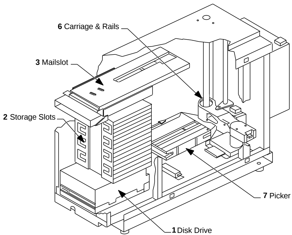
Figure 1-1 Small Optical Library Components (RW504/524-ZA)
