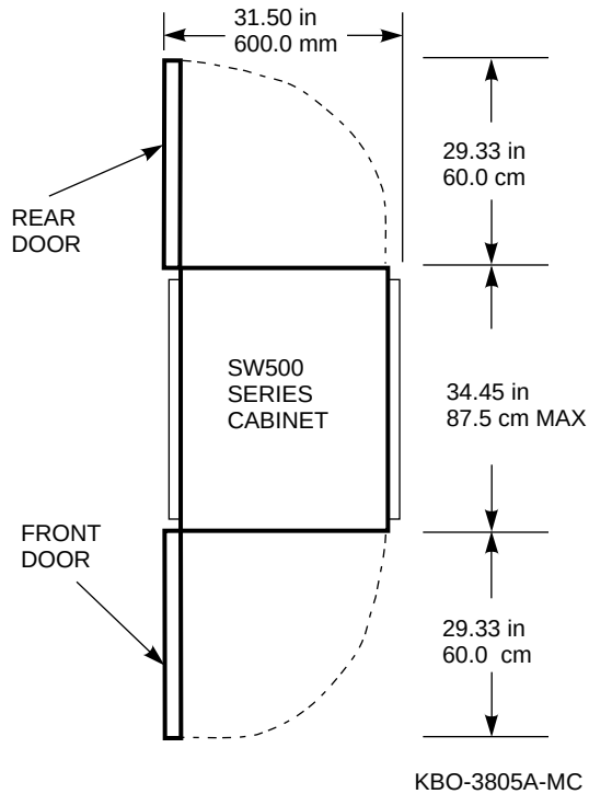
Figure 3–1 Minimum Installation Clearances
