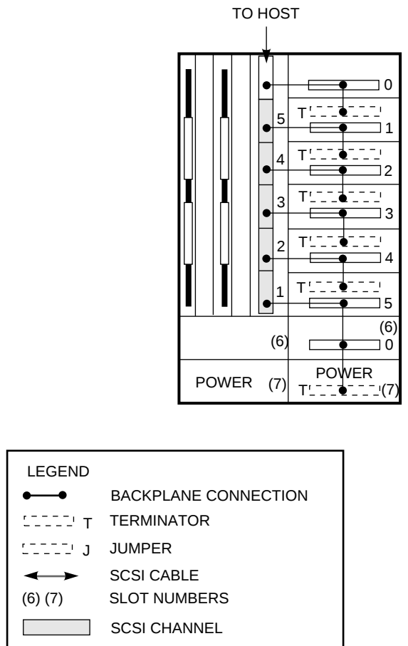
Figure 7-8 Single BA350-EA Shelf
