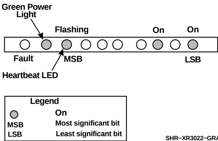
Figure 6–2 LED Indicators
