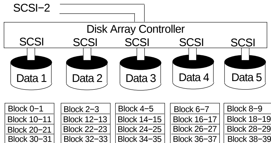
Figure 3–2 Diagram of RAID 0
