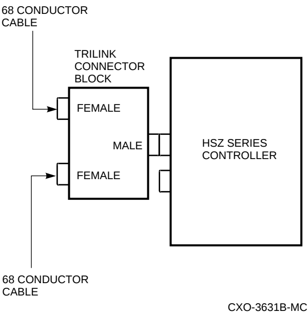
Figure 5-3 Trilink Connector Midbus Connection
