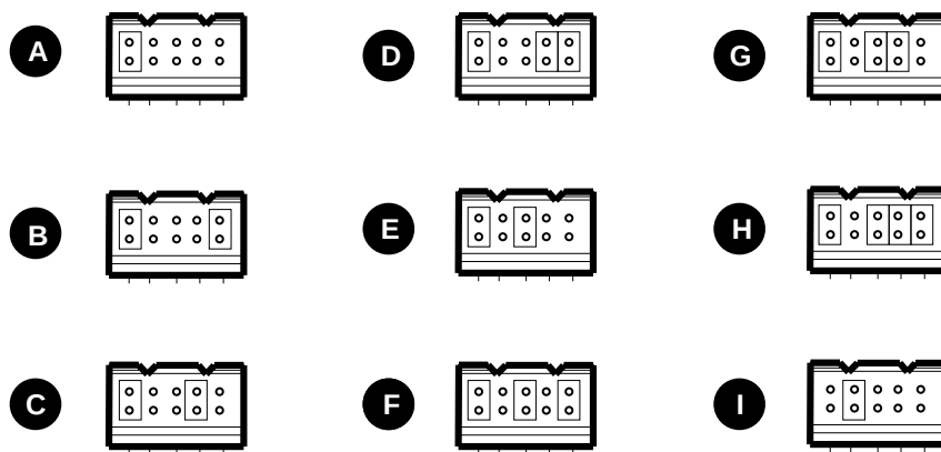
Figure 3-3 Jumper Positions
