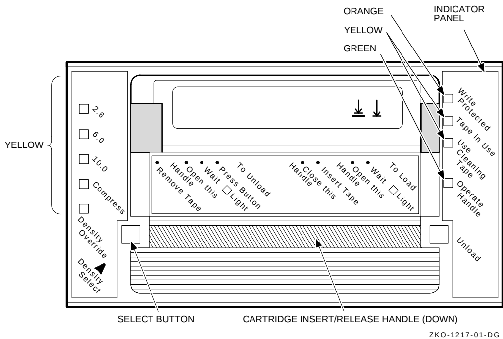
Figure 3-6 DLT2000 Indicators
