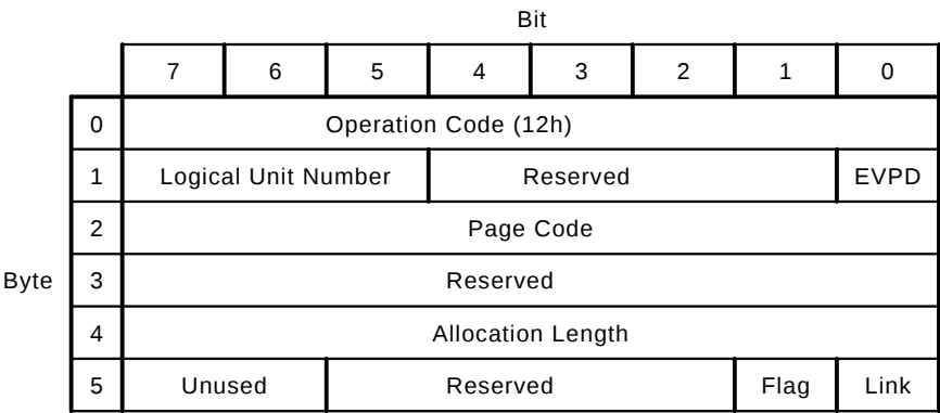
Figure 7-4 INQUIRY CDB
