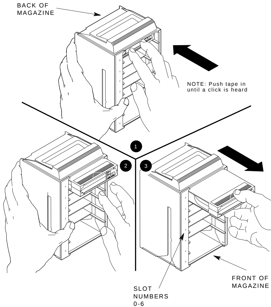
Figure 4-6 Removing a Cartridge from the Front of the Magazine
