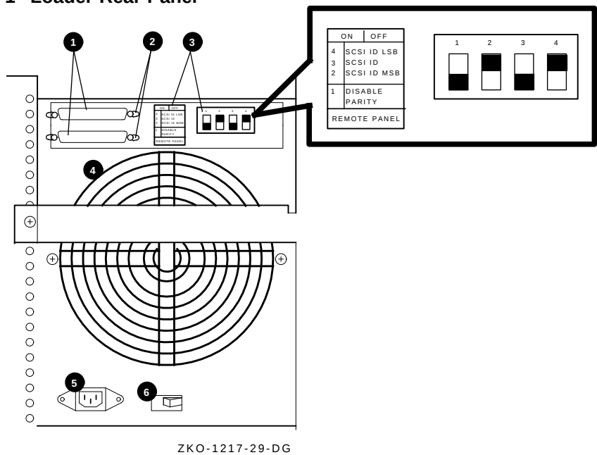
Figure 4-1 Loader Rear Panel
