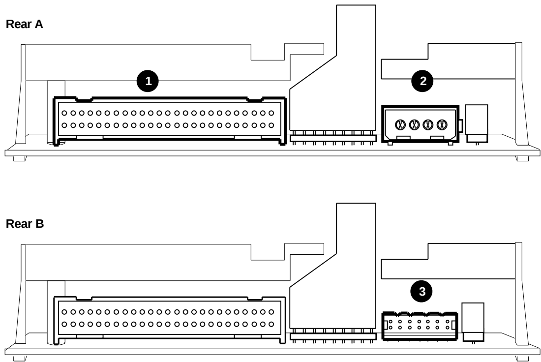
Figure 3-5 DLT2000 Rear Connectors
