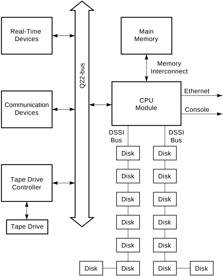
Figure 1-1: VAX 4000 Model 300 Block Diagram
