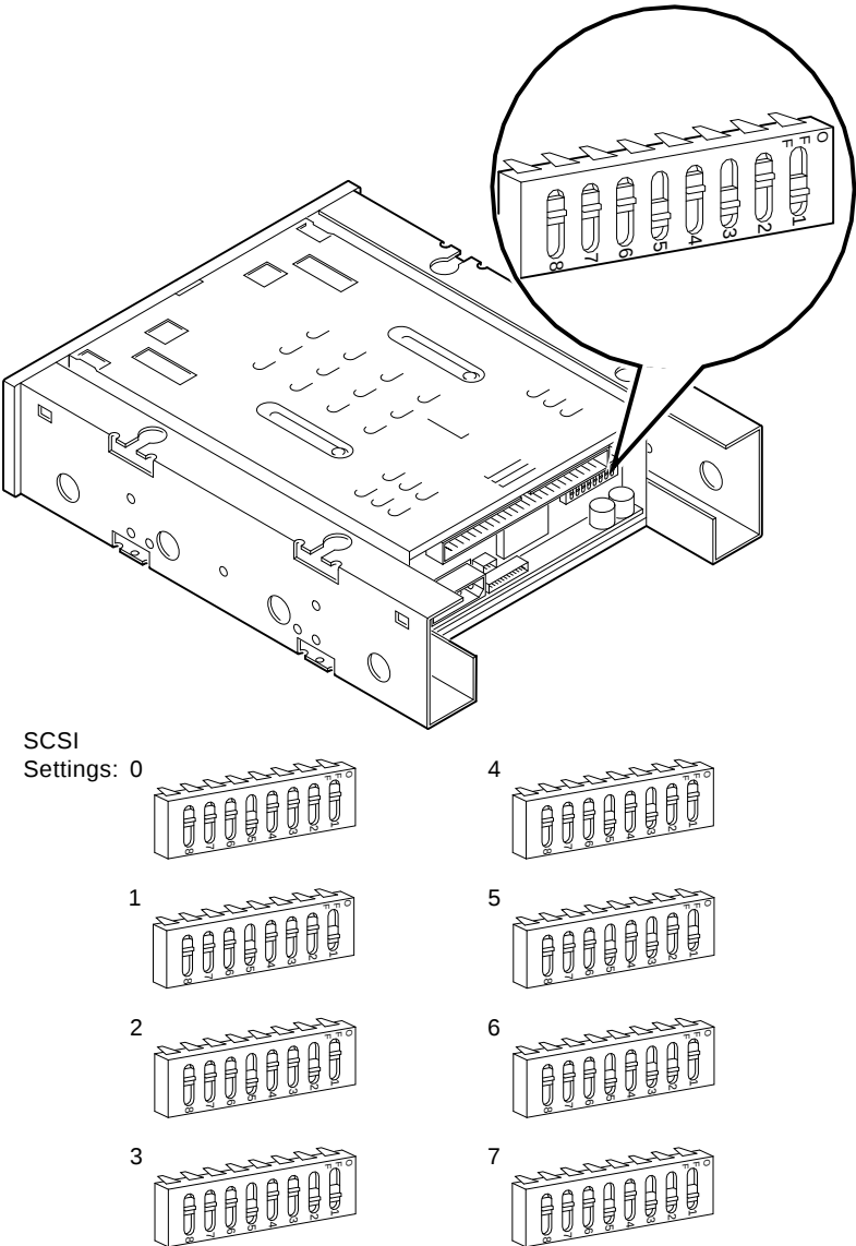
Figure 5-2 TLZ06 Mode and SCSI Address Switches
