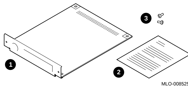
Figure 10–2 TURBOchannel Option Components
