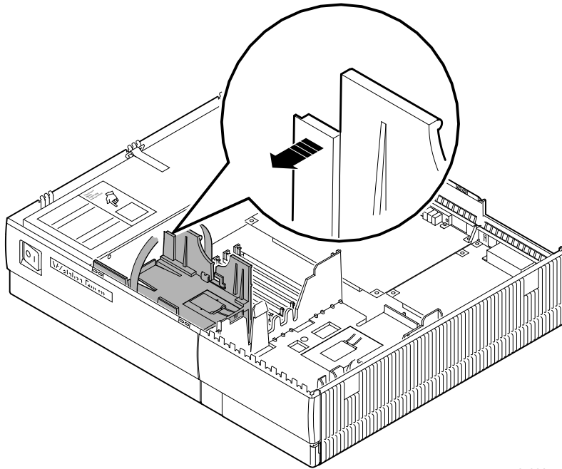
Figure 6–8 Removing the H-Bracket from the System Unit
