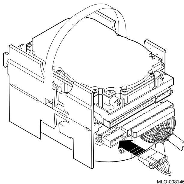
Figure 6–15 Connecting the Power Cable to the Disk Drive
