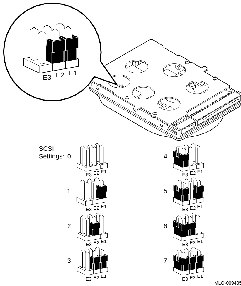
Figure 6-1 Setting the RZ23L Drive SCSI ID
