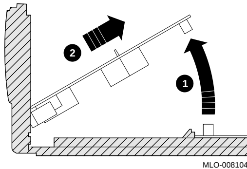
Figure 2-6 Removing the Diagnostics Board
