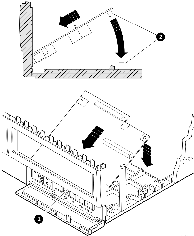
Figure 5-10 Replacing the Diagnostics Board
