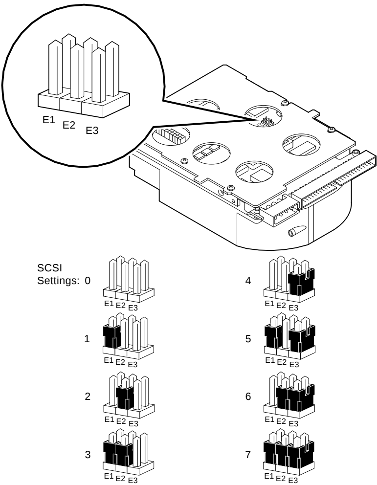
Figure 6-2 Setting the RZ24 Drive SCSI ID
