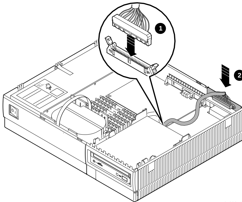
Figure 10–9 Replacing the SCSI Cables
