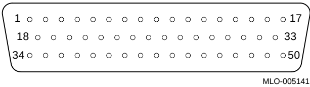
Figure C-1 Synchronous Communications Port Pins
