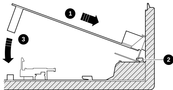
Figure 8-14 Installing an LCSPX Graphics Board
