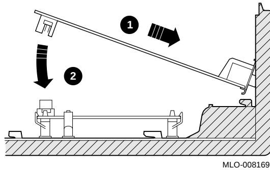
Figure 10–8 Inserting the TURBOchannel Option
