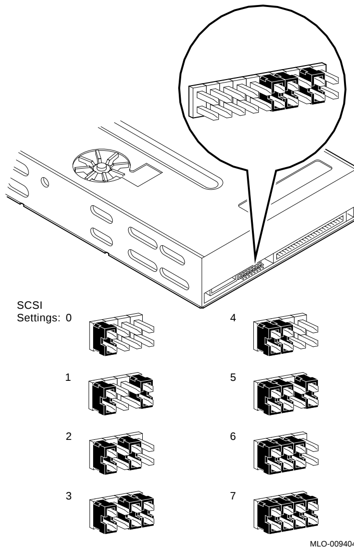
Figure 4-2 Verifying the TZK10 Tape Drive SCSI ID
