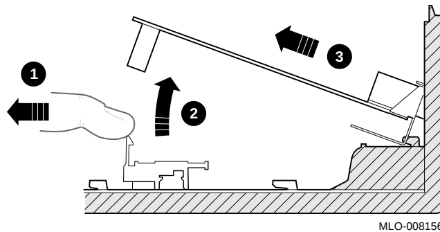
Figure 8–9 Removing an Existing LCG Board
