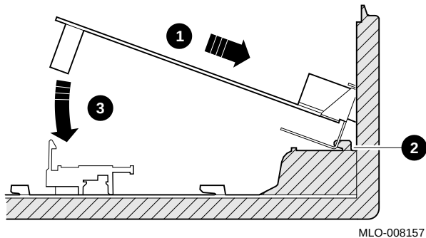
Figure 8-13 Installing an LCG Board
