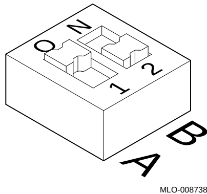
Figure E-1 Setting the Refresh Rate
