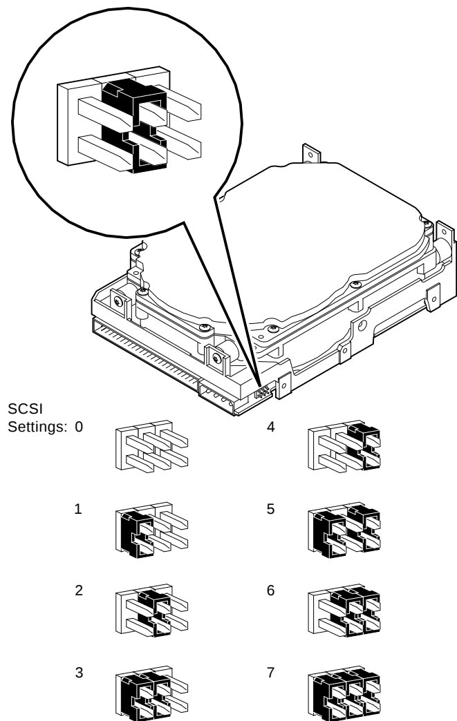
Figure 6-4 Setting the RZ25 Drive SCSI ID
