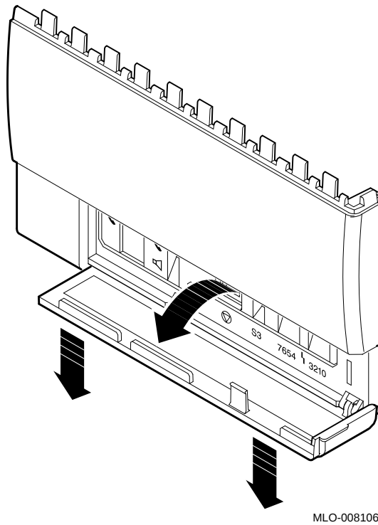
Figure 5–8 Removing the Door from the Bezel
