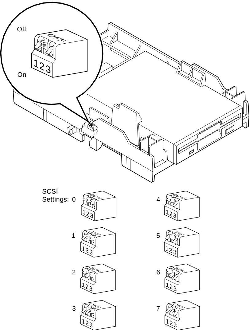
Figure 3-2 Setting the RX26 Diskette Drive SCSI ID
