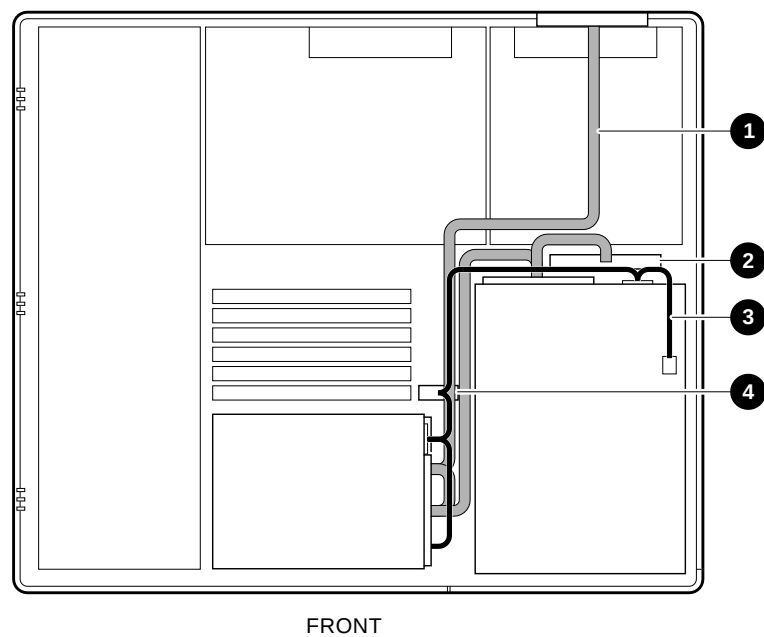
Figure 11-1 Routing Cables
