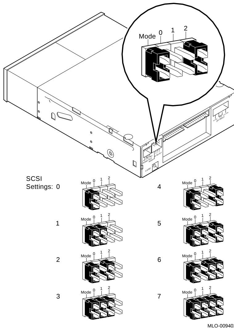
Figure 2-2 Verifying the RRD42 Drive SCSI ID
