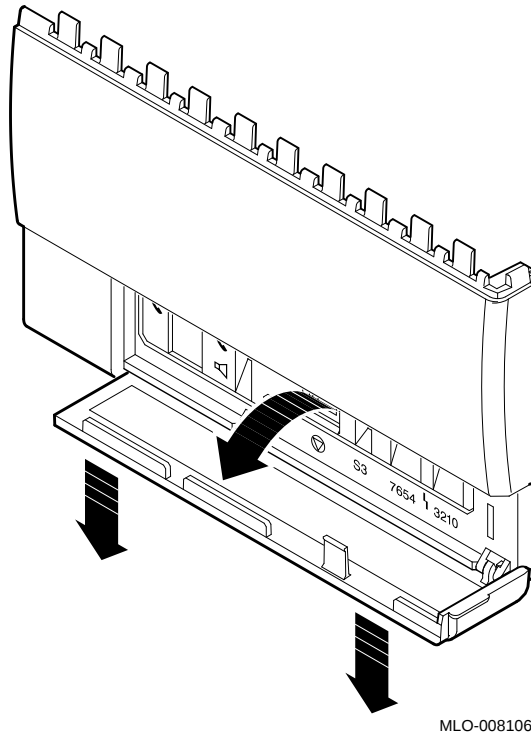
Figure 3-8 Removing the Door from the Bezel
