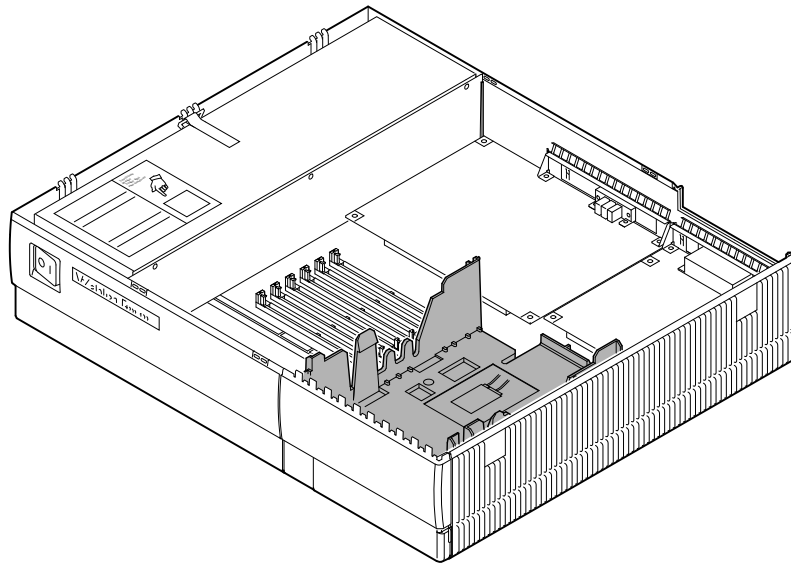
Figure 5-3 Location of the Removable Media Bracket
