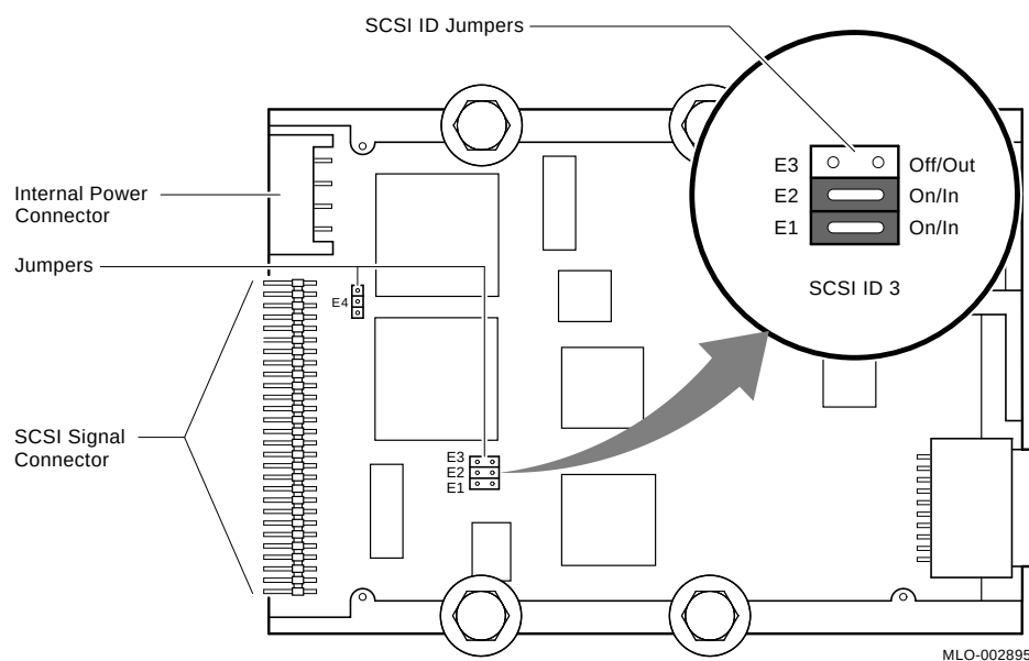
Figure 3-3 RZ5x Disk Drive SCSI ID Jumper Location
