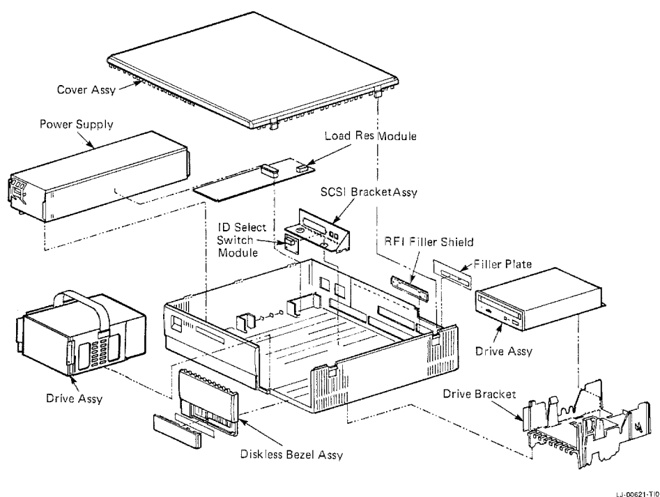
Figure 1-1 BA46 Storage Expansion Box
