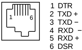
Figure A-4 MMJ Adapter Pins
