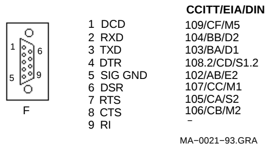
Figure A-2 9-Pin EIA 232 Port
