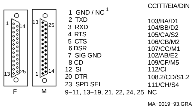
Figure A-1 Serial Communication/Printer Ports 1
