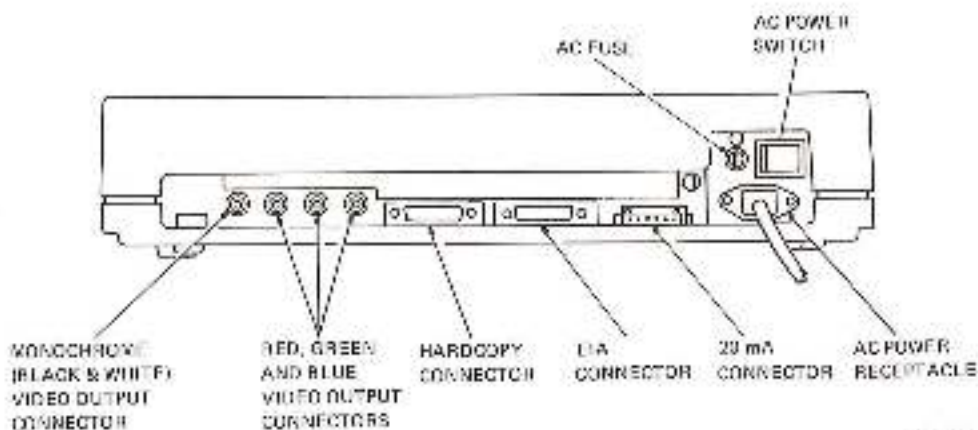
FIGURE 3-1 Terminal Controls
