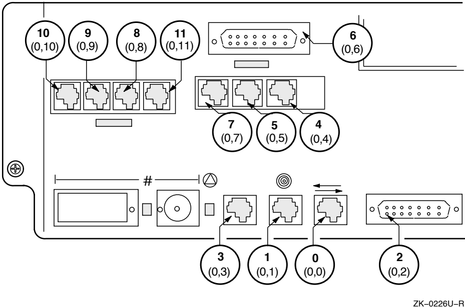
Figure 2-4: DECsystem 5100 KN230 with Async Terminal Ports
