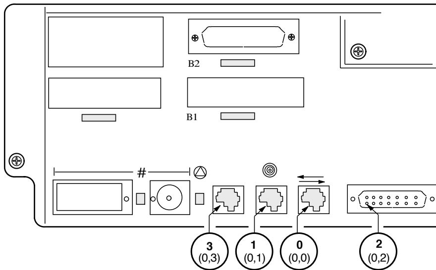
Figure 2-3: DECsystem 5100 Console and Terminal Ports
