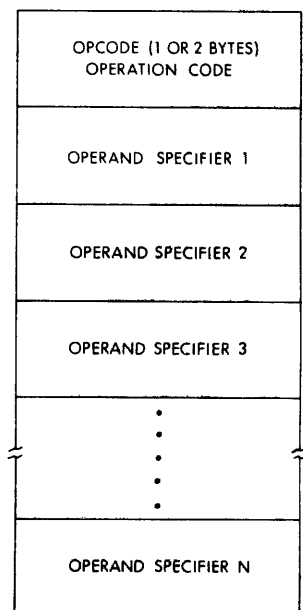
Figure 5-1 General VAX-11 Instruction Format
