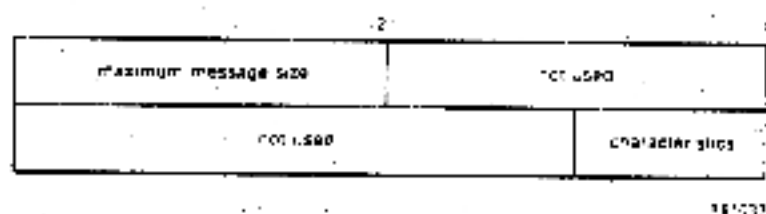
Figure 3-1 P1 Characteristics Buffer (Set Controller)
