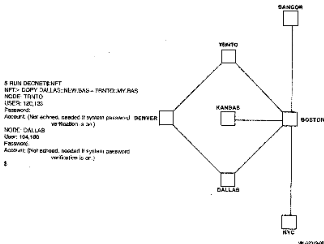
Figure 4-1: NFT Transfers Files to, from, and between Remote Nodes
