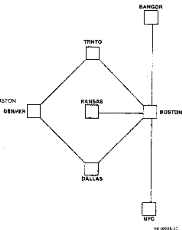
Figure 3-1: NET Provides Access to Another DECnet/E Node
