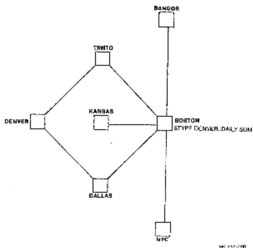
Figure 4-10: Example of the NFT TYPE Command
