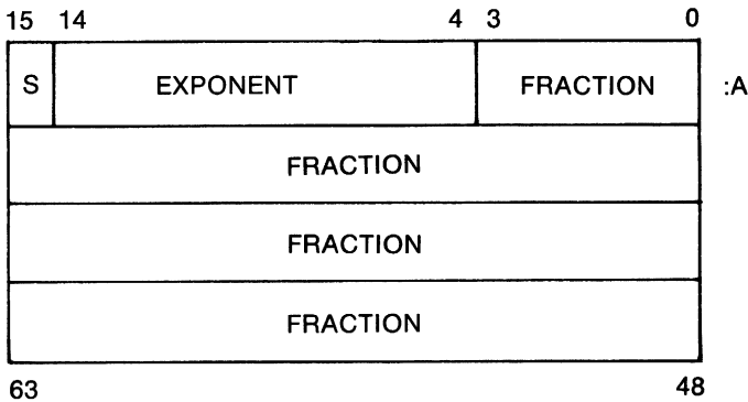
Figure 5-4: G_Floating-Point Double-Precision Representation
