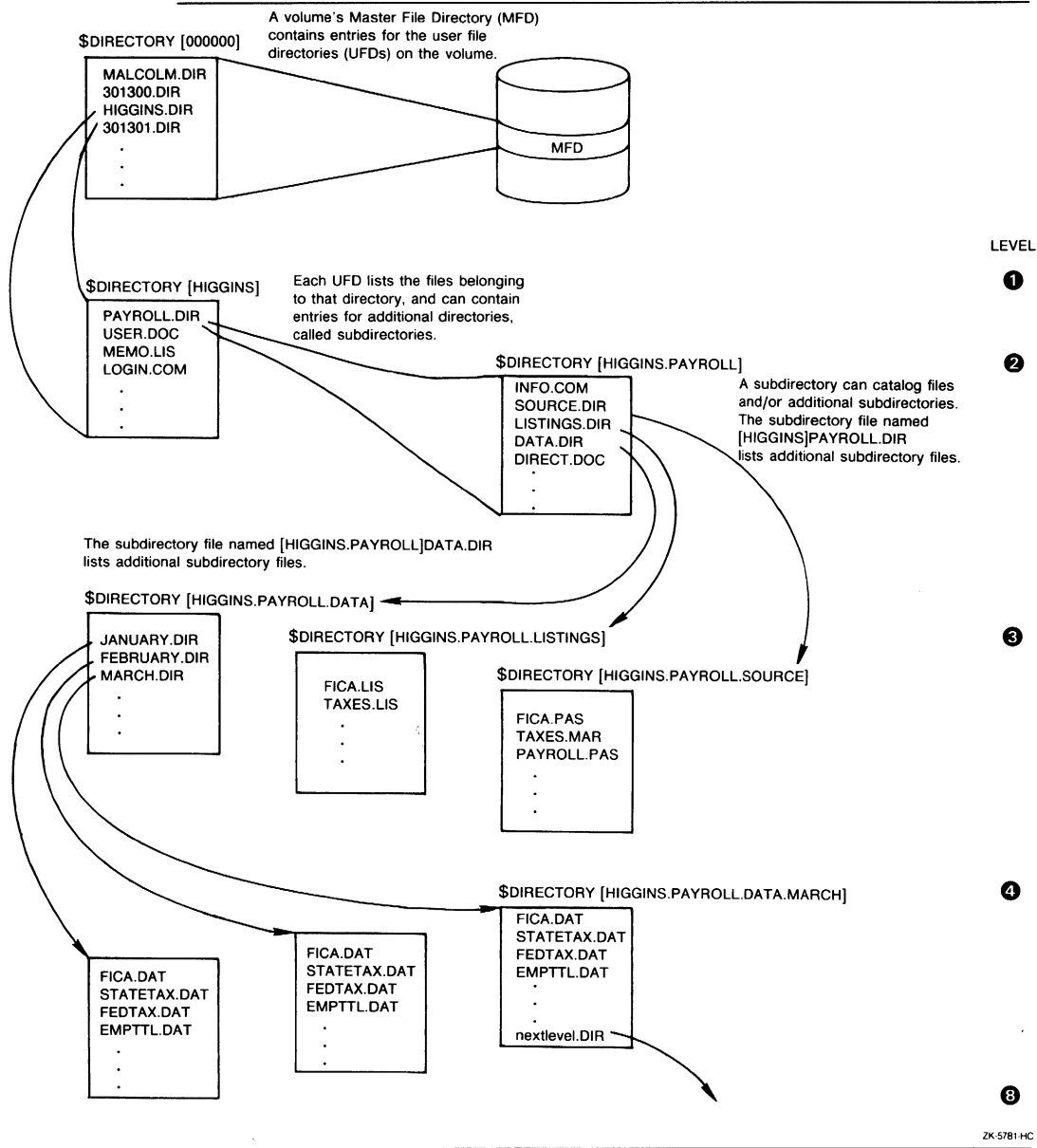
Figure 2-2: A Directory Hierarchy
