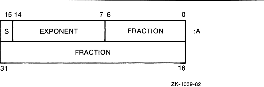
Figure 5-2: Single-Precision Floating-Point Data Representation
