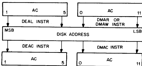
Figure 7-10 Address Words
