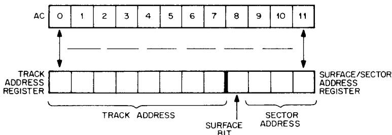
Figure 7-7 Address Word (Read)
