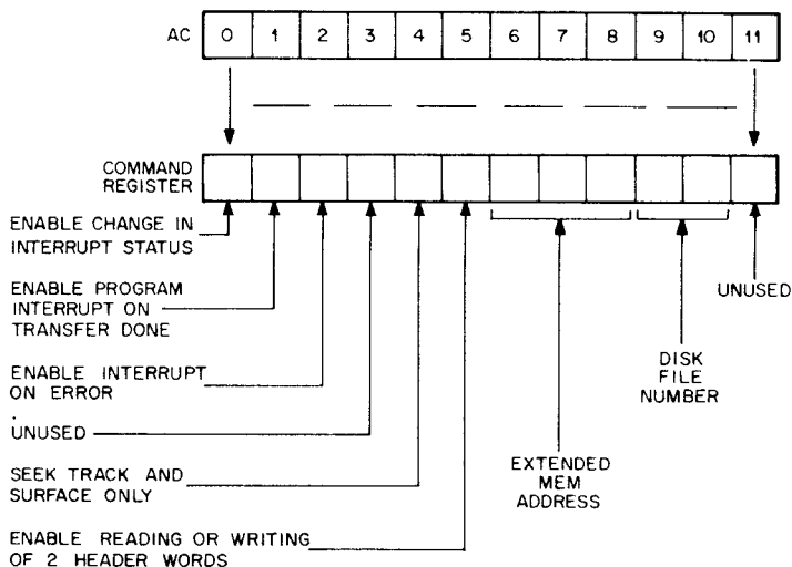
Figure 7-6 Command Word
