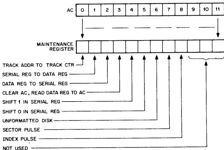
Figure 7-9 Maintenance Word
