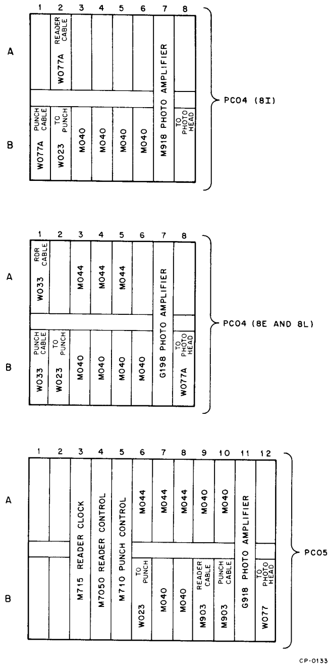
Figure 2-1 PC04/PC05 Module Locations
