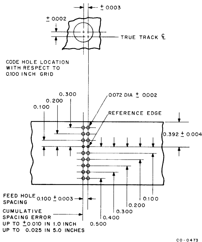
Figure 5-10 Specifications for 1-In. Paper Tape
