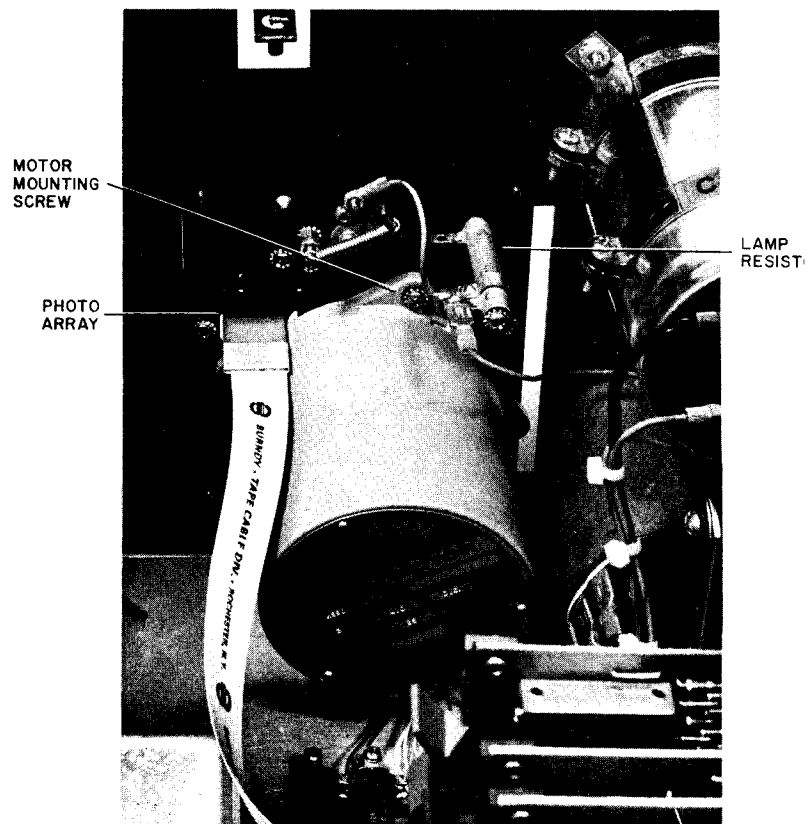
Figure 5-5 PC04/PC05, Rear View
