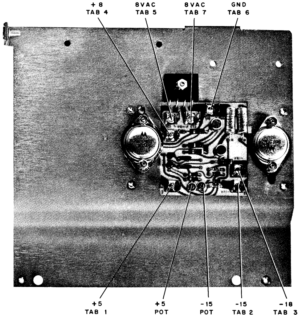
Figure 5-1 Regulator Board
