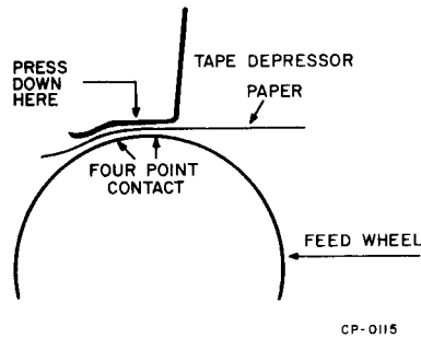
Figure 5-3 Tape Depressor
