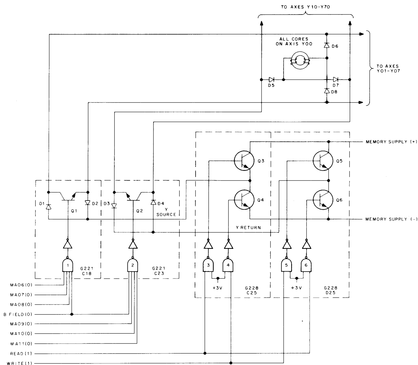
Figure 4-9 Memory Address Selector and Read/Write Current Control
