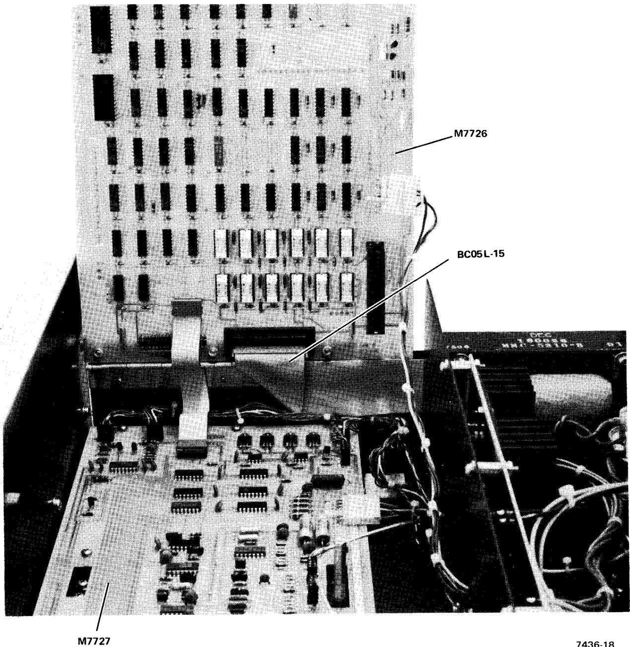
Figure 2-6 Cable Routing, BC05L-15
