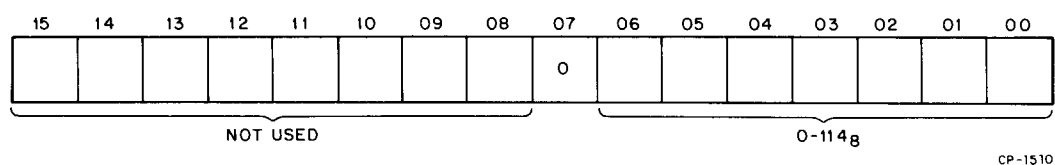
Figure 3-2 RXTA Format (RX11)
