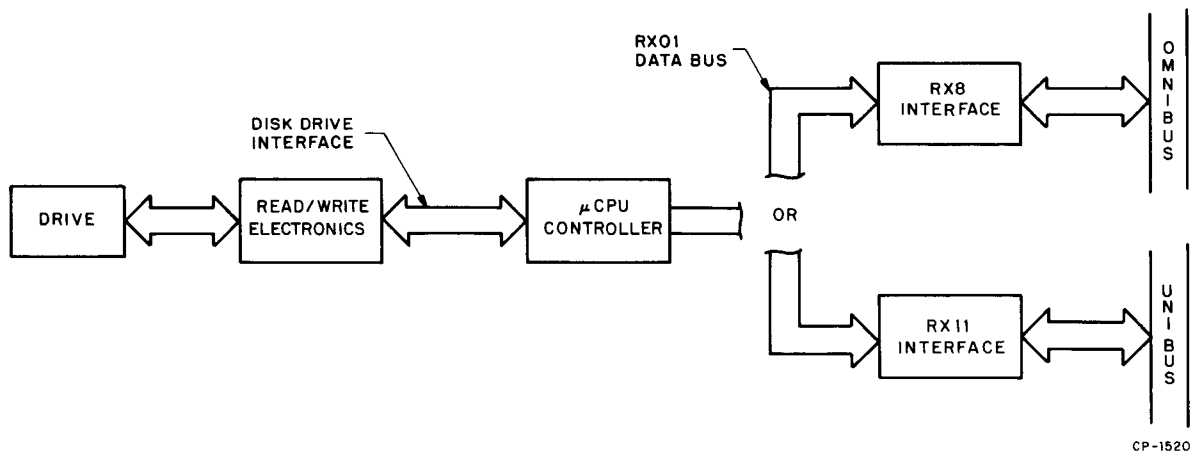
Figure 5-1 Bus Structure
