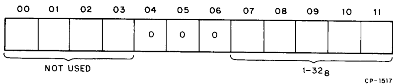
Figure 4-5 RXSA Format (RX8E)
