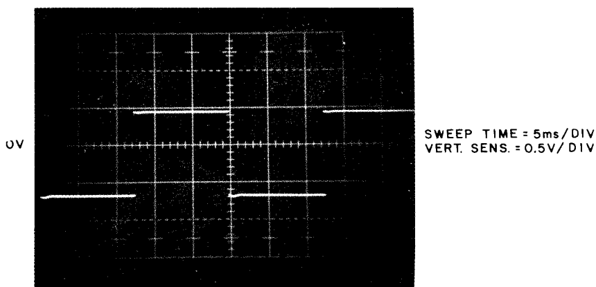
Q9 Collector Voltage
