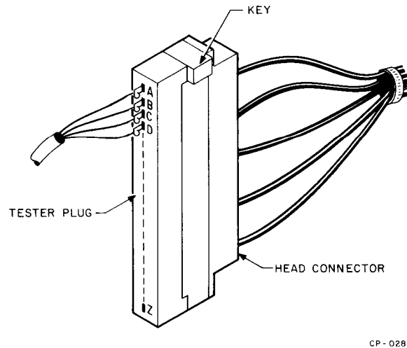
Figure 4-4 Skew Tester to Head Cable Connection
