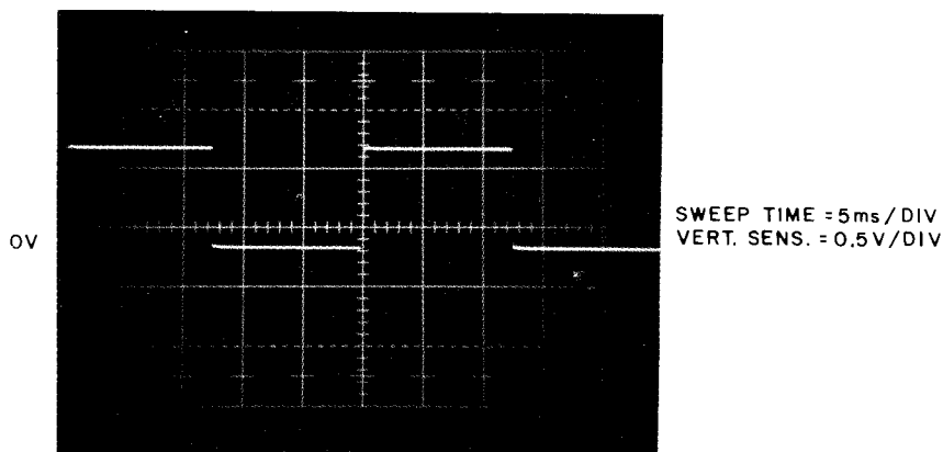
Q9 Emitter to Base Voltage
