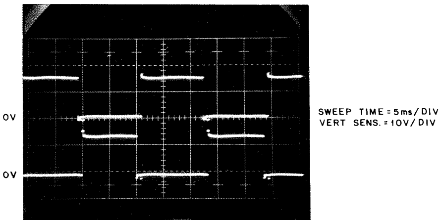
Q5 and Q6 (top), Q7 and Q8 (bottom), Collector Voltage
