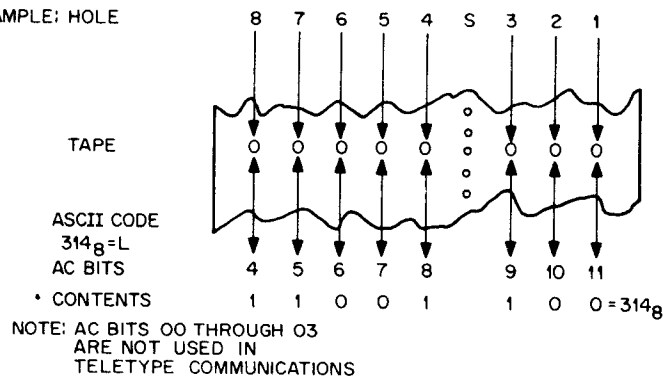
Figure 7-5 Relationship Between Teletype Tape AC Contents and Binary and Octal Number Being Transferred
