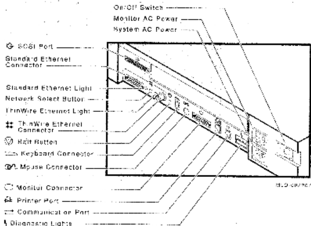
Figure 2-3 System Unit Parts and Connectors
