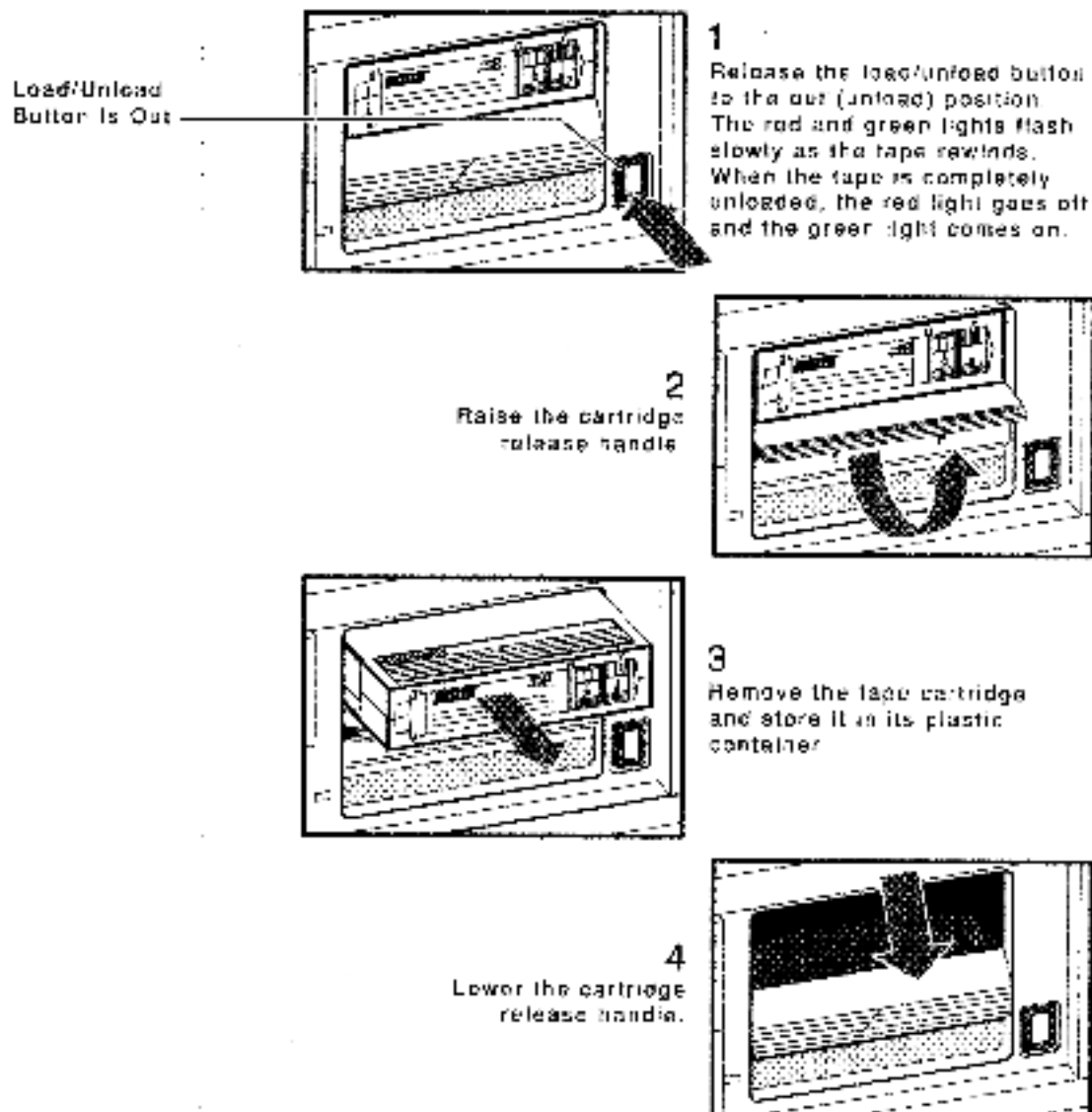
Figure 12-18 Removing a Tape Cartridge from the TK50Z
