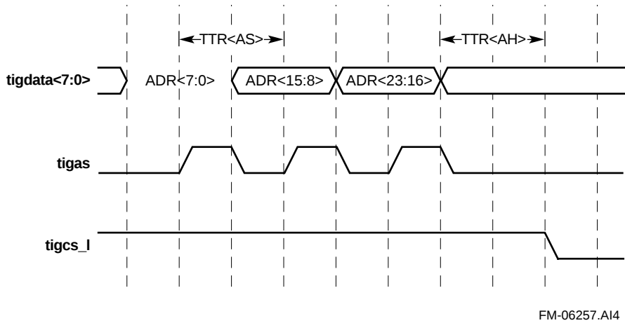
Figure 6–8 TIG Address Timing Parameters
