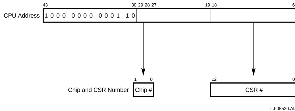
Figure 10–5 CSR Space Address Translation
