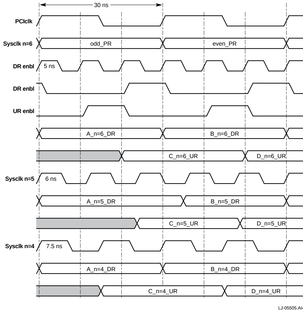
Figure 8–3 PCI Clock to System Clock Transitions
