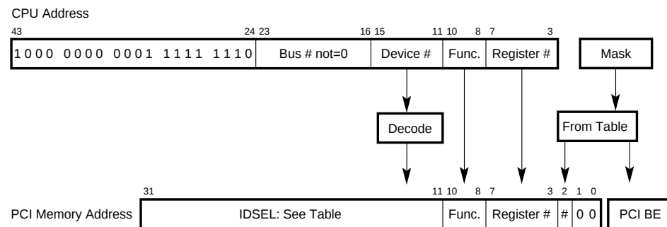
Figure 10–3 Converting Linear Configuration Address to Type 0 PCI Configuration Cycle
