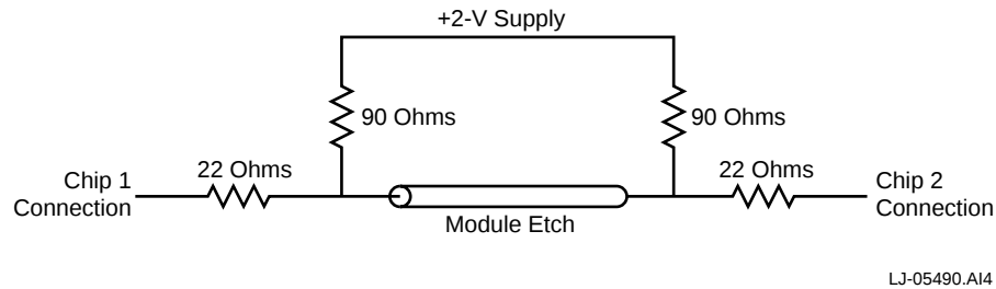
Figure 4–1 Open-Drain Termination Scheme
