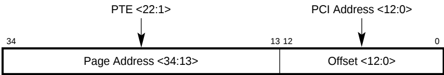
Figure 10–8 Generating System Address from Scatter-Gather PTE
