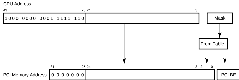
Figure 10–2 Linear I/O Address Translation
