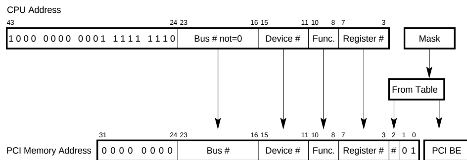
Figure 10–4 Converting Linear Configuration Address to Type 1 PCI Configuration Cycle
