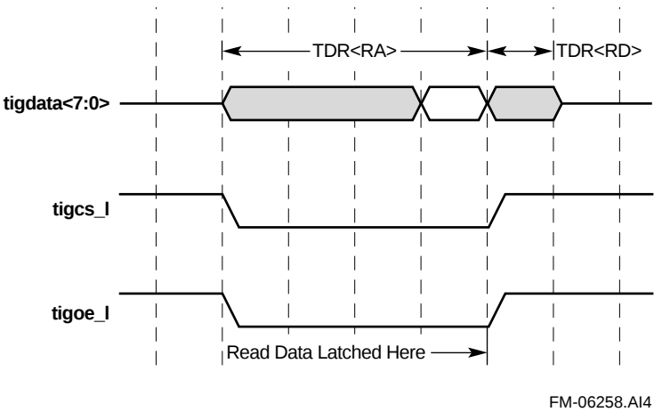
Figure 6–9 TIG Read Timing Parameters
