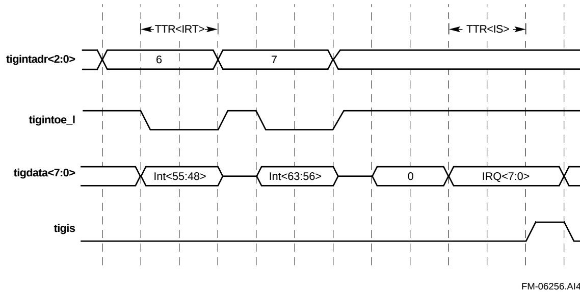
Figure 6–7 Interrupt Timing Parameters
