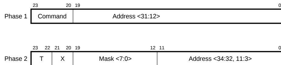
Figure 6–3 Format of 2-Cycle Commands
