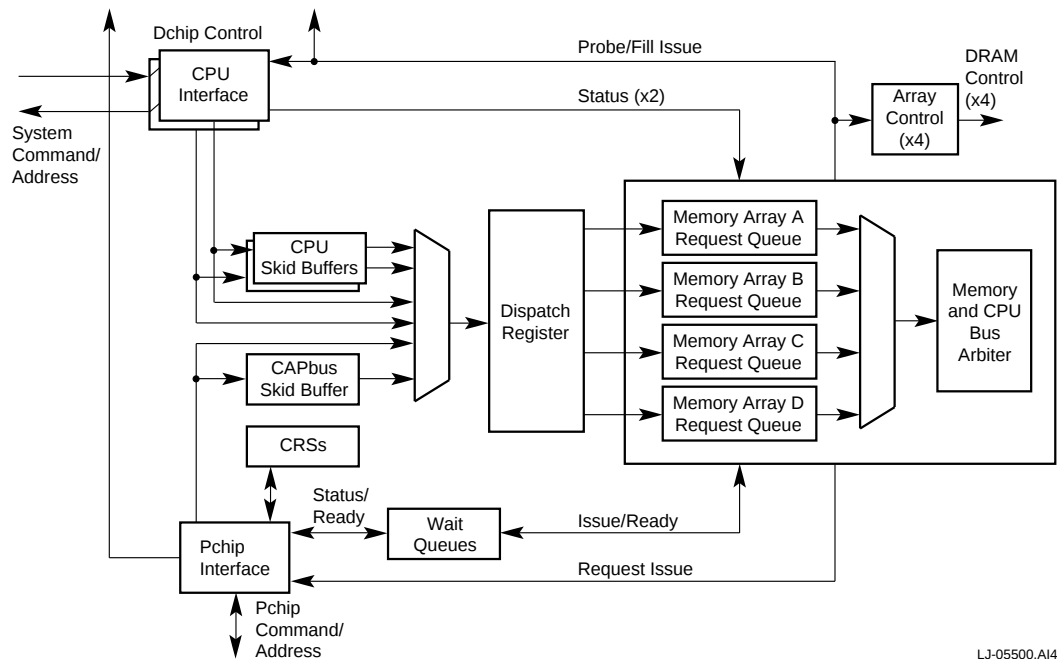
Figure 6–1 Cchip Block Diagram
