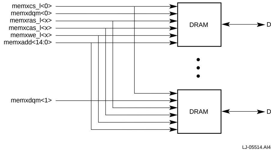
Figure 9–1 Nonsplit Array Block Diagram
