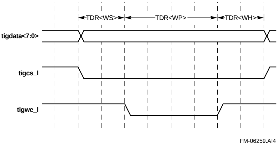
Figure 6–10 TIG Write Timing Parameters
