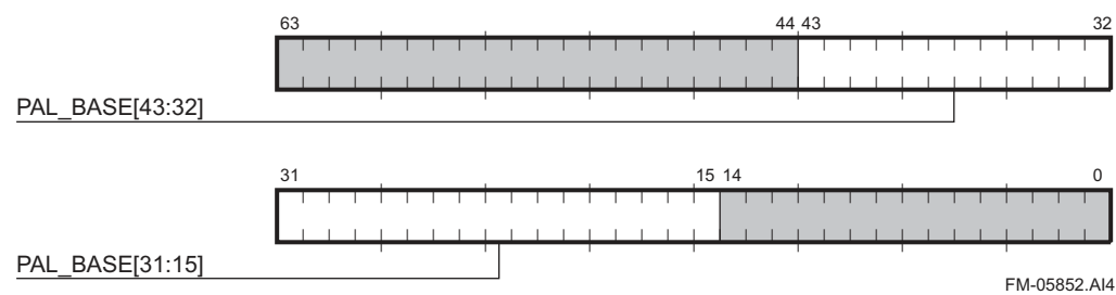
Figure 5–20 PAL Base Register
