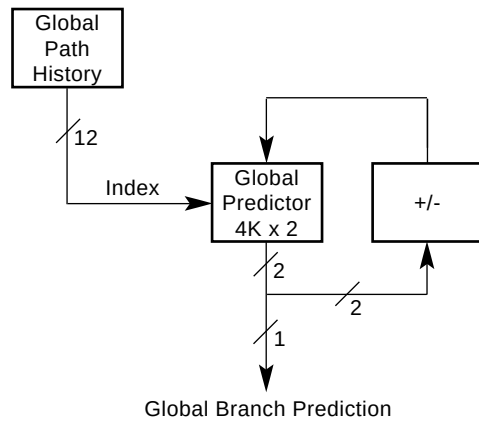
Figure 2–4 Global Predictor
