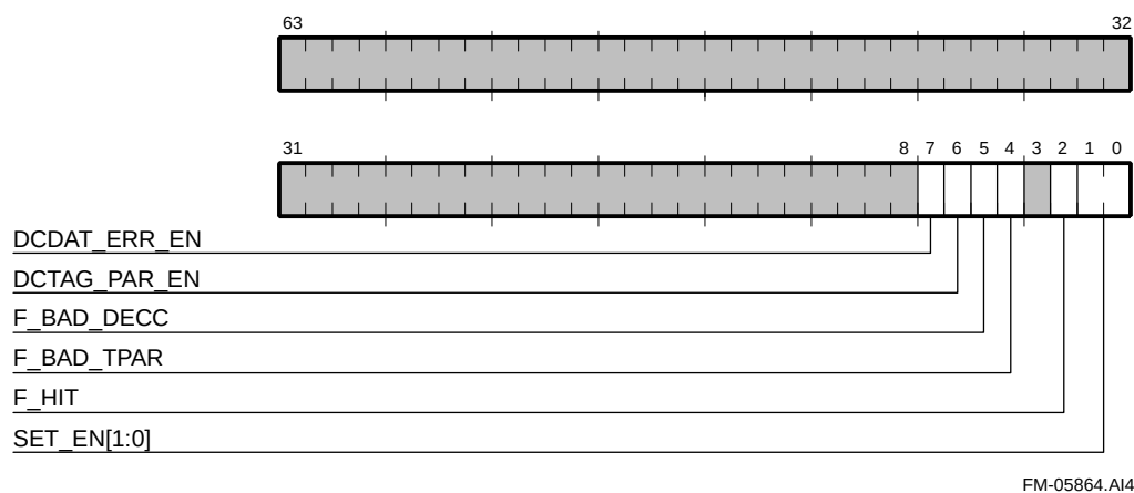
Figure 5–32 Dcache Control Register
