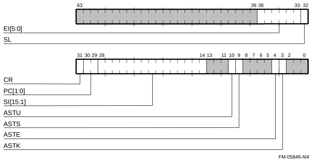
Figure 5–17 Interrupt Summary Register
