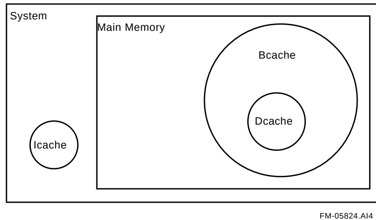
Figure 4–3 Cache Subset Hierarchy
