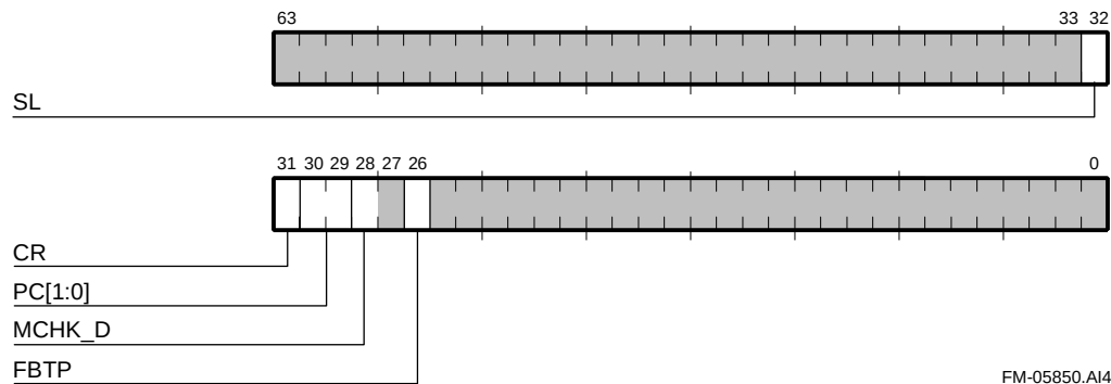
Figure 5–18 Hardware Interrupt Clear Register
