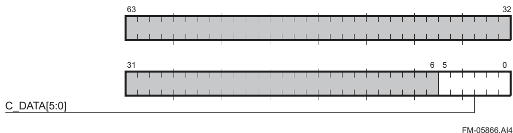
Figure 5–34 Cbox Data Register
