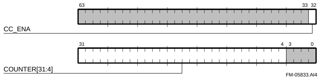
Figure 5–2 Cycle Counter Control Register
