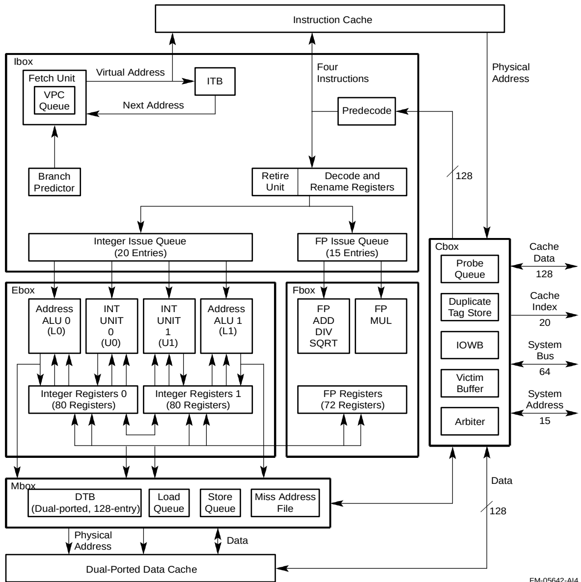
Figure 2–1 21264/EV6 Block Diagram
