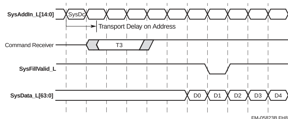
Figure 4–6 SysFillValid_L Timing
