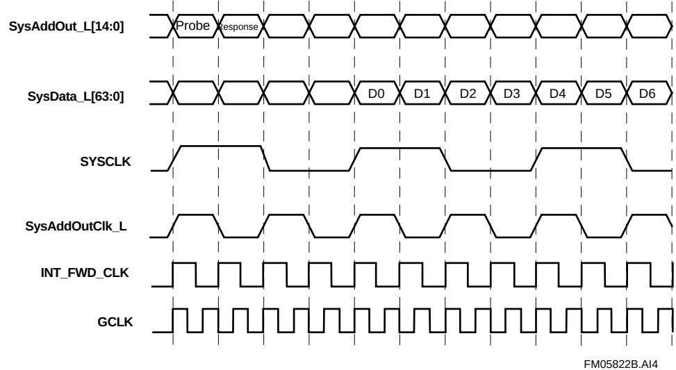
Figure 4–5 Fast Transfer Timing Example
