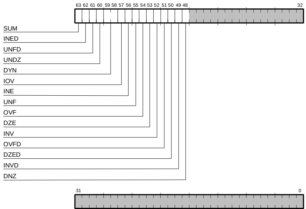
Figure 2–11 Floating-Point Control Register
