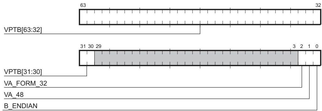
Figure 5–4 Virtual Address Control Register
