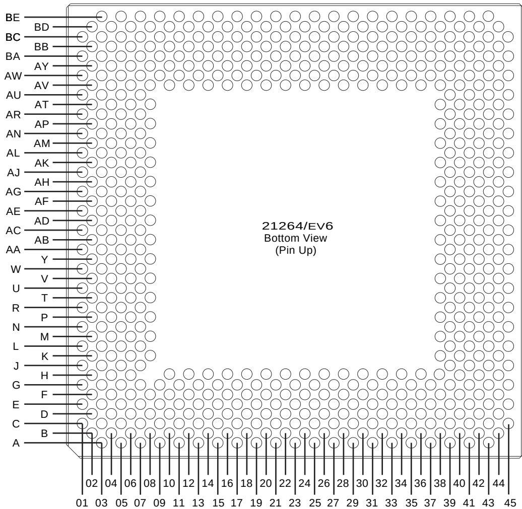
Figure 3–4 21264/EV6 Bottom View (Pin Up)
