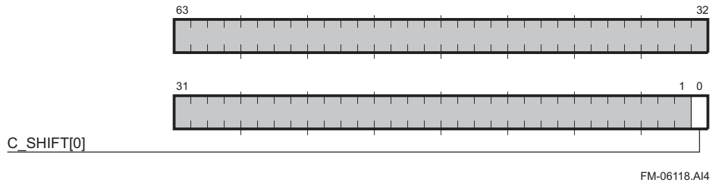
Figure 5–35 Cbox Shift Register
