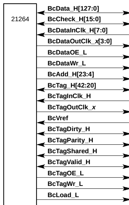
Figure 4–2 21264/EV6 Bcache Interface Signals
