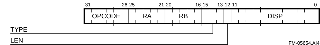
Figure 6–2 HW_ST Instruction Format
