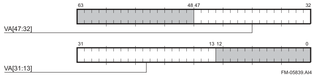
Figure 5–8 ITB Tag Array Write Register
