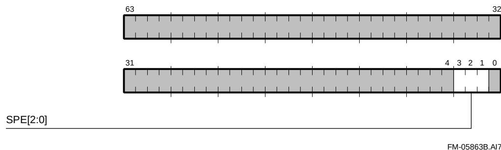
Figure 5–31 Mbox Control Register
