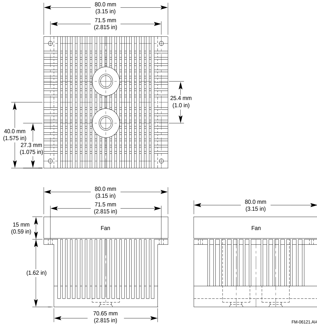
Figure 10–3 Type 3 Heat Sink
