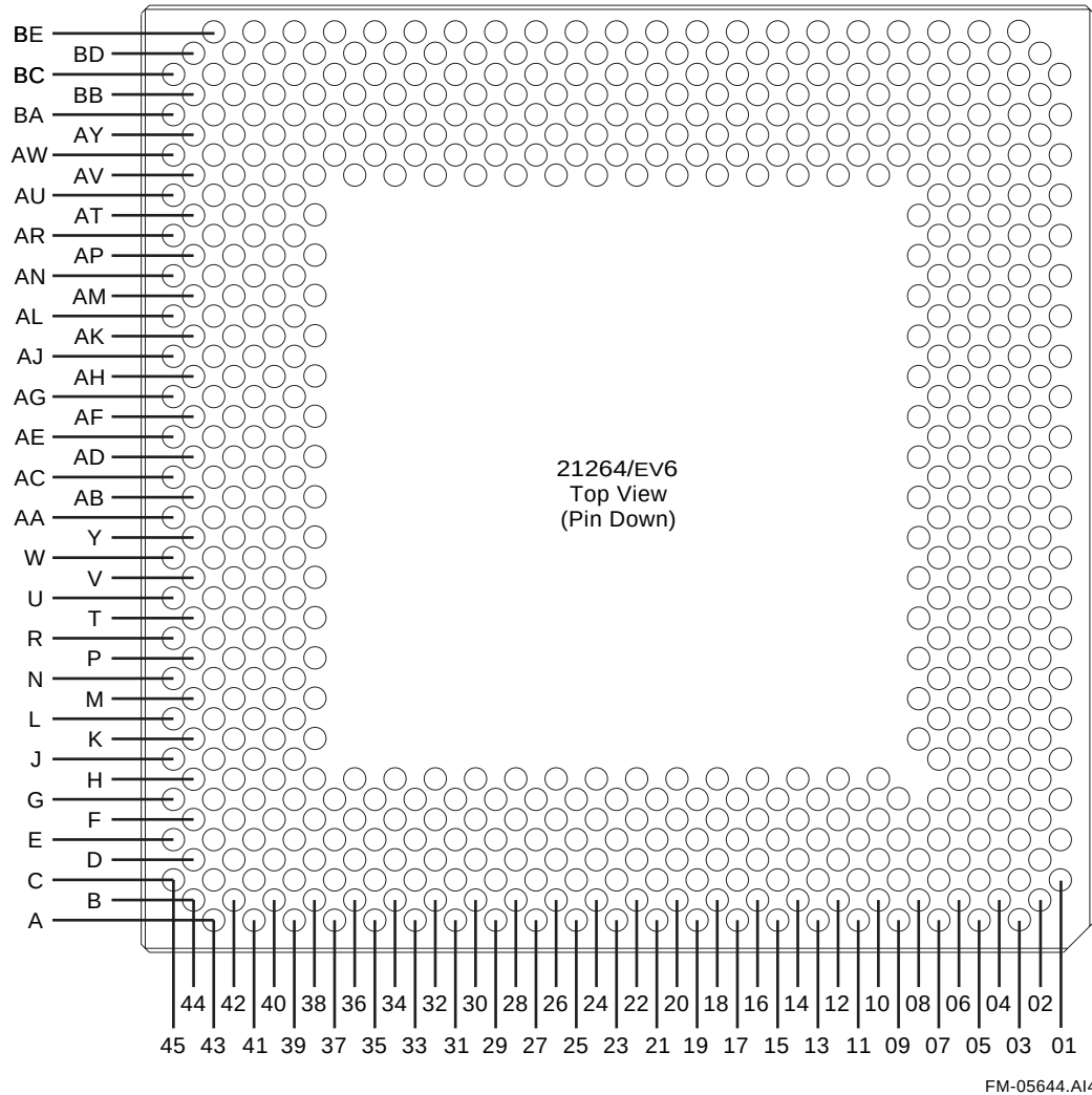
Figure 3–3 21264/EV6 Top View (Pin Down)
