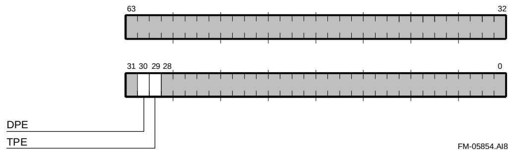
Figure 5–22 Ibox Status Register
