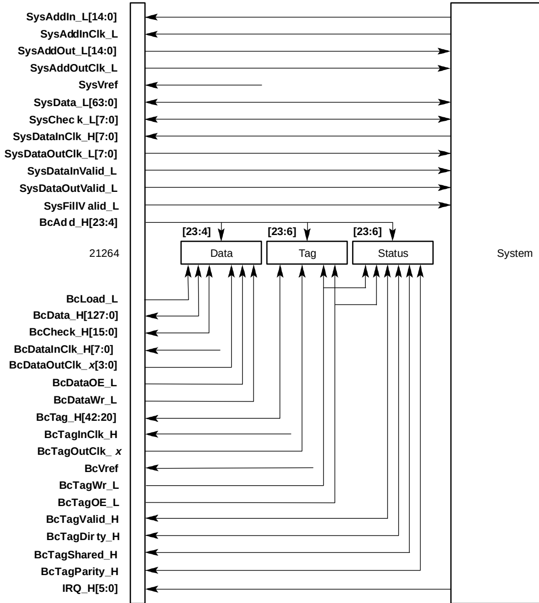
Figure 4–1 21264/EV6 System and Bcache Interfaces
