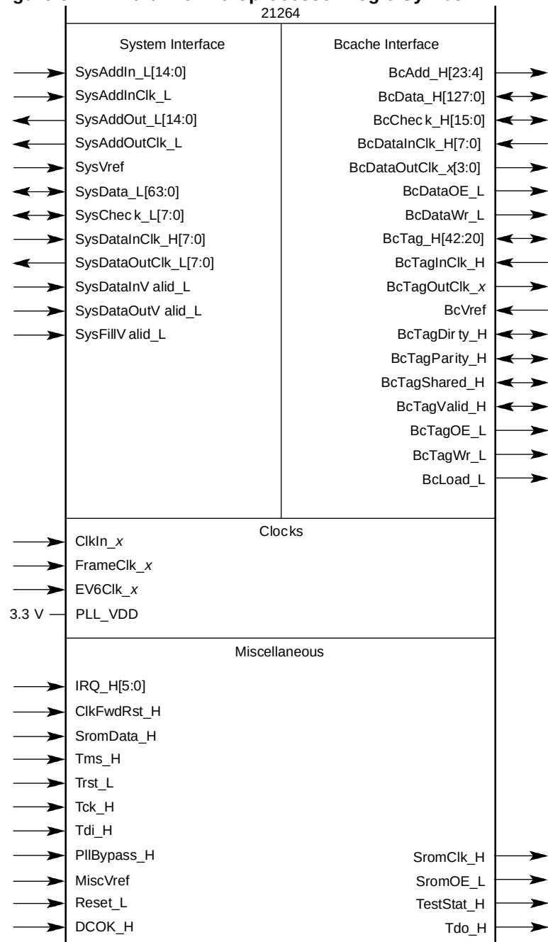
Figure 3–1 21264/EV6 Microprocessor Logic Symbol
