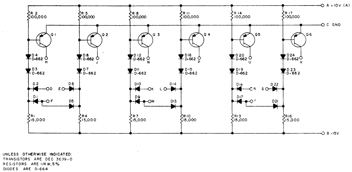
Figure 5-9 Diode Gate, R123
