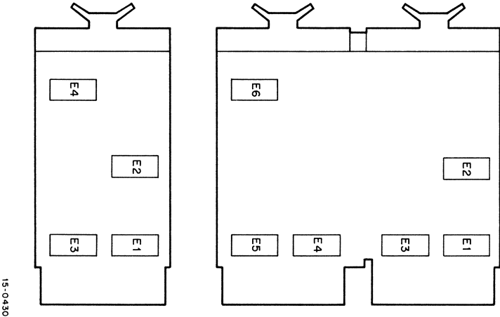
Figure 5-1 IC Location
