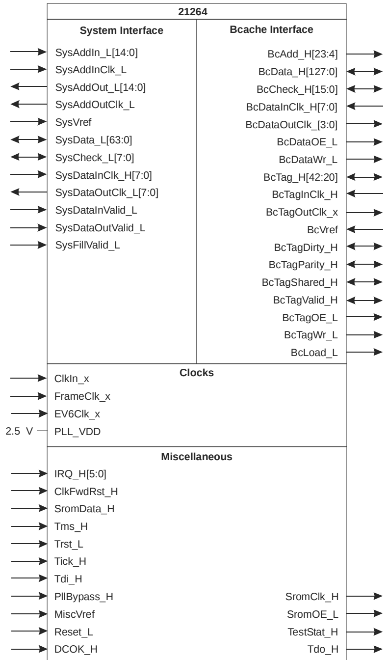
Figure 3–1 21264/EV68A Microprocessor Logic Symbol
