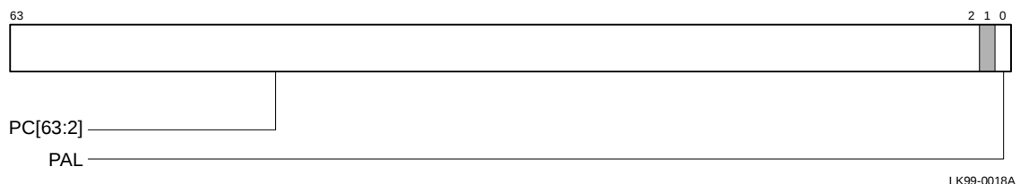
Figure 5–12 Exception Address Register
