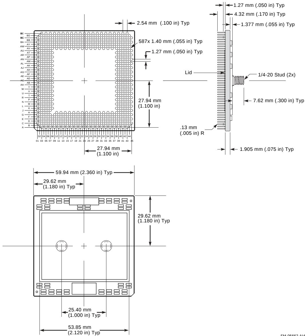
Figure 3–2 Package Dimensions
