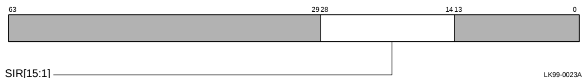
Figure 5–17 Software Interrupt Request Register
