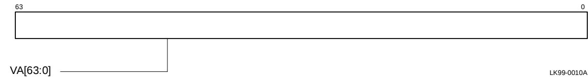
Figure 5–3 Virtual Address Register
