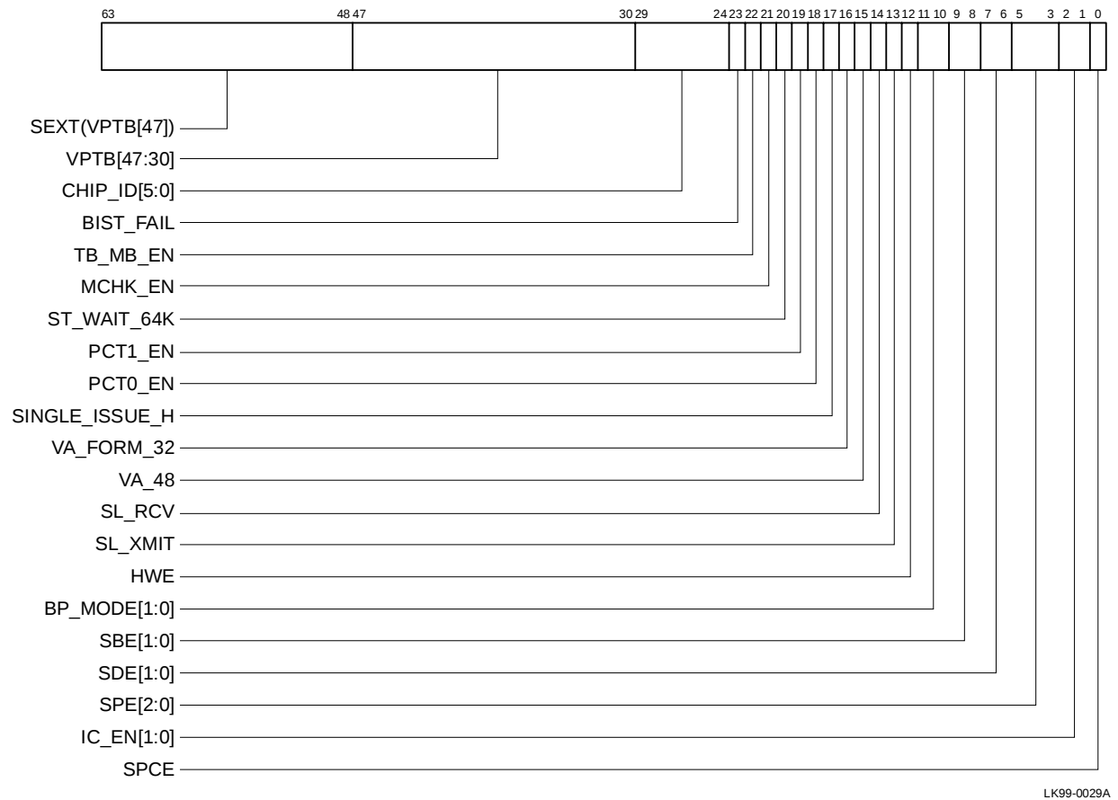
Figure 5–22 Ibox Control Register
