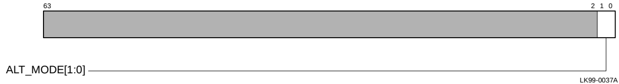
Figure 5–28 DTB Alternate Processor Mode Register
