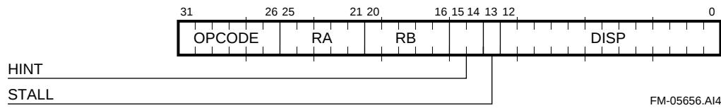
Figure 6–3 HW_RET Instruction Format
