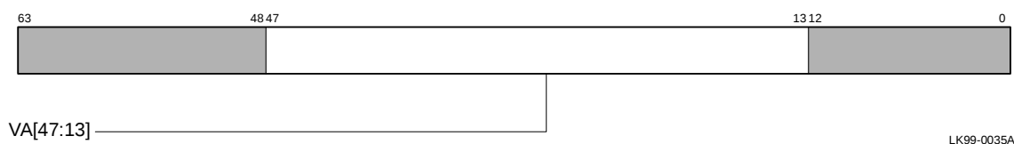
Figure 5–26 DTB Tag Array Write Registers 0 and 1
