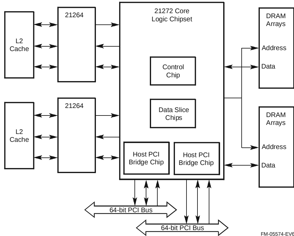
Figure 2–13 Typical Multiprocessor Configuration
