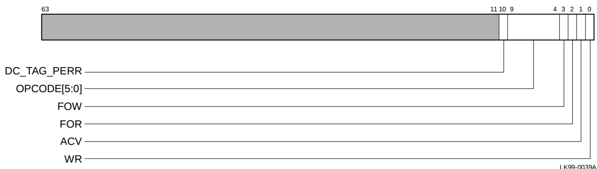
Figure 5–31 Memory Management Status Register
