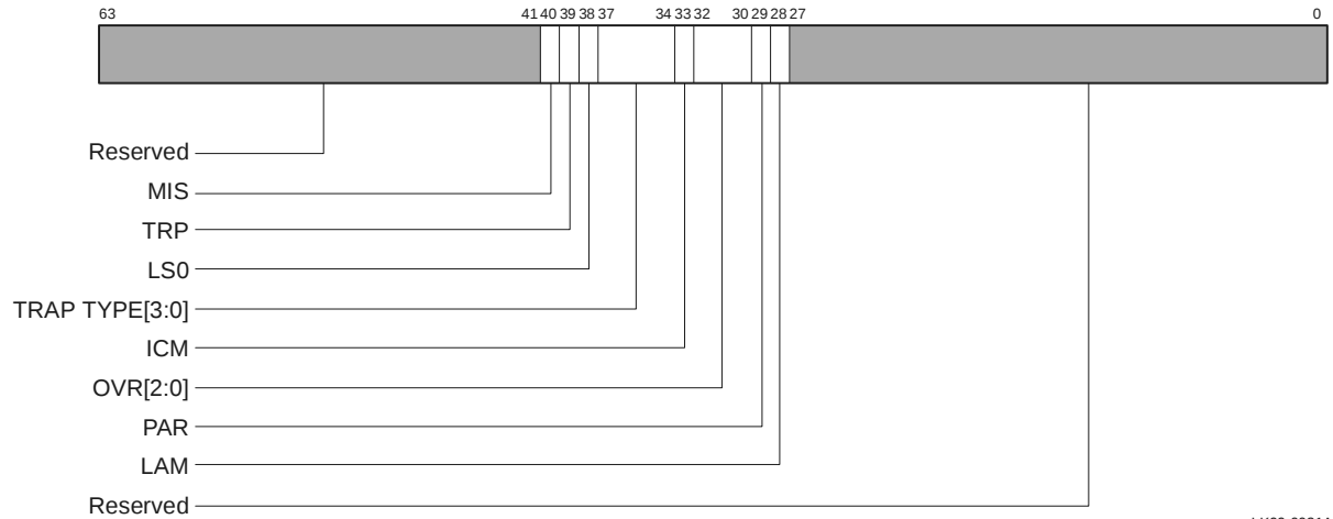
Figure 5–23 Ibox Status Register
