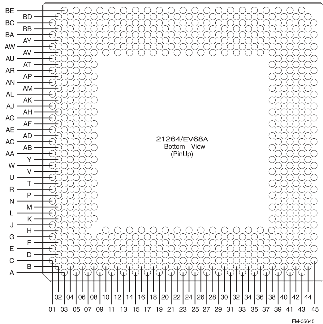
Figure 3–4 21264/EV68A Bottom View (Pin Up)
