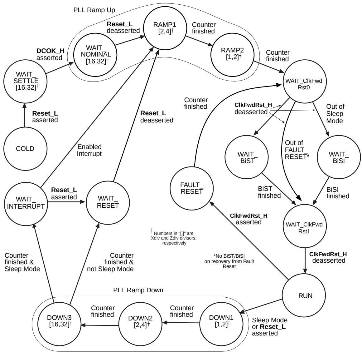
Figure 7–5 21264/EV68A Reset State Machine State Diagram
