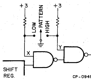
Figure 5-12 Typical Front Panel Switch Arrangement
