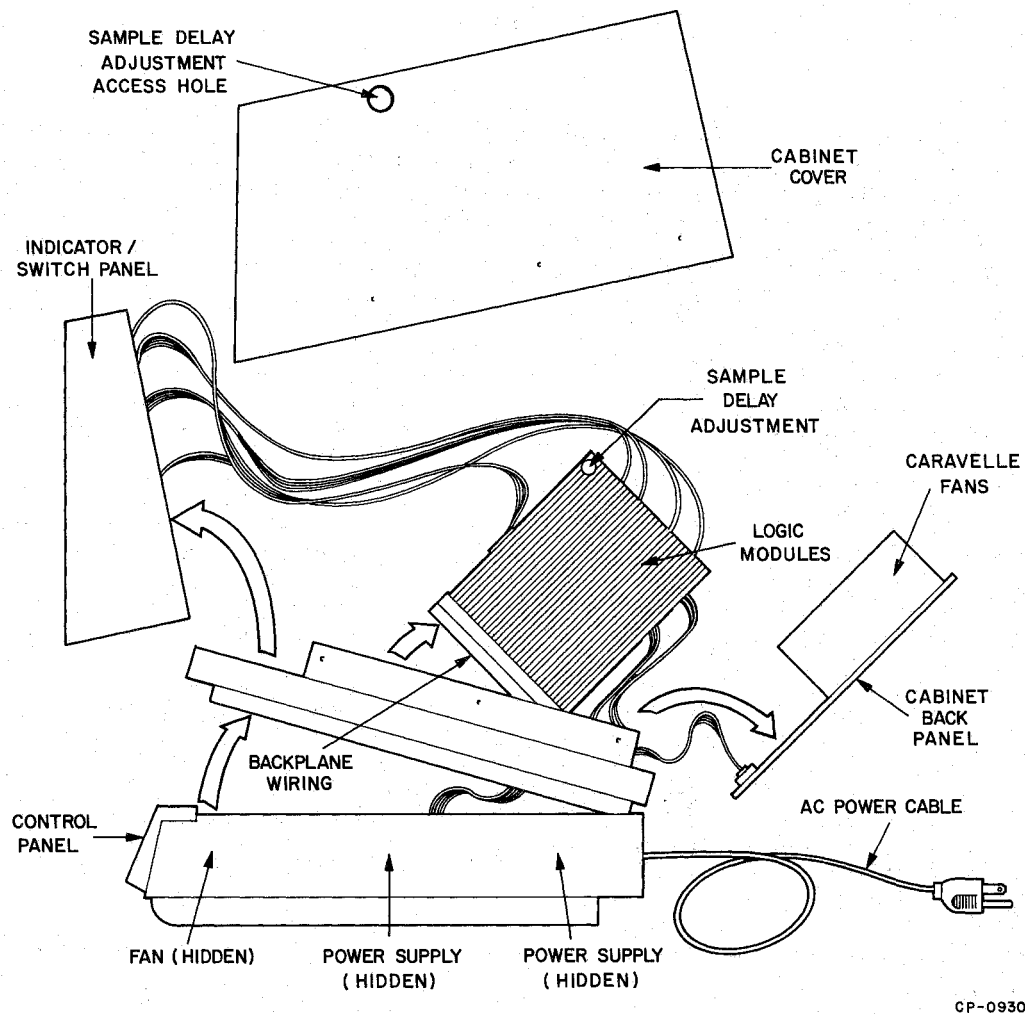
Figure 1-3 2340 Access Schematic
