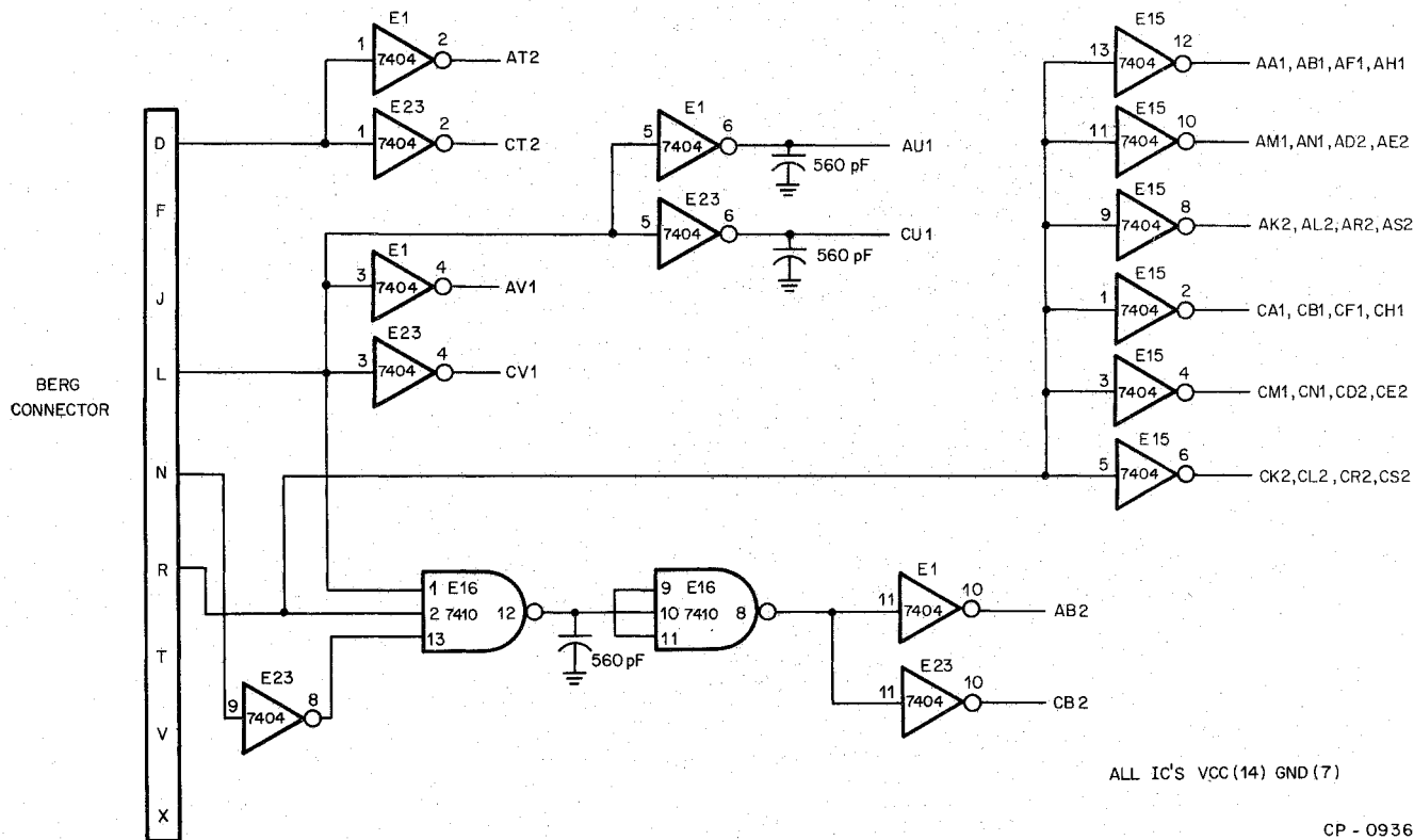
Figure 3-2 M249 Adapter
