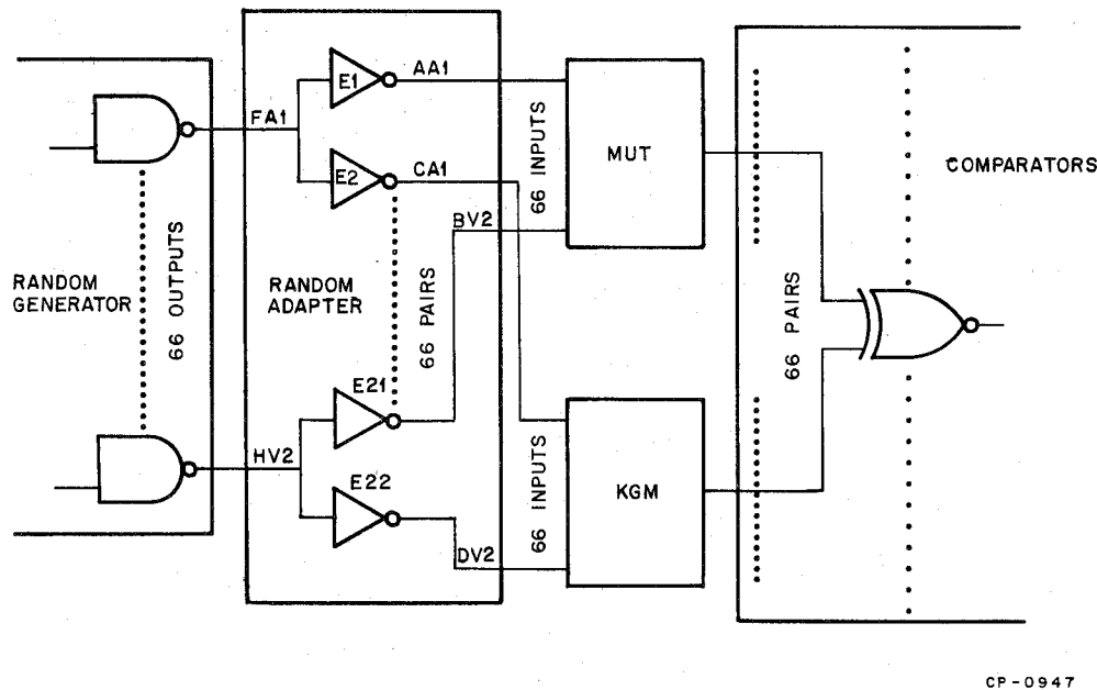
Figure 5-10 Random Adapter Block Diagram
