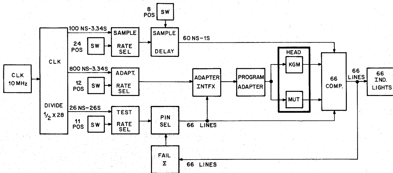
Figure 5-2 2340 Program Mode Functional Block Diagram
