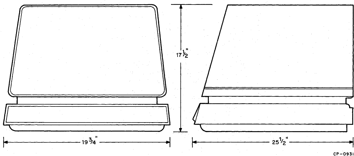
Figure 1-4 2340 Overall Dimensions
