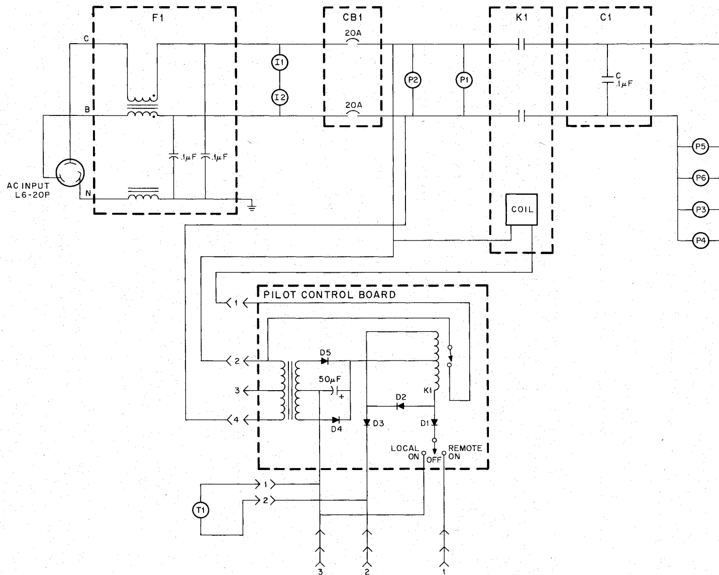
Figure 4-2 861-B Simplified Circuit Schematic Diagram
