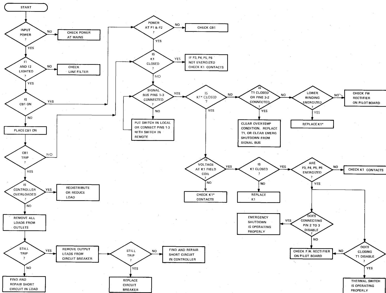
Figure 5-2 Troubleshooting Flow Diagram
