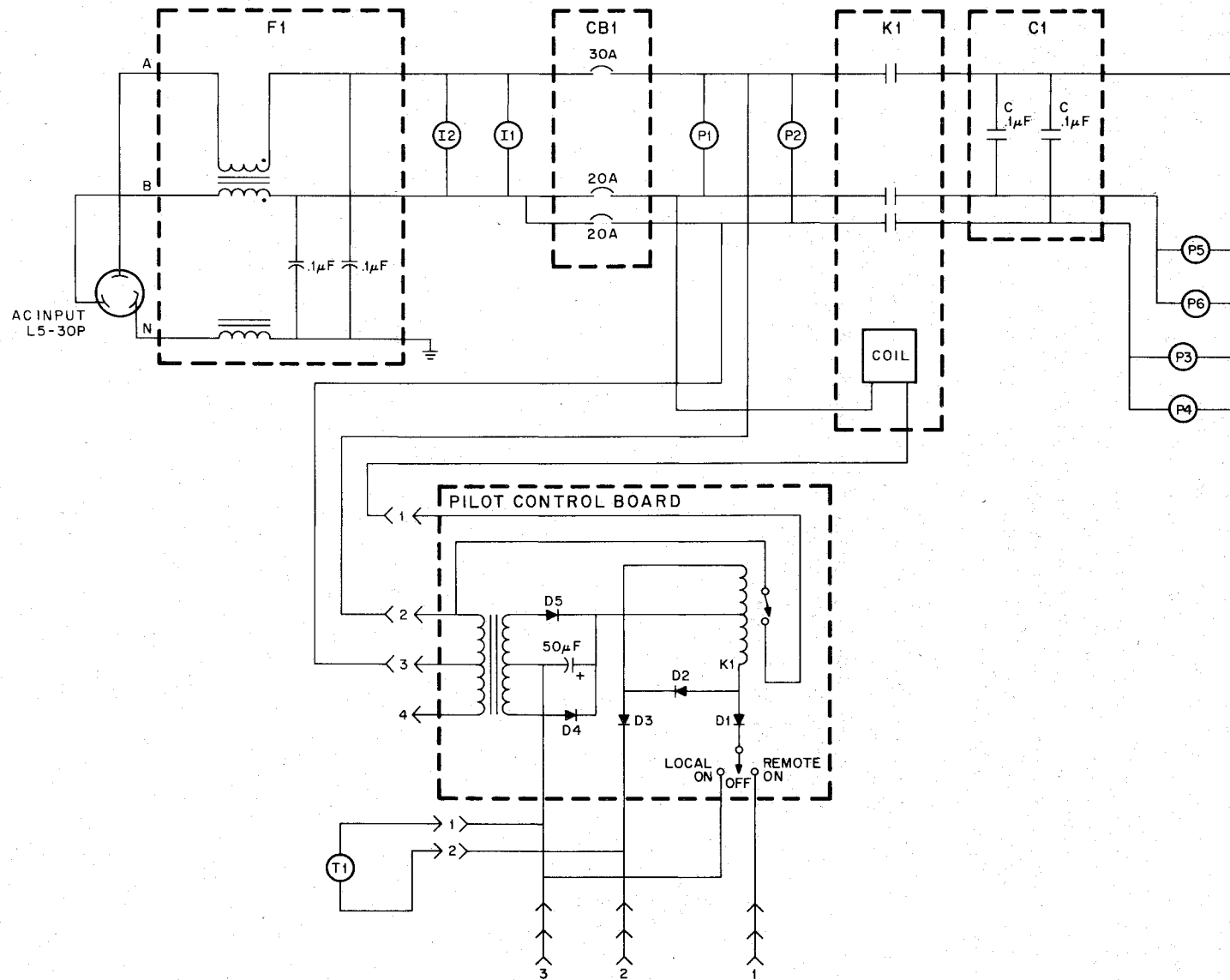
Figure 4-3 861-C Simplified Circuit Schematic Diagram
