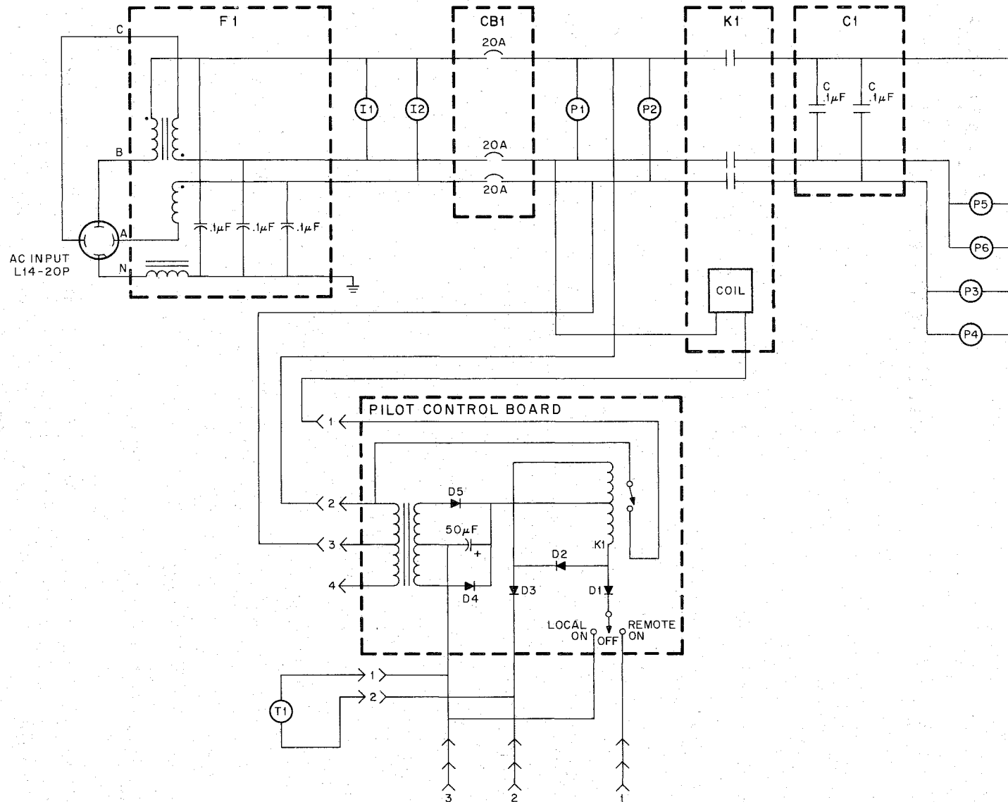
Figure 4-1 861-A Simplified Circuit Schematic Diagram
