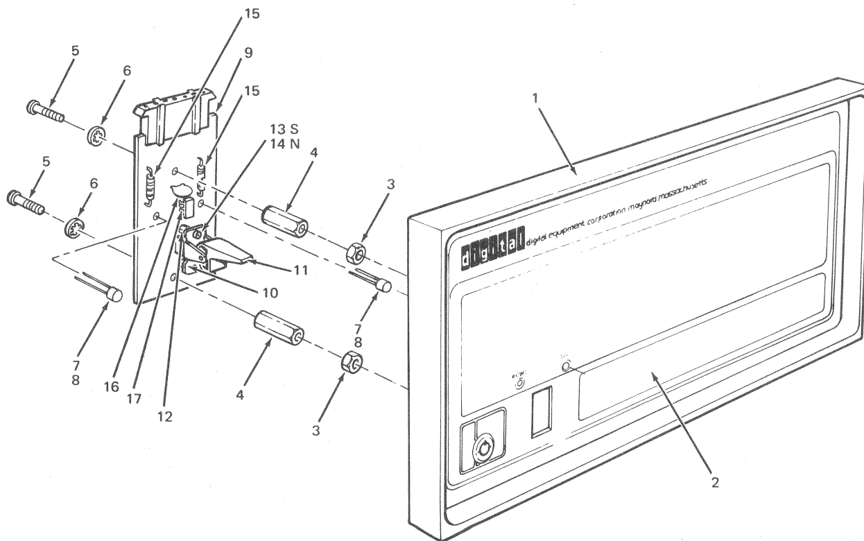
Figure 3. Console Assembly (Operator)
