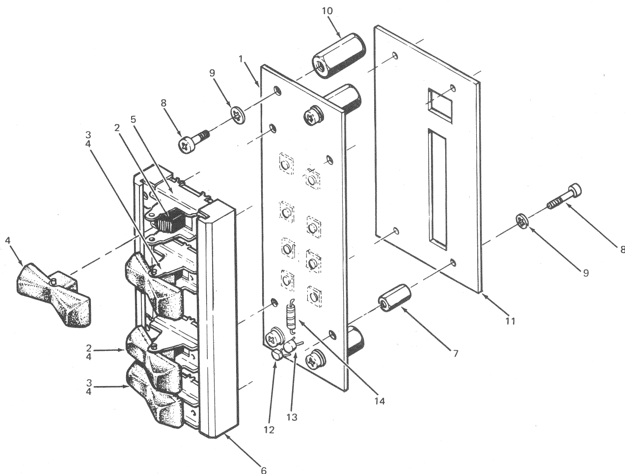
Figure 5. PCO Switch Assembly
