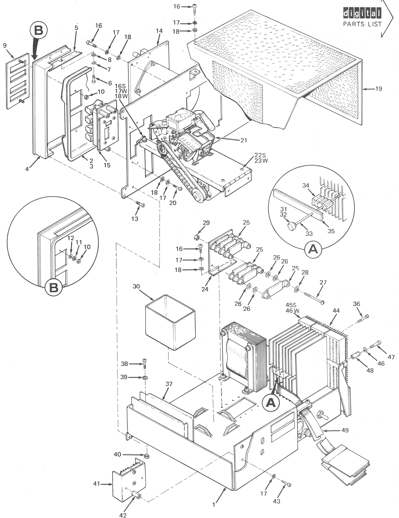
Figure 1. Model PC05 Paper Tape Reader/Punch Assembly
