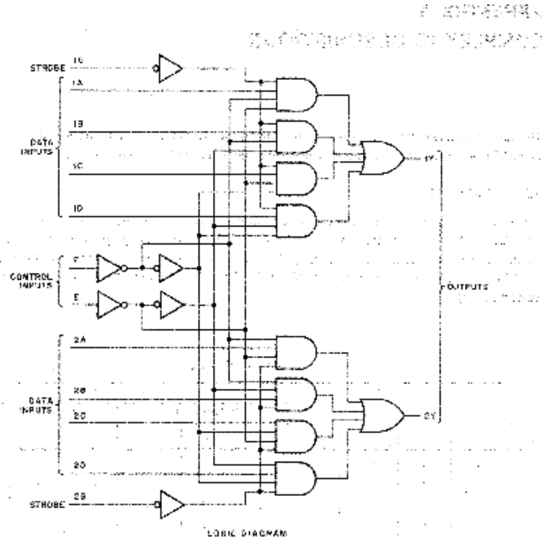
Figure A-3 74153 Dual 4-Line-To-1-Line Data Selector/Multiplexer
