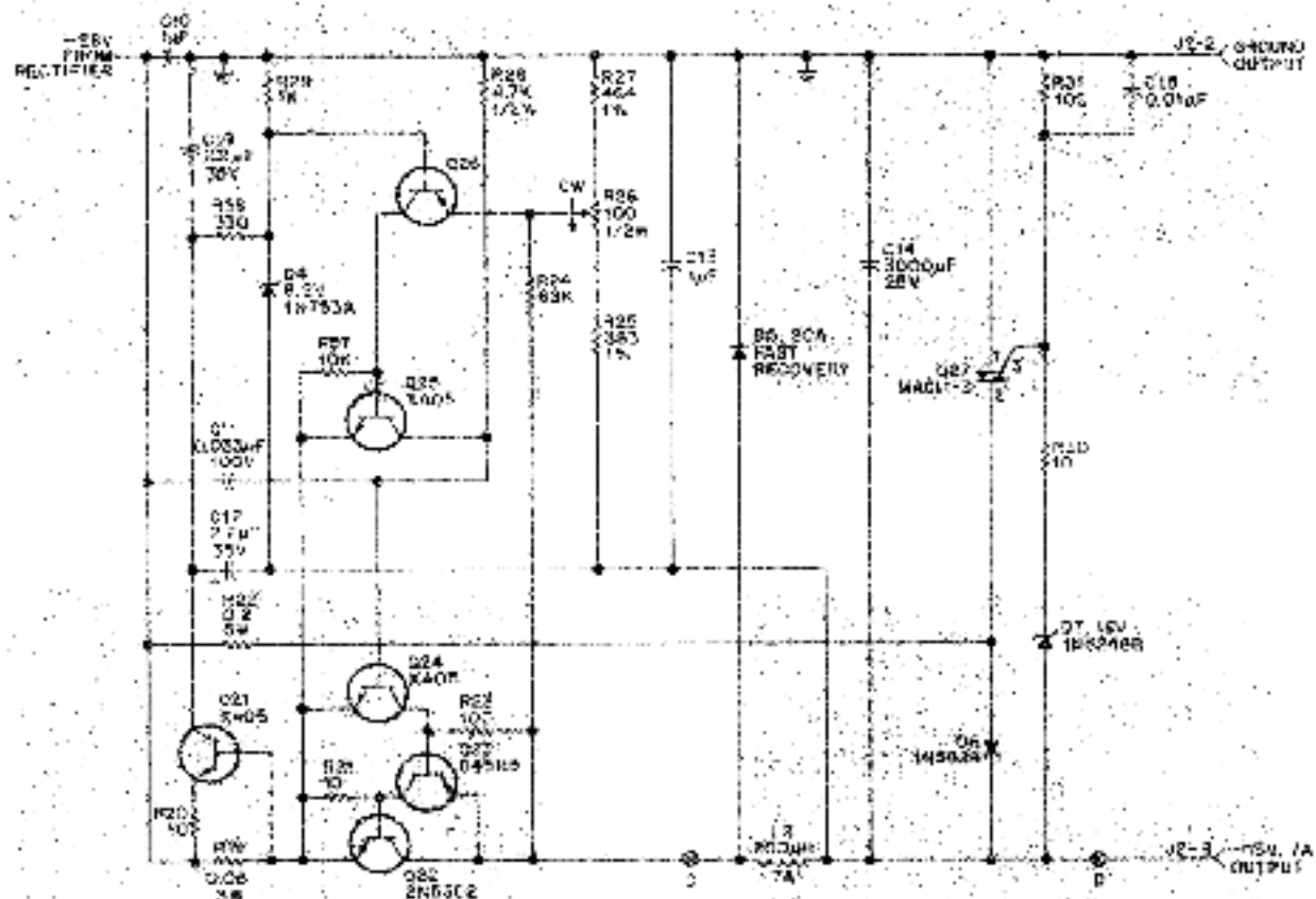
Figure 2-11 -15V Regulator Circuit
