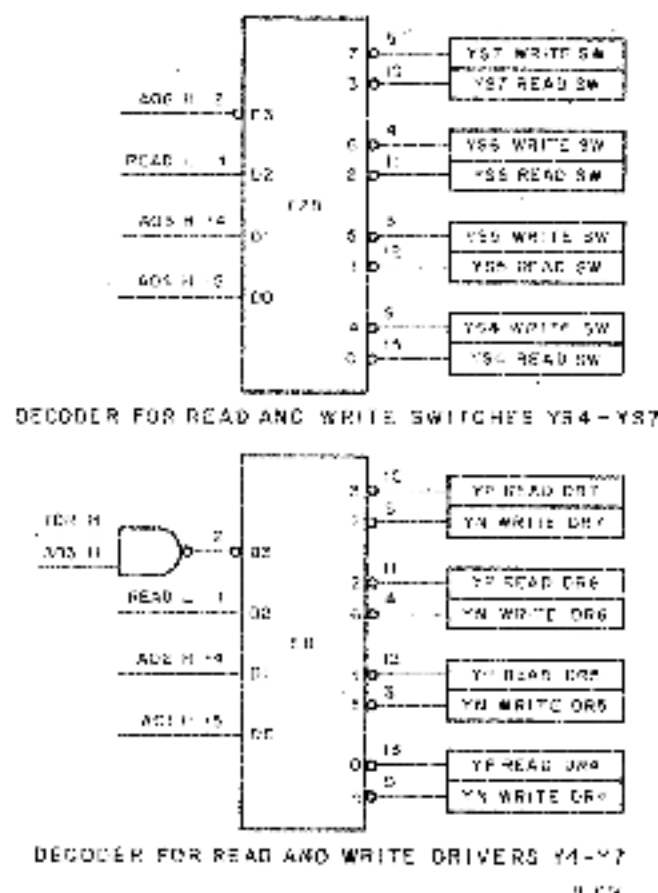
Figure 3-14 Decoding of Read/Write Switches and Drivers Y4-Y7
