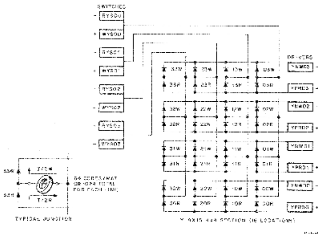
Figure 3-16 Y-Line Selection Slack Diode Matrix
