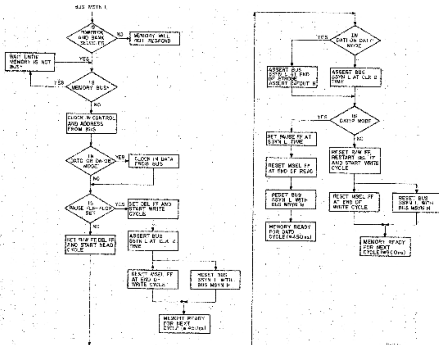
Figure 3-30 Flow Chart for Memory Operation
