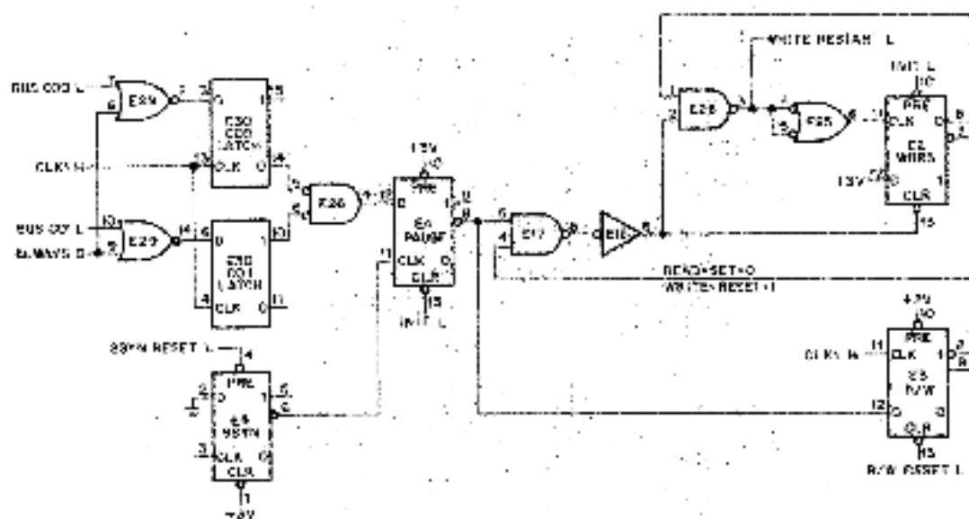
Figure 3-28 Pause/Write Restart Circuit
