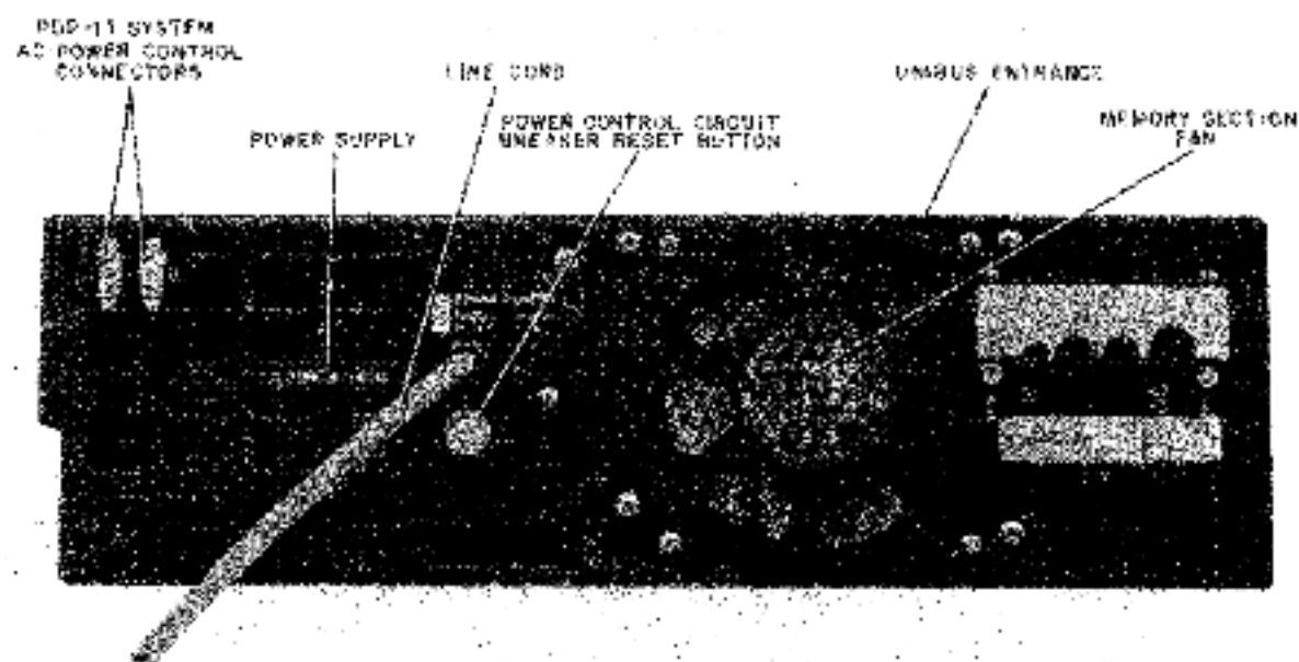
Figure 1-3 Rear View of MB11-L
