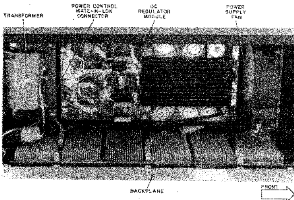
Figure 1-6 Power Supply Section of ME11-L
