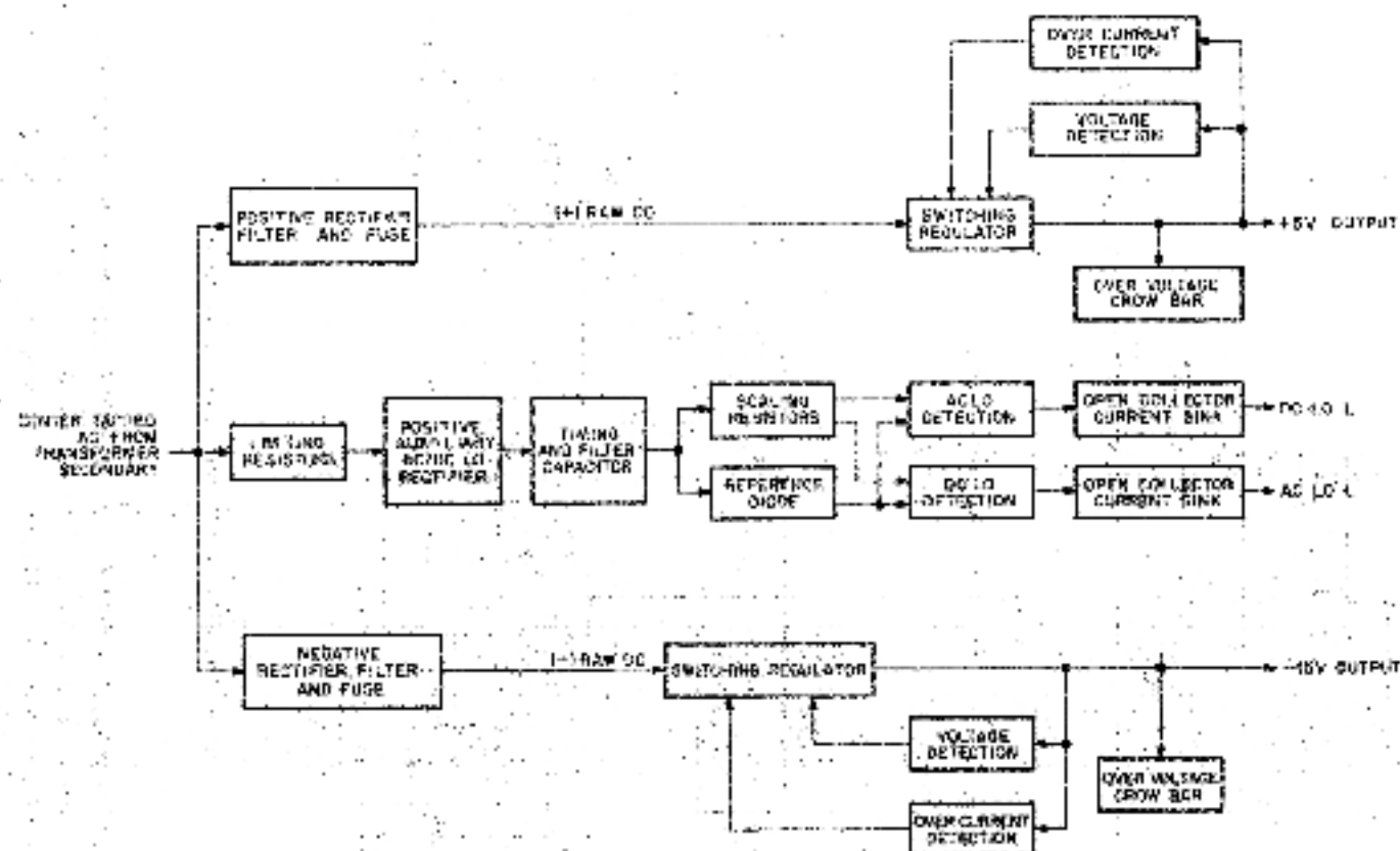
Figure 2-7 DC Regulator Module, Block Diagram
