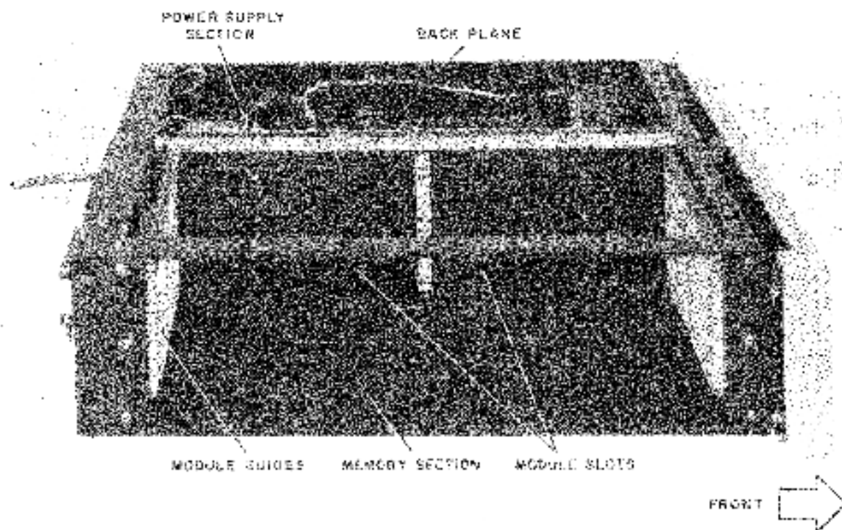
Figure 1-4 MB11-L without Memory Modules
