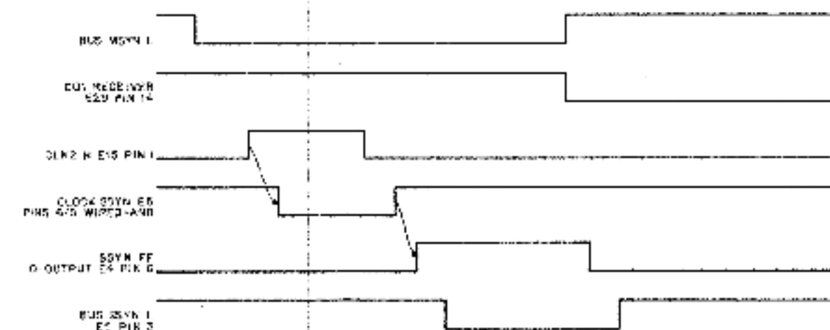
Timing Diagram for SSYN Circuit During DATO and DATOP
