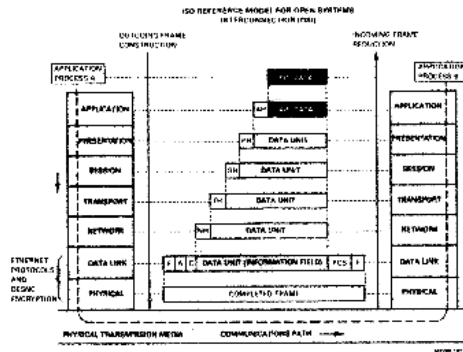
Figure 5-4 ISO Reference Model for Open Systems Interconnection (OSI)
