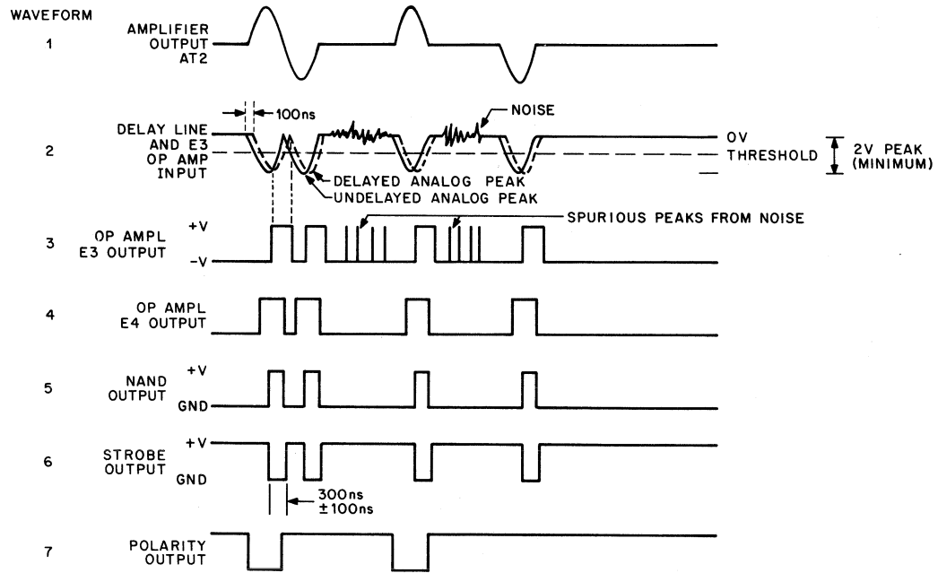
Figure 3-10 G088 Read Amplifier-Peak Detector Waveforms
