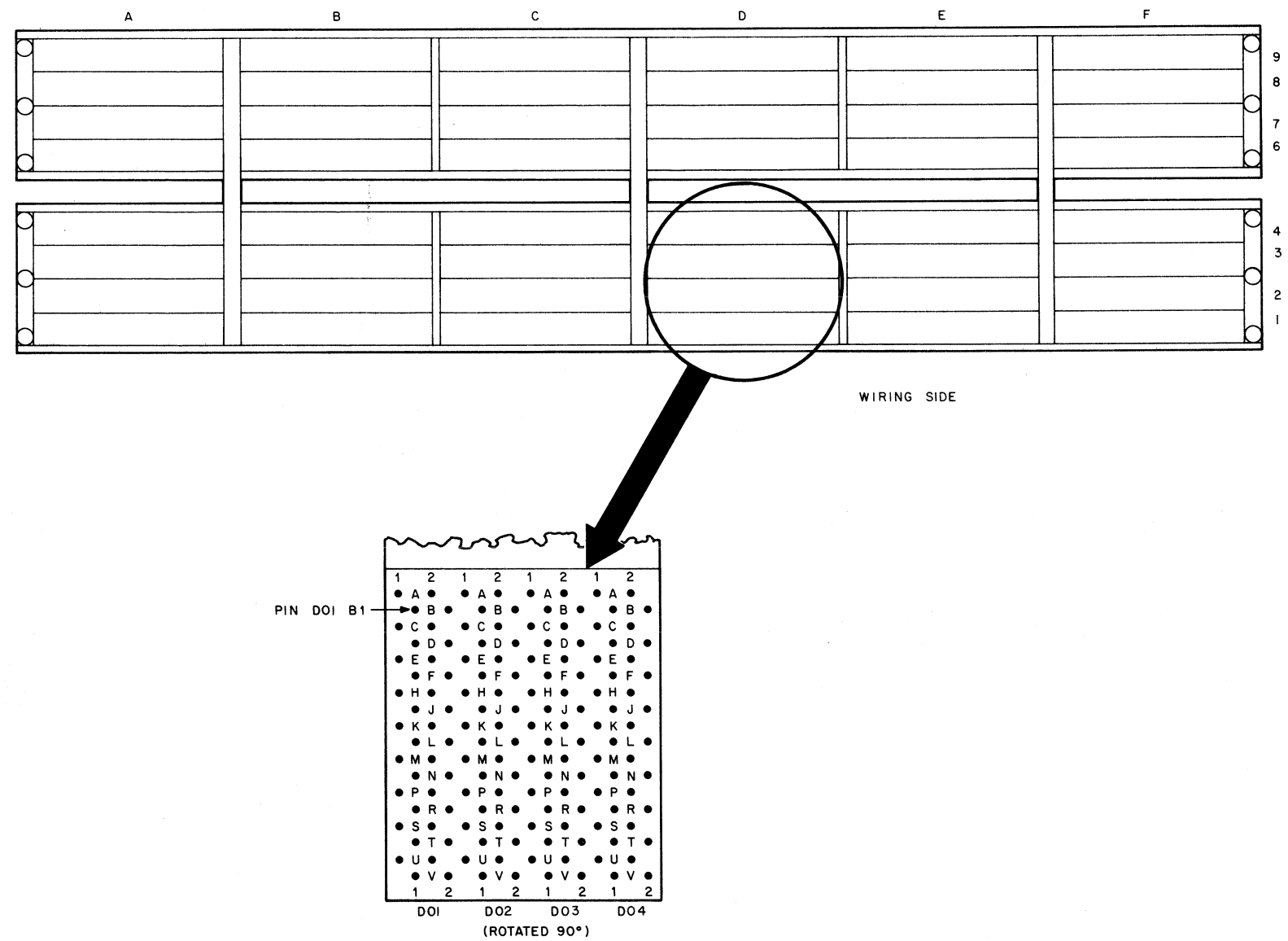
Figure 5-1 Module and Pin Designations
