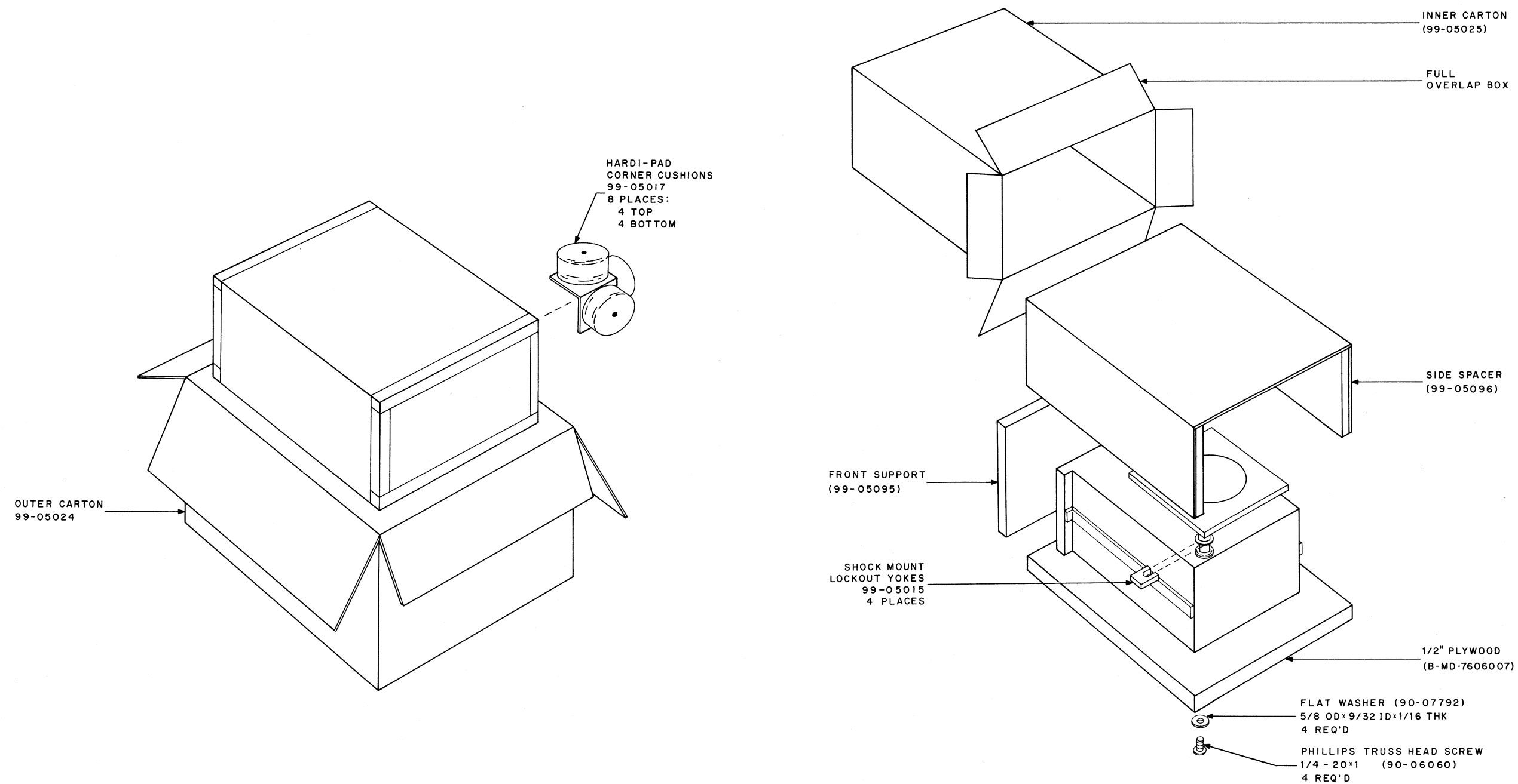
Figure 2-1 RS64 Disk File Packaging
