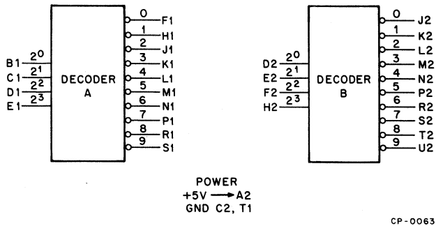
Figure 3-14 M163 Decoder Simplified Diagram
