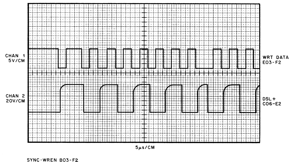
Figure 5-7 WRT Data and DSL Relationships
