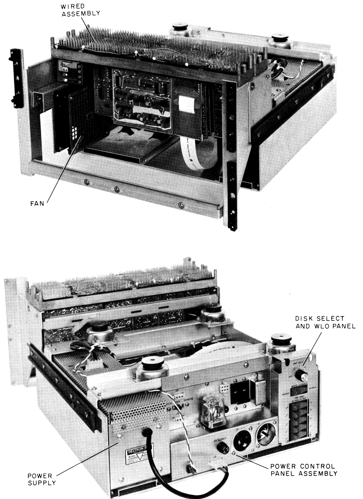
Figure 1-3 Power and Control Logic Assembly*
