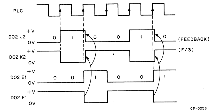
Figure 3-6 Counter Timing Relationships
