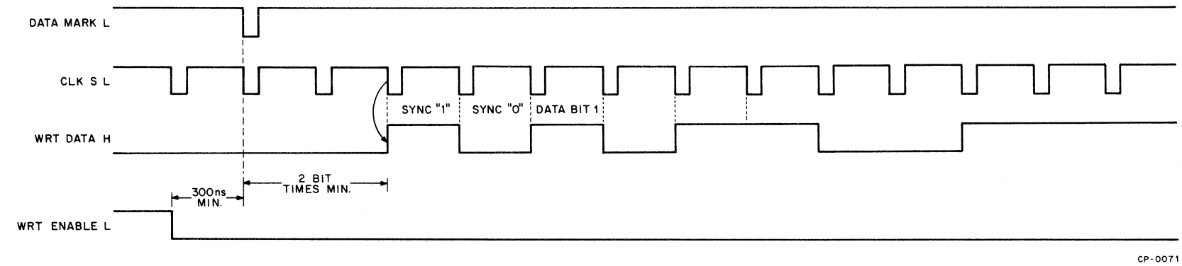
Figure 4-5 Write Synchronization
