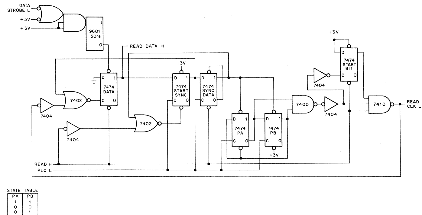
Figure 4-6 Read Synchronizing Interface Logic
