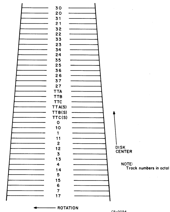
Figure 3-4 Track Arrangement
