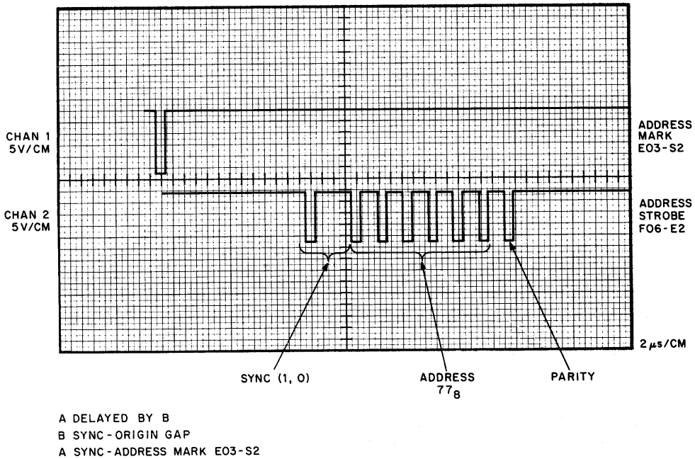
Figure 5-4 Address Mark and Address Strobe
