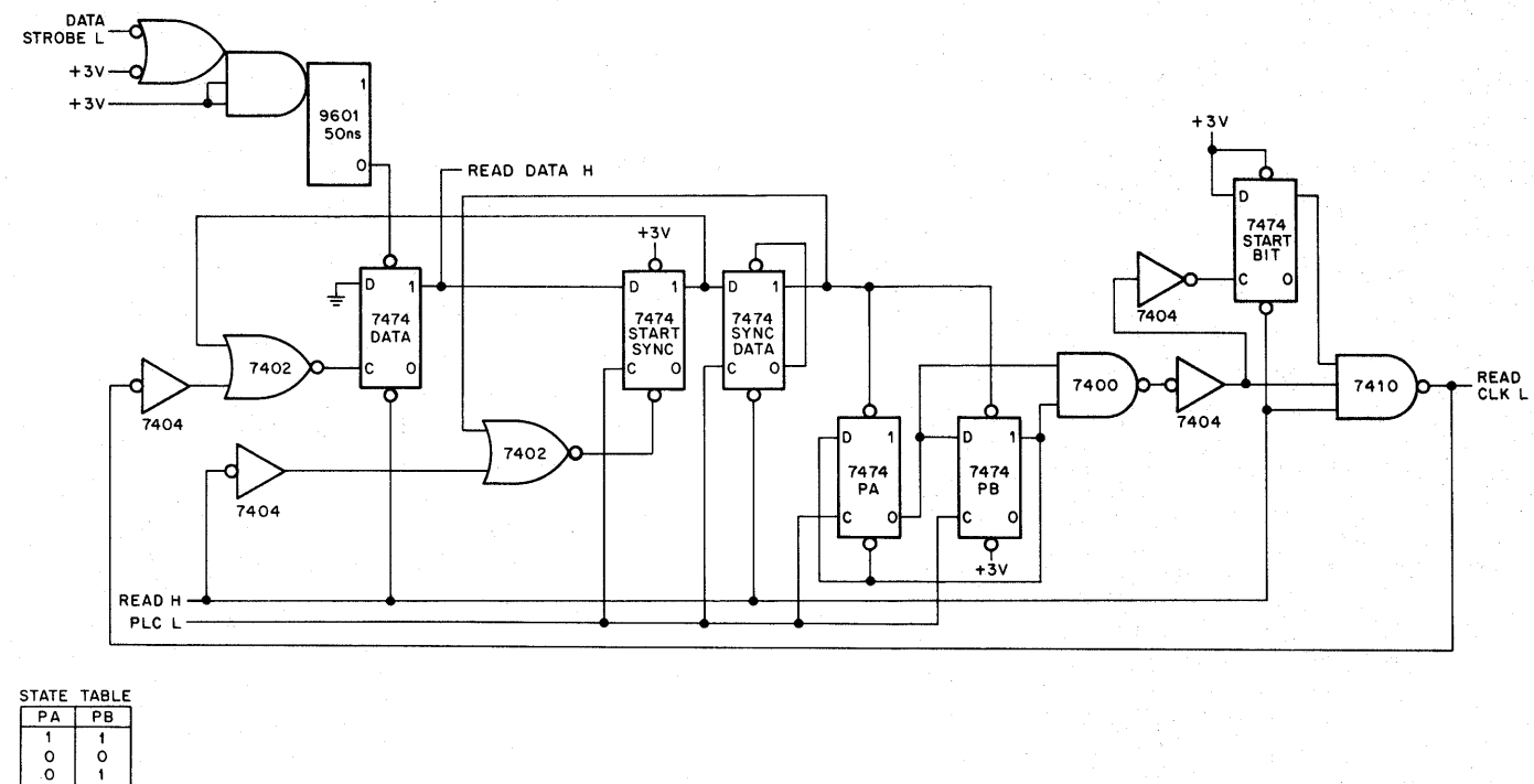
Figure 4-6 Read Synchronizing Interface Logic
