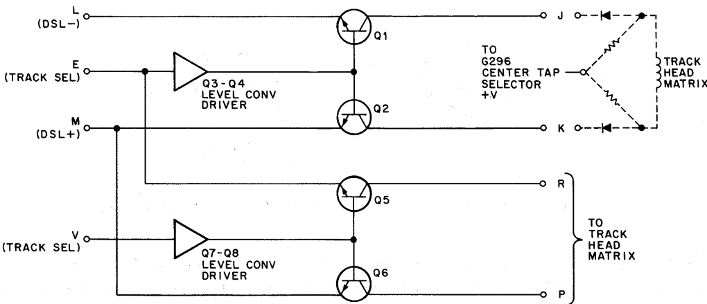
Figure 3-12 G295 Series Switch Simplified Diagram
