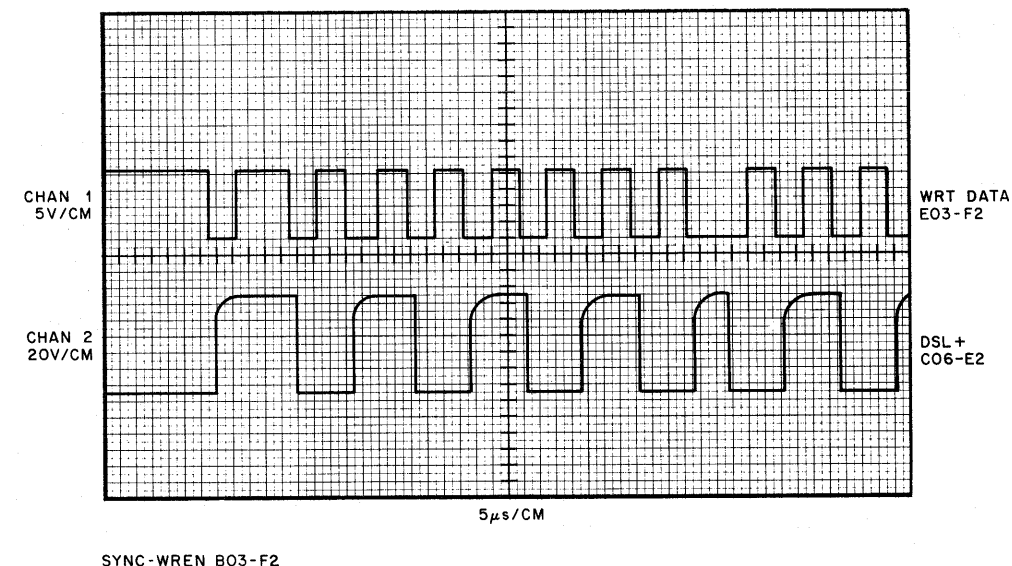
Figure 5-7 WRT Data and DSL Relationships
