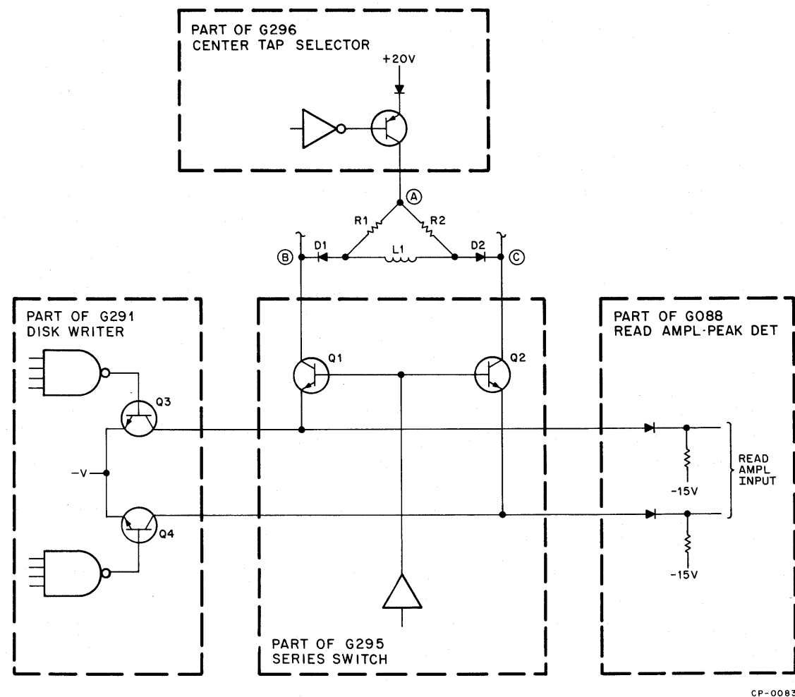
Figure 3-7 Read/Write Electronics
