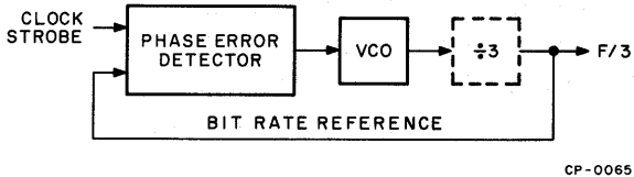
Figure 3-16 M4201 Phase-Locked Clock Simplified Diagram
