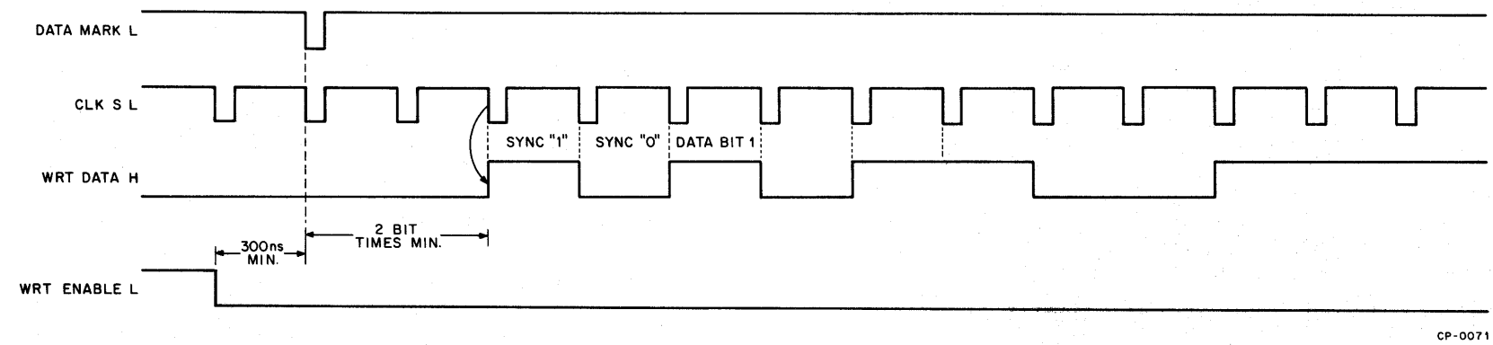
Figure 4-5 Write Synchronization
