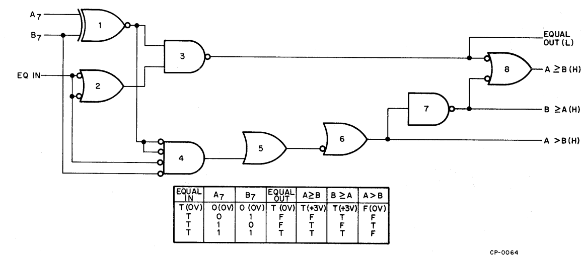
Figure 3-15 M167 Comparator Simplified Diagram
